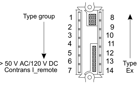
Functional diagram for coding (suggestion) Partial view of socket
