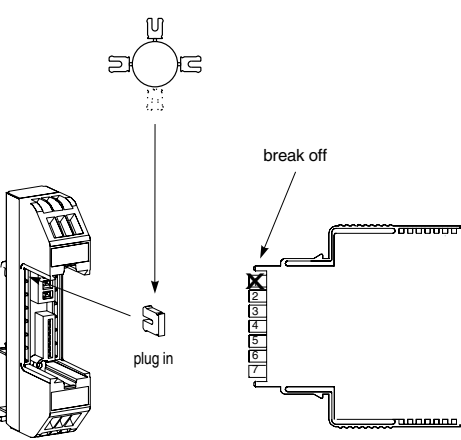
Example of coding (type V17131-1x) Encoding star with 4 encoding pins (part of supply for socket/backplane)
