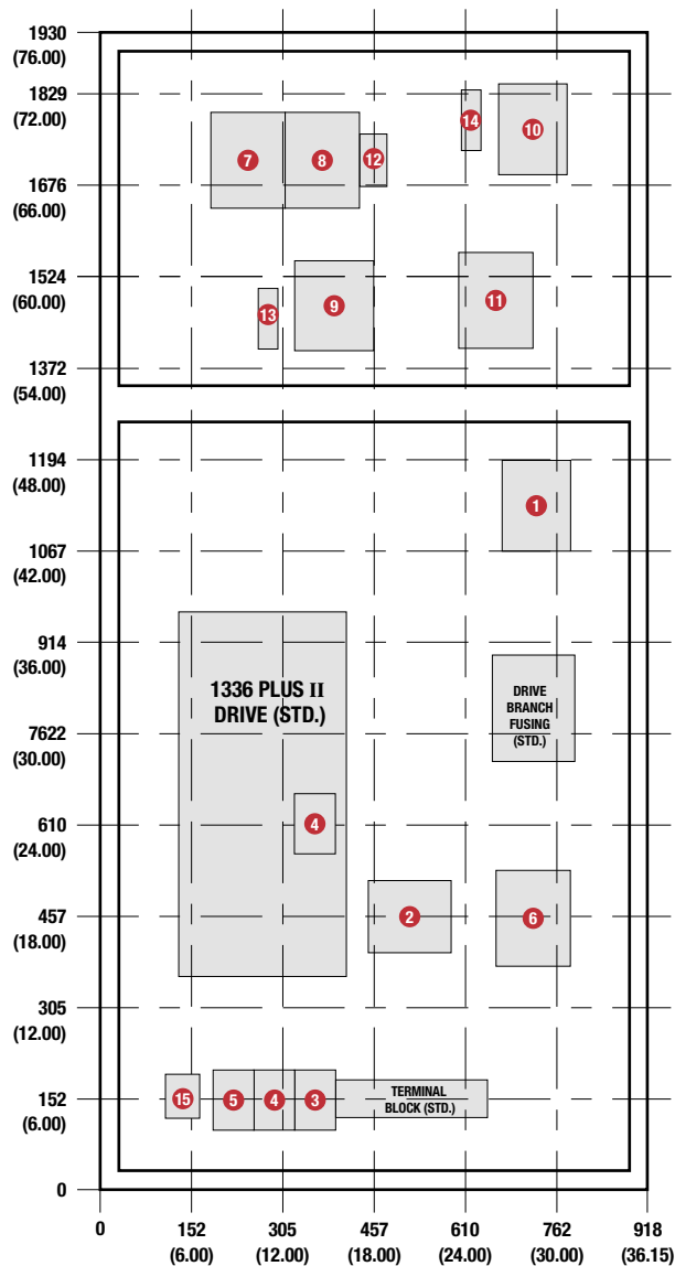
WITH OPTION BAY
