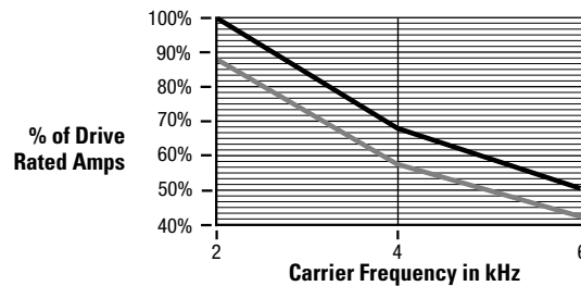
Figure AA 1336F-CP400, CPR450
