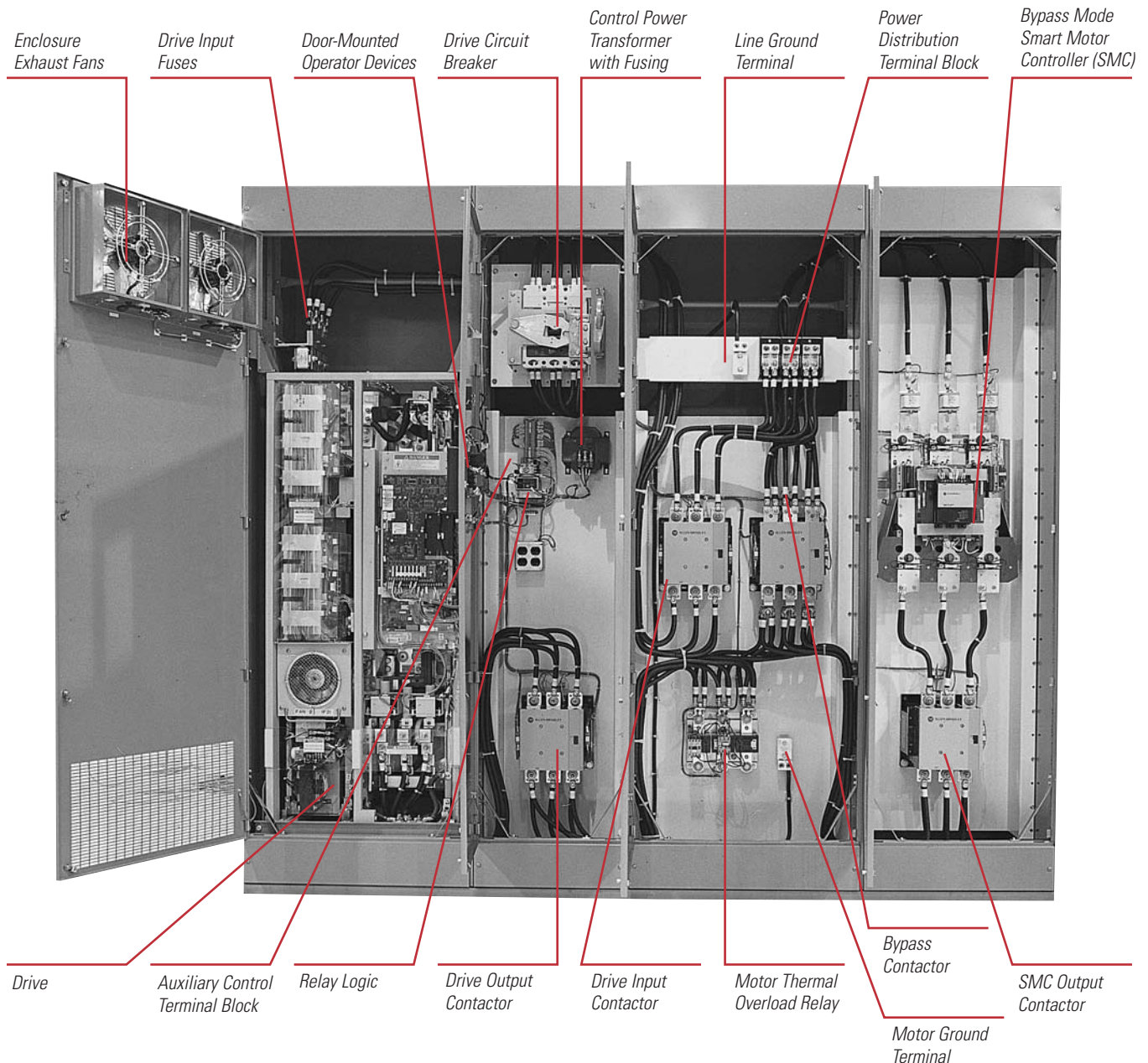
500 HP 6 Pulse 460V AC NEMA Type 1 Floor Mounted Packaged Drive with SMC Style Bypass
