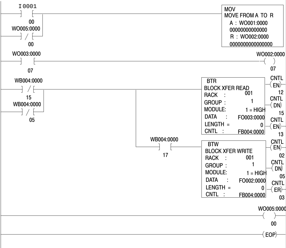
Figure 6.3 Test Program (PLC-3)
