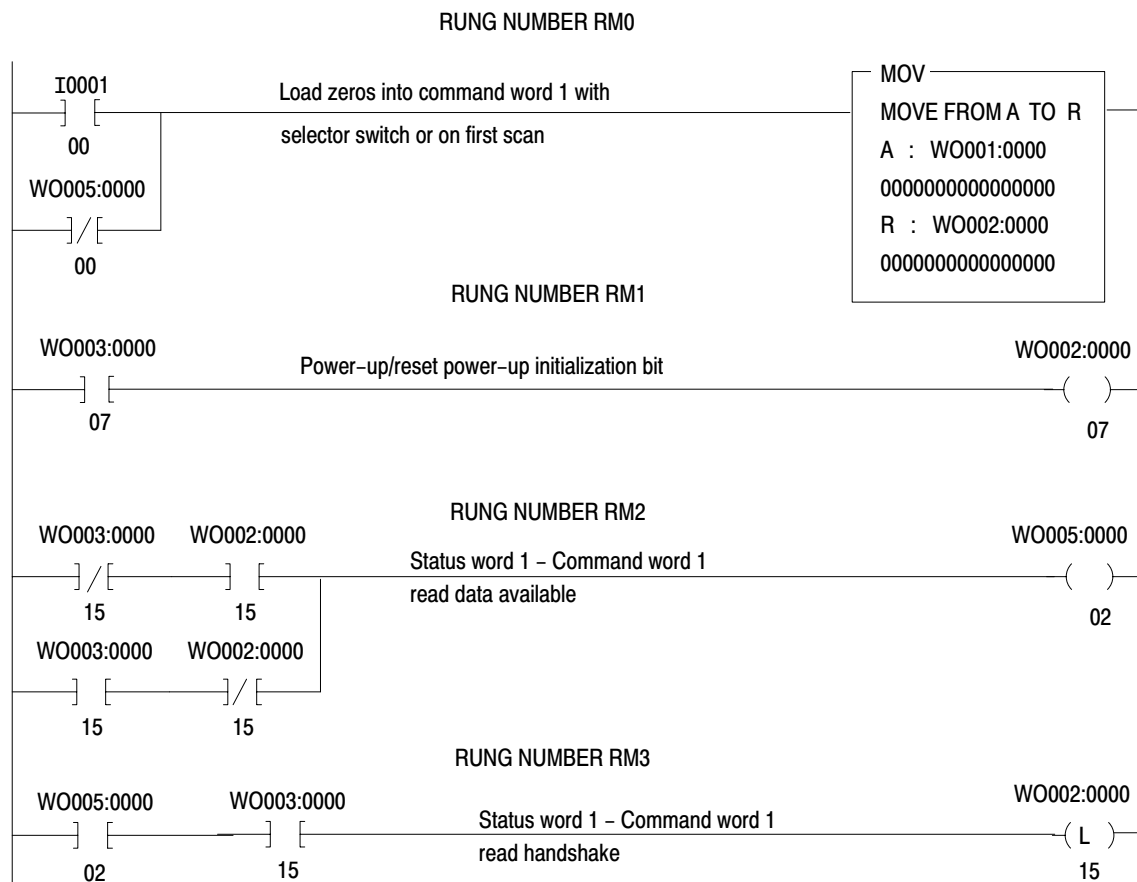
Figure B.11 Example Read/Write Program
