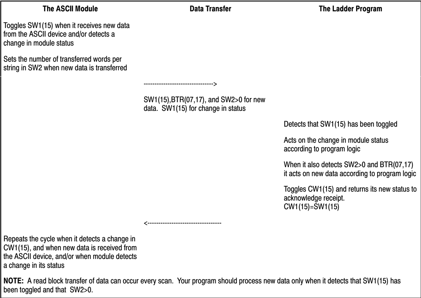
Figure 4.1 Read Handshaking
