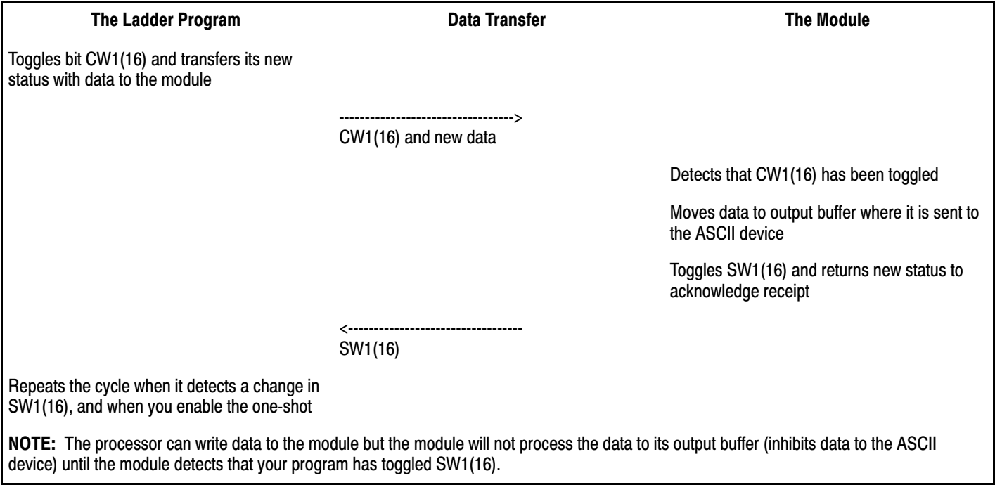
Figure 4.2 Write Handshaking
