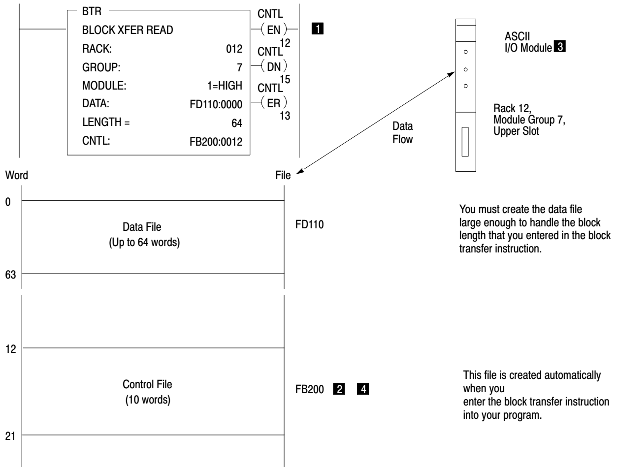
Figure B.2 Example Block Transfer Operation
