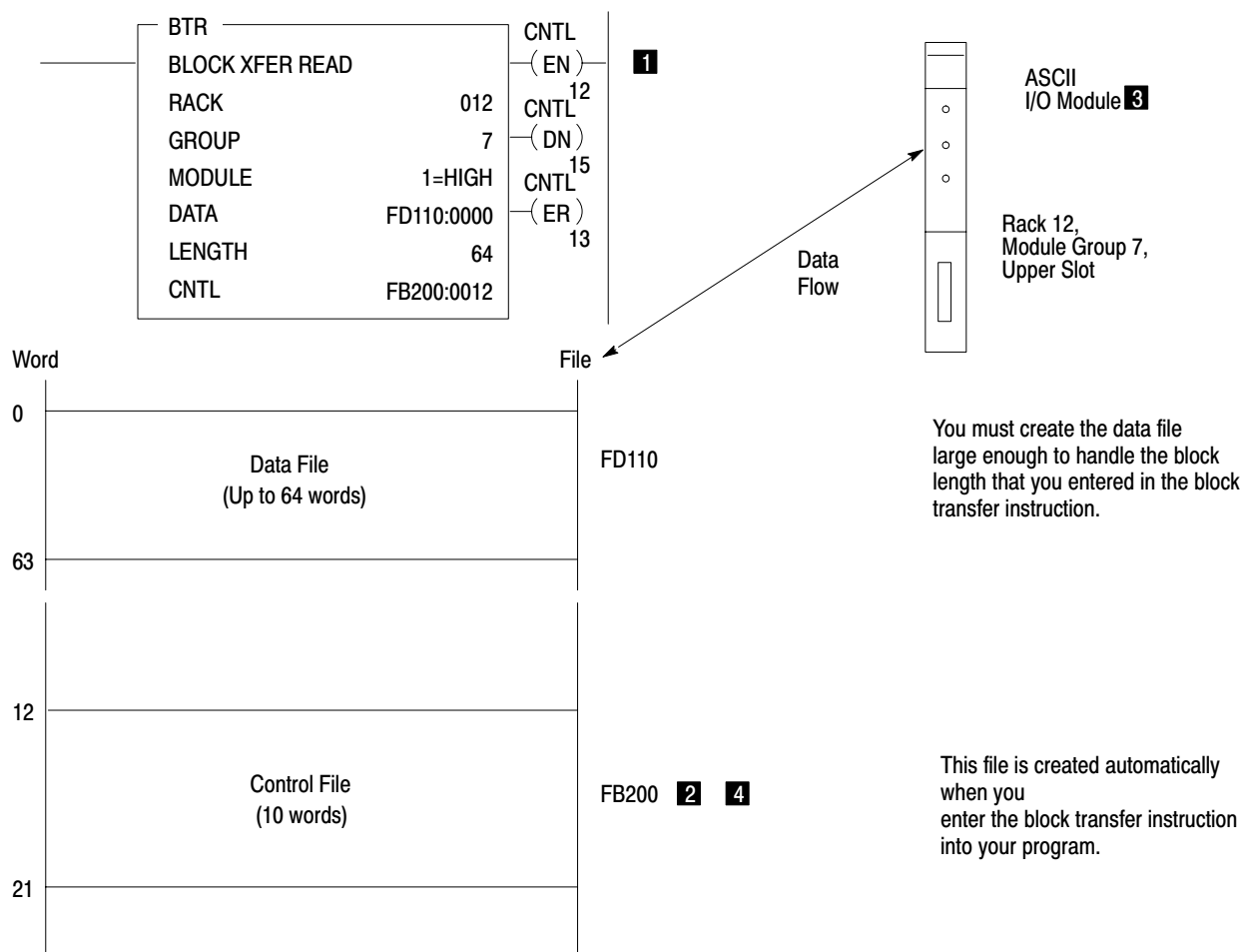
Figure A.11 Example Block Transfer Operation
