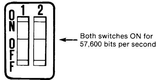
Switch assembly SW-5
