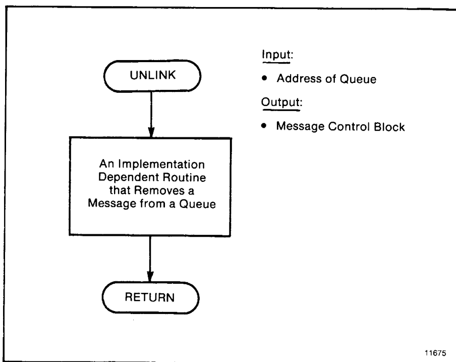
Figure B.22 — UNLINK Subroutine
