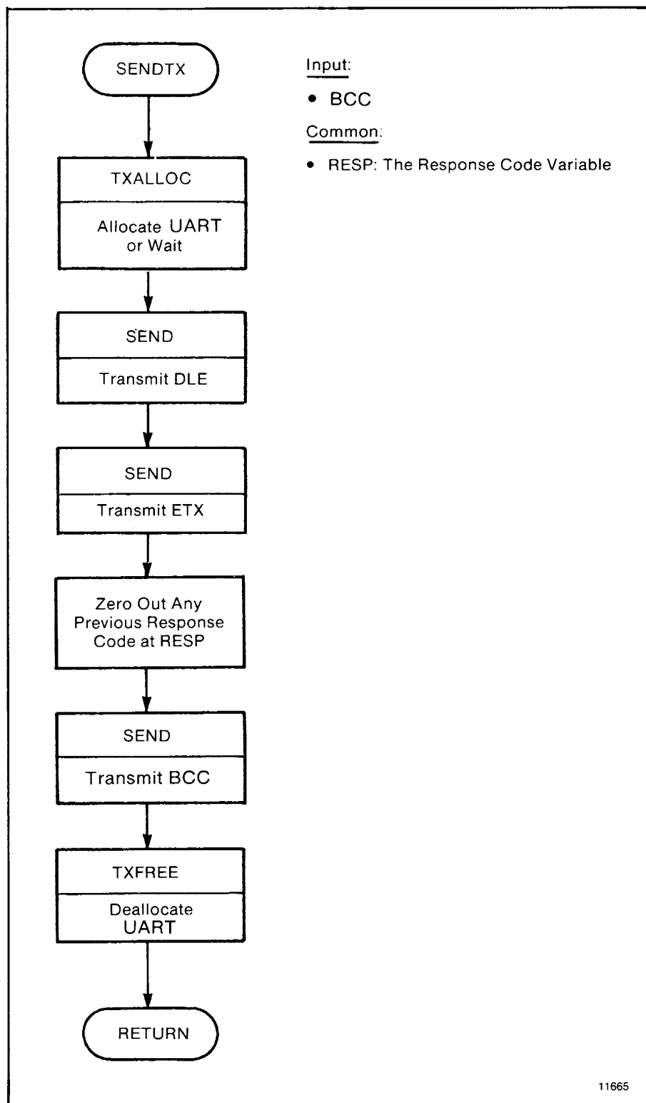
Figure B.12 — SENDTX Subroutine
