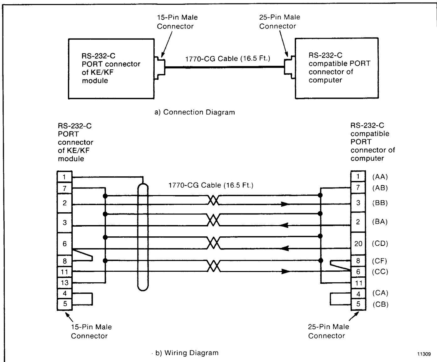
Figure 3.9 — Connection to a Computer
