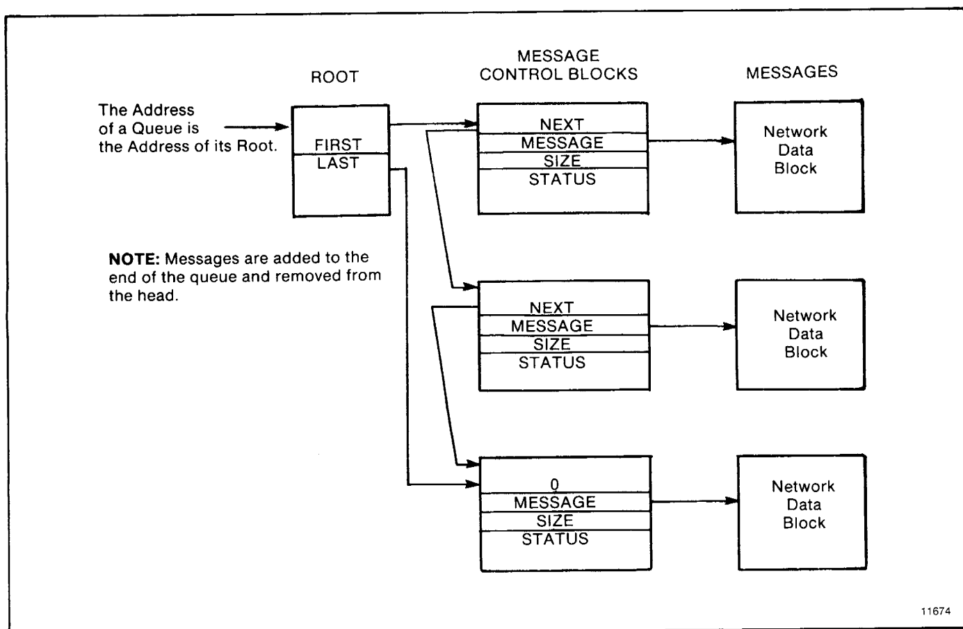
Figure B.21 — Message Queue
