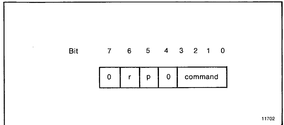
Figure 5.4 — CMD Byte Format
