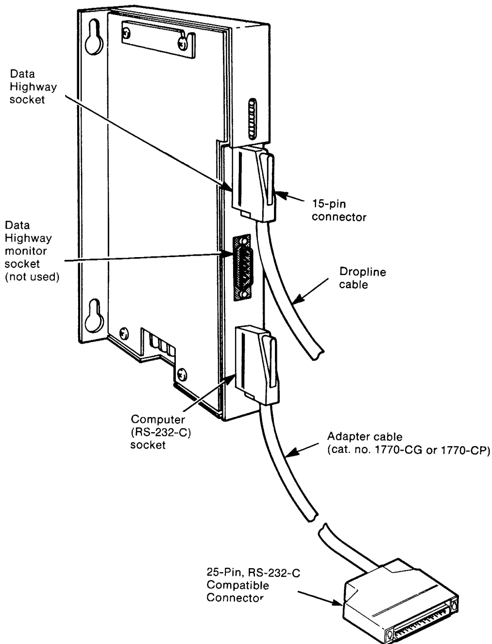
Figure 3.8 — KE/KF Module Connectors
