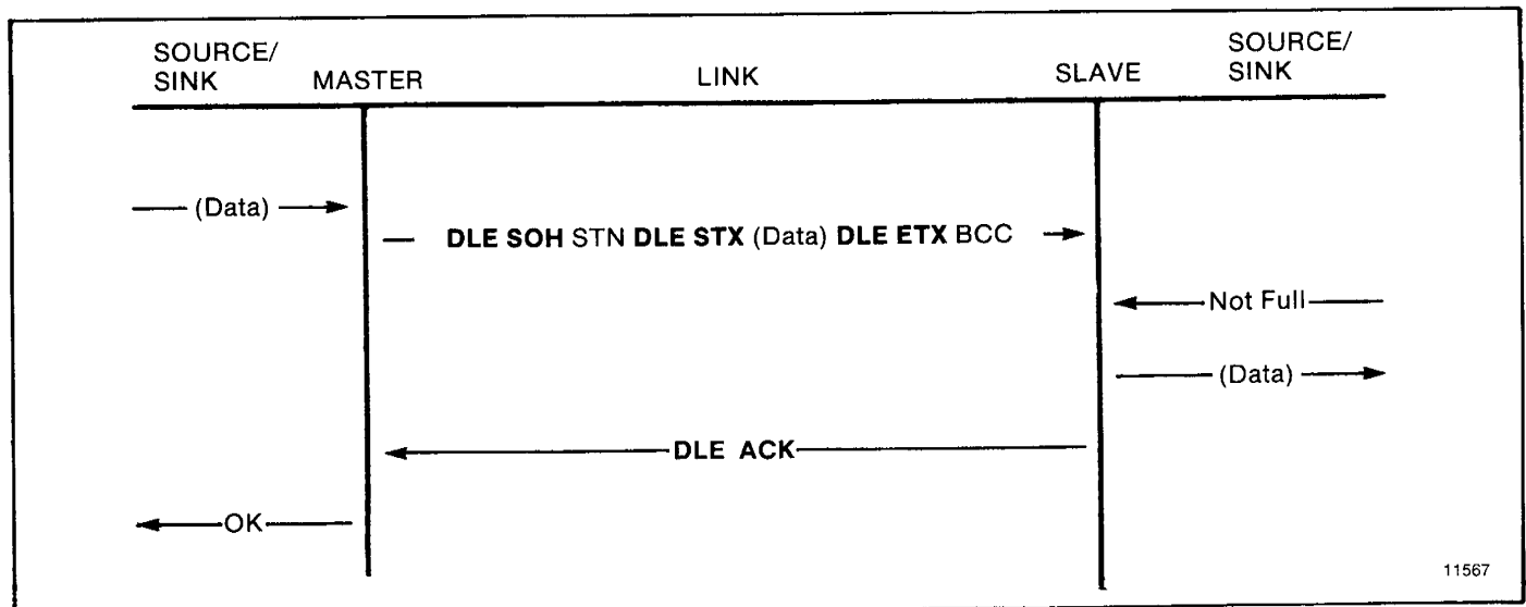
Figure 4.17 — Normal Message Transfer
