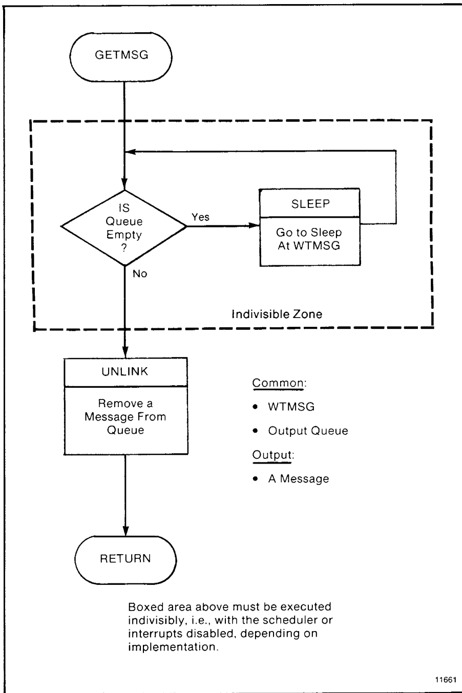
Figure B.8 — GETMSG Subroutine
