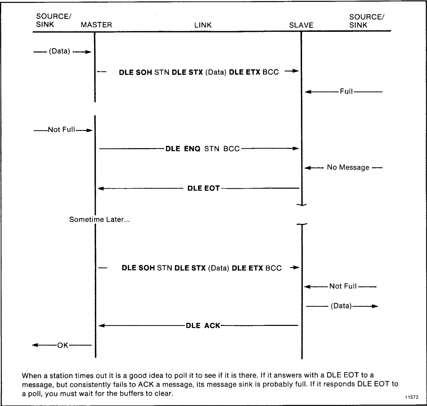
Figure 4.23 — Message Sink Full, Case 1
