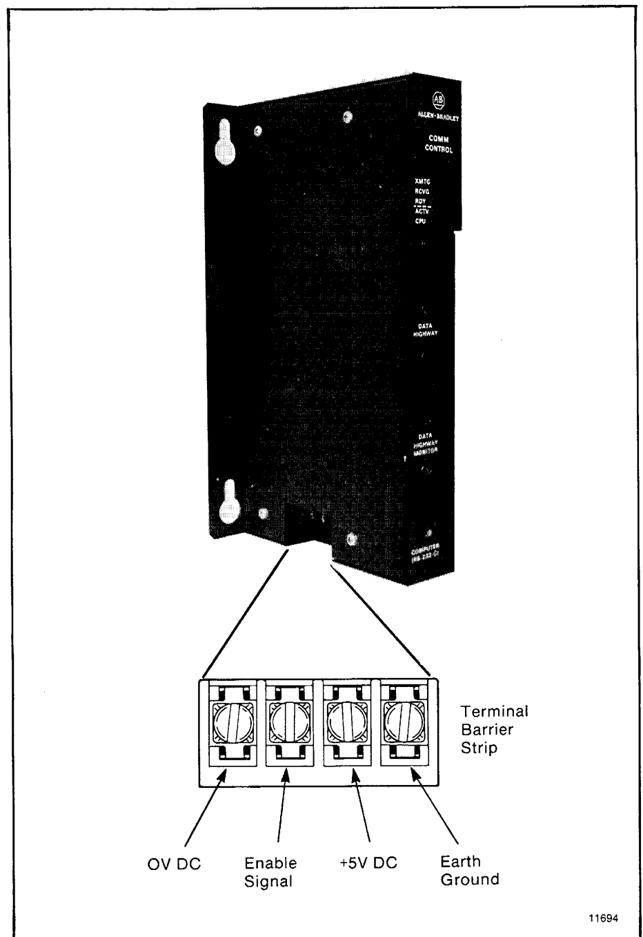
Figure 3.6 — Power Supply Connections for 1771-KF Module
