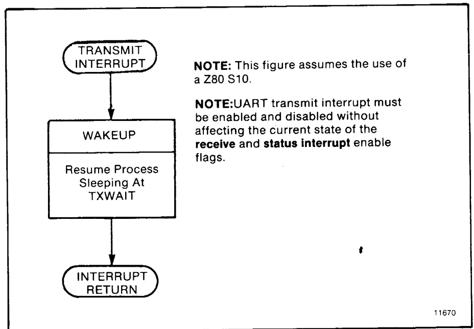
Figure B.17 — TRANSMIT INTERRUPT Subroutine
