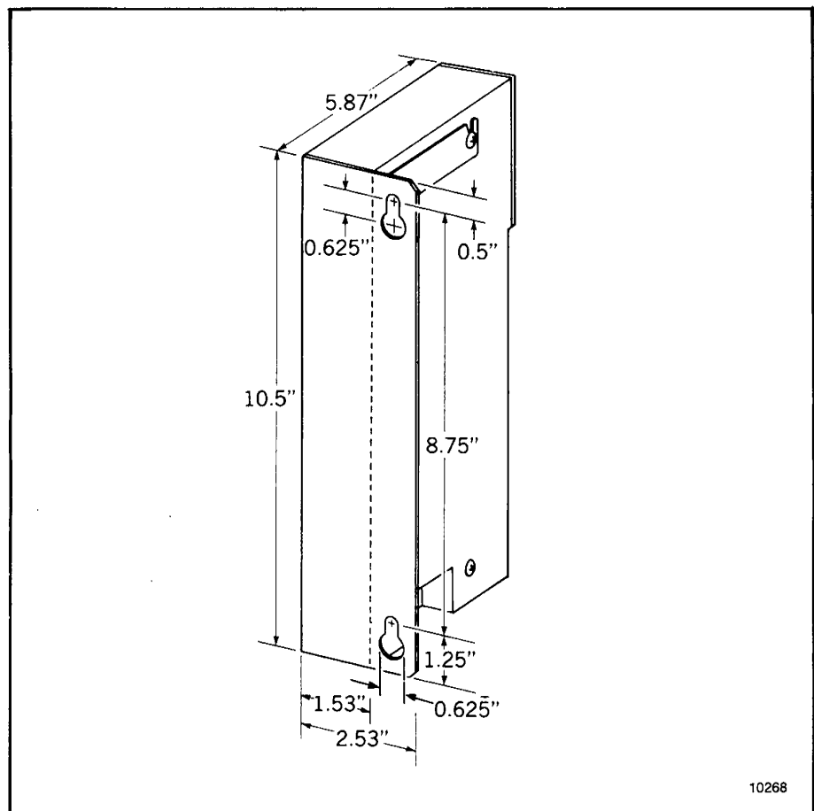
Figure 3.5 — Mounting Dimensions for 1771-KF Module
