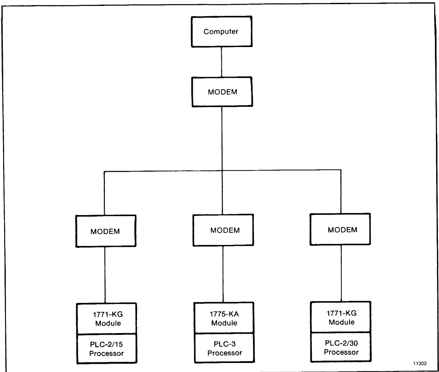
Figure 2.4 — Stand-Alone Multidrop Link to a Computer
