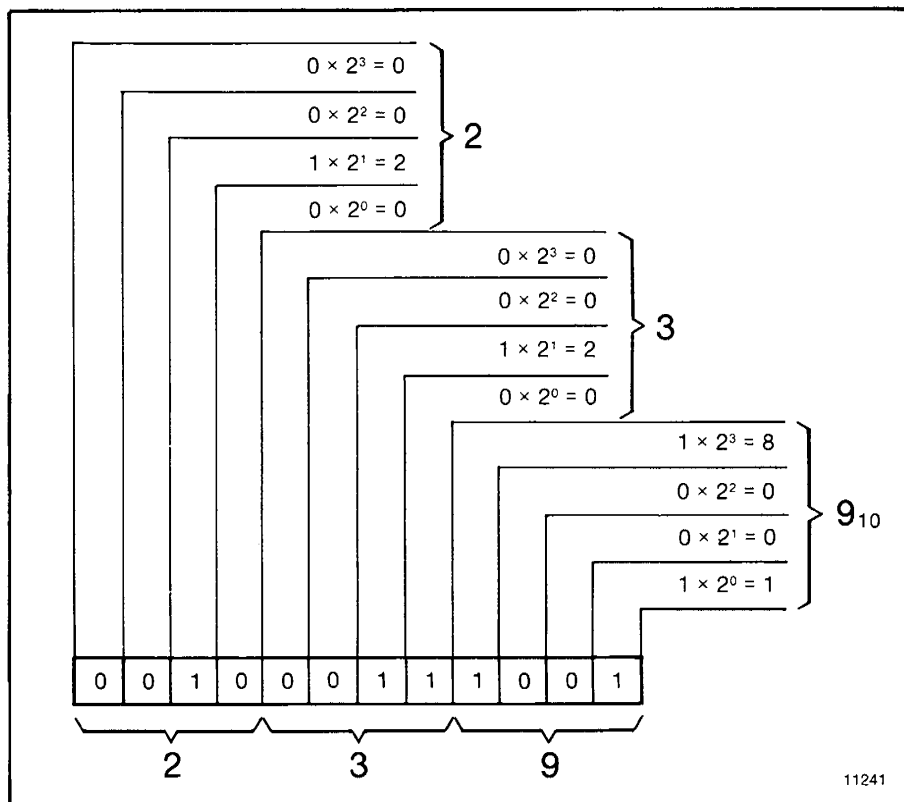
Figure 6.2 — BCD Representation of Decimal 239
