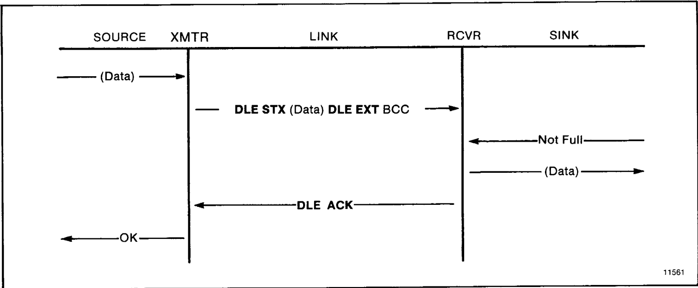
Figure 4.9 — Normal Message Transfer
