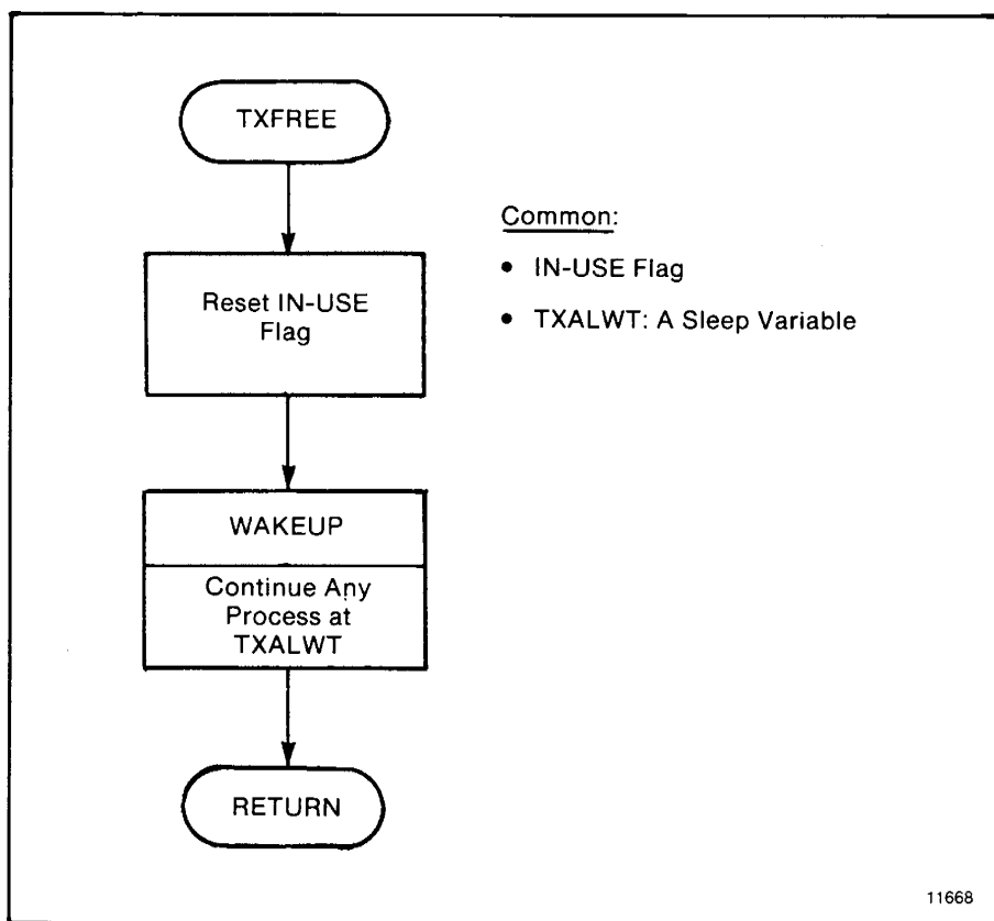
Figure B.16 — TXFREE Subroutine
