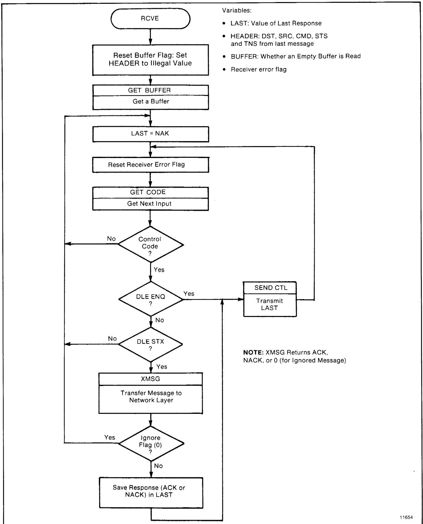
Figure B.24 — Receiver Routine for Full-Duplex Protocol
