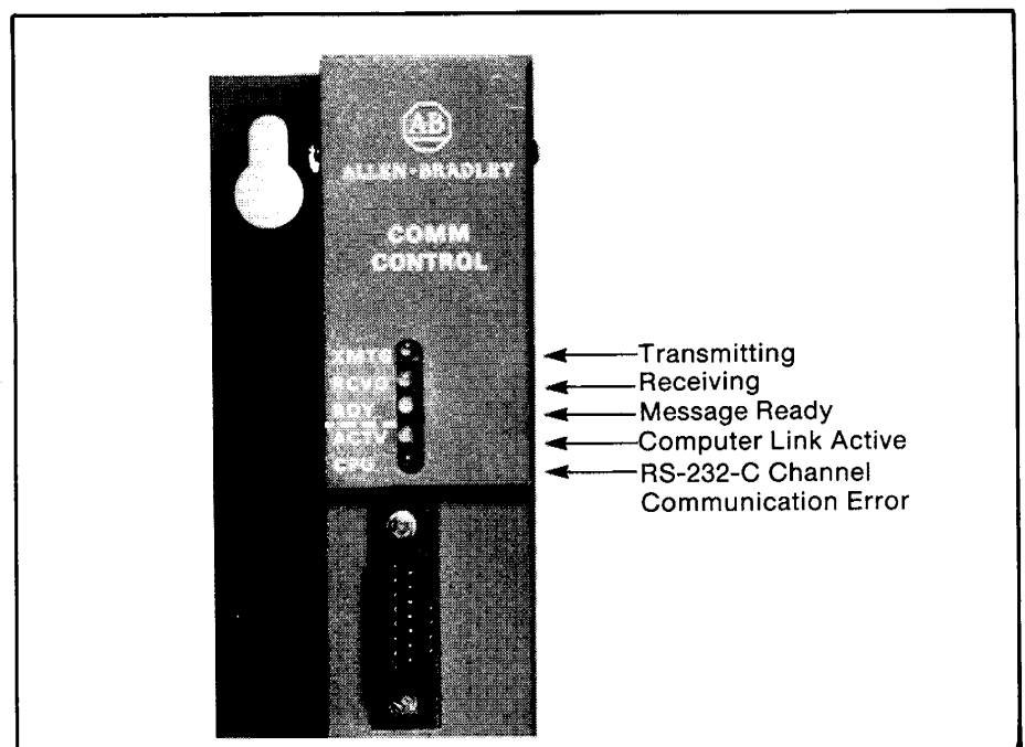
Figure 3.13 — Diagnostic Indicators
