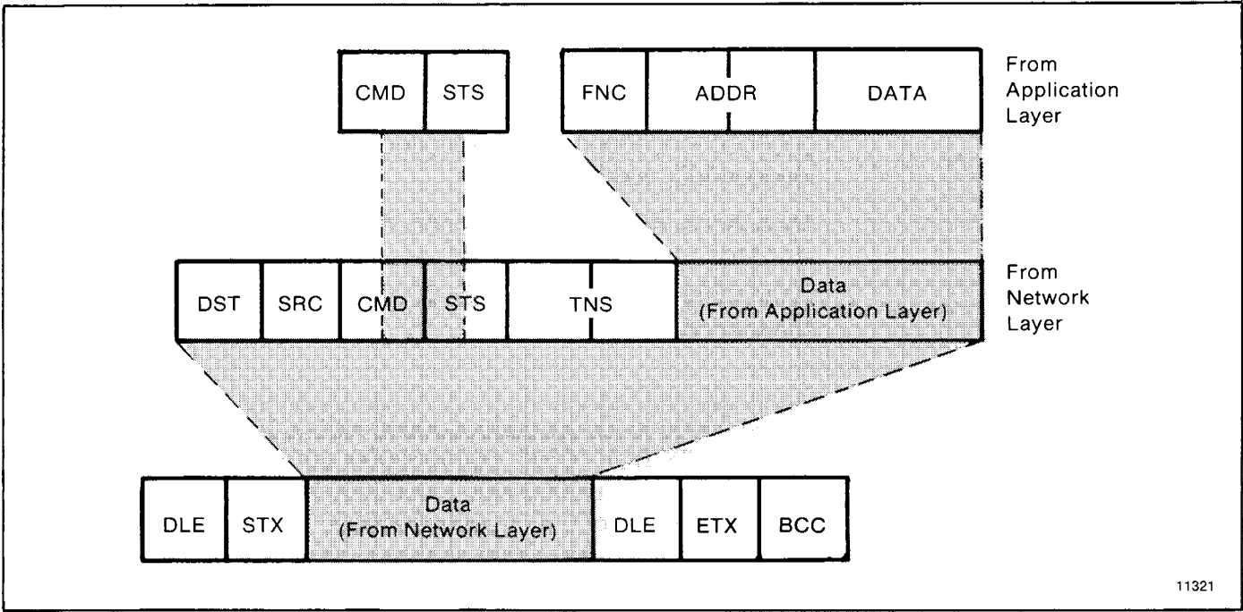
Figure 4.1 — Link Packet Format for Full-Duplex Protocol
