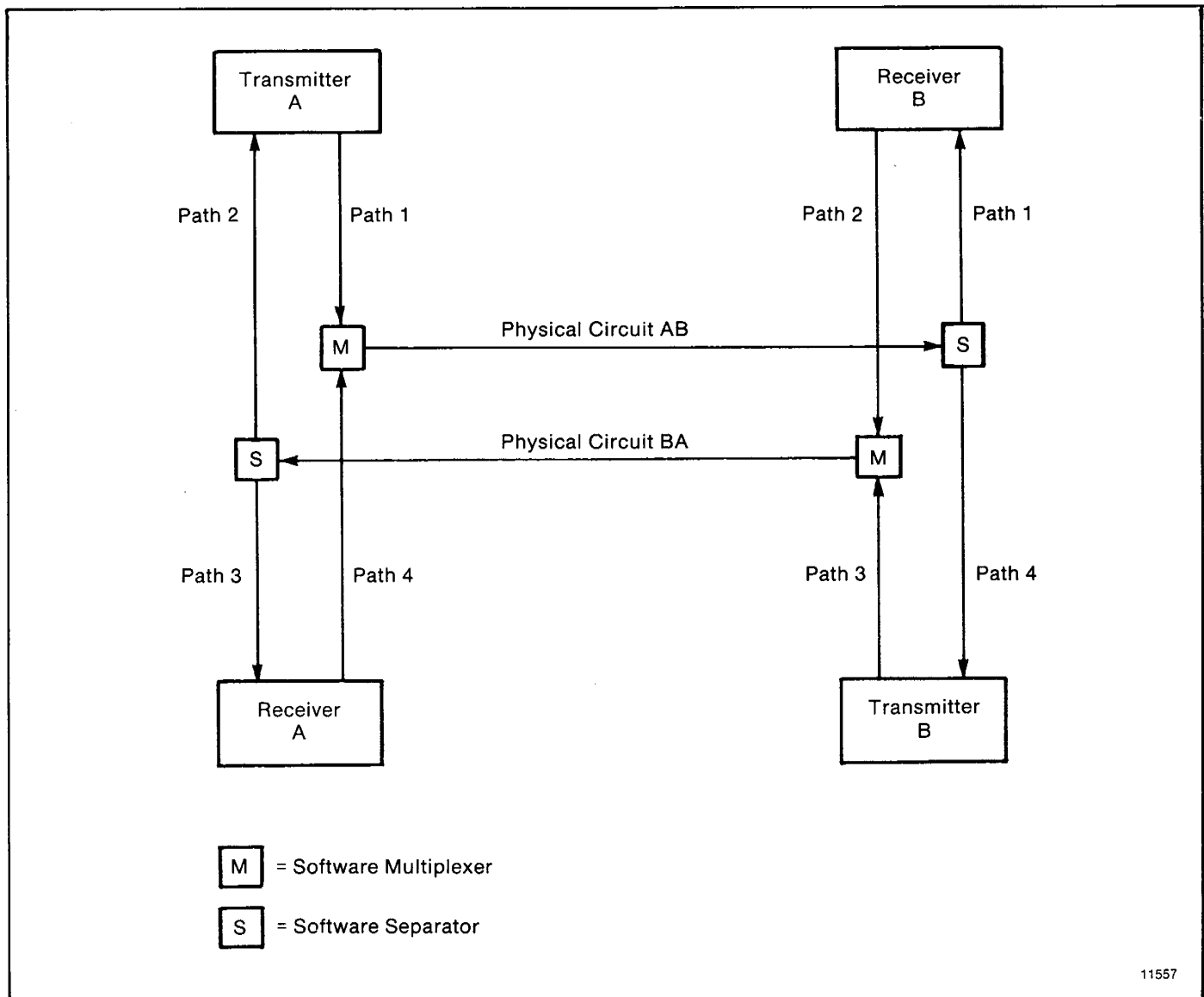
Figure 4.3 — Software Implementation of Data Paths
