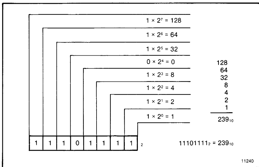
Figure 6.1 — Binary Numbers
