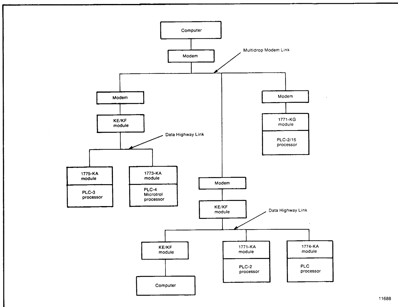
Figure 1.3 — Multidrop Link
