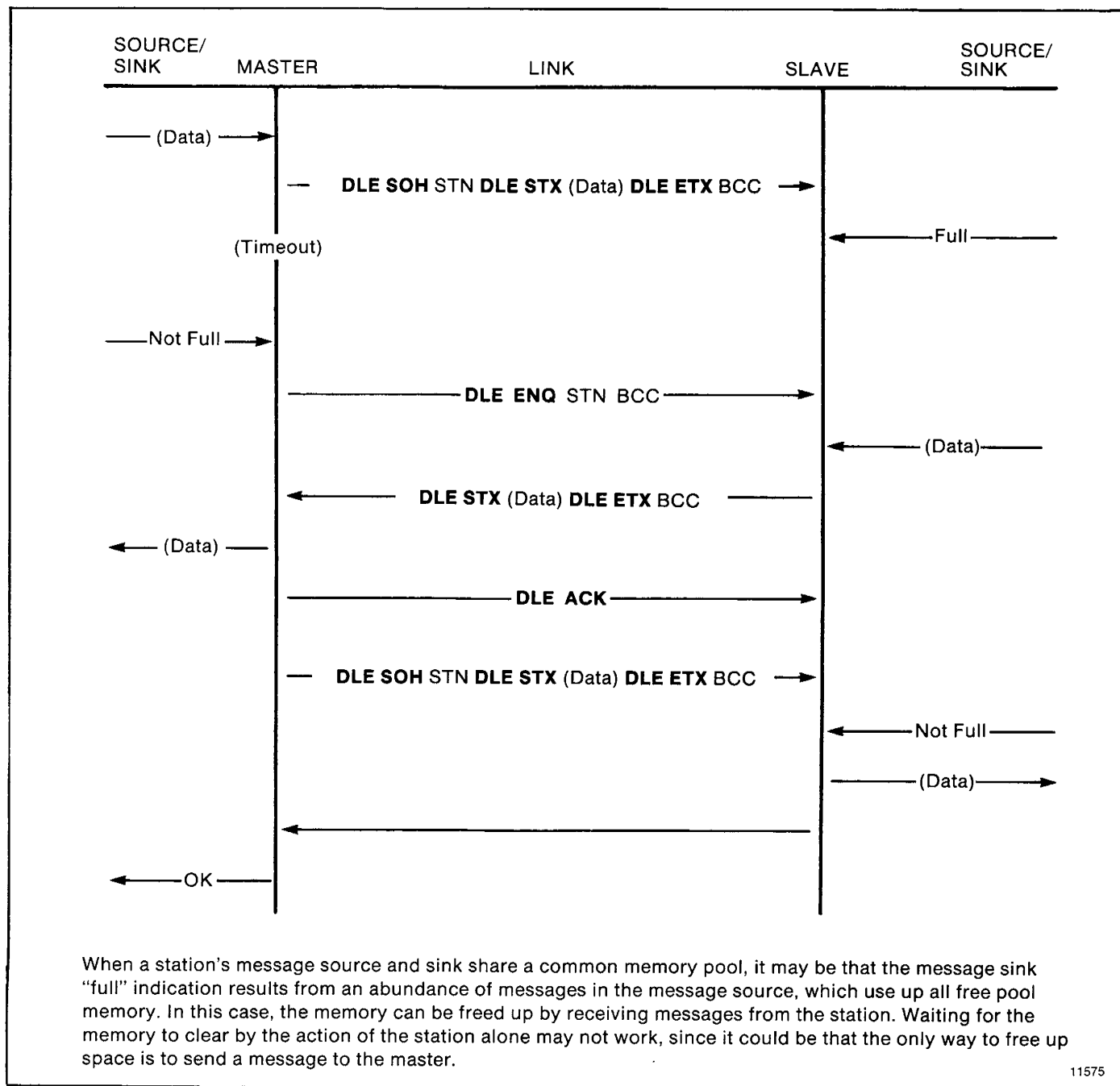
Figure 4.24 — Message Sink Full, Case 2
