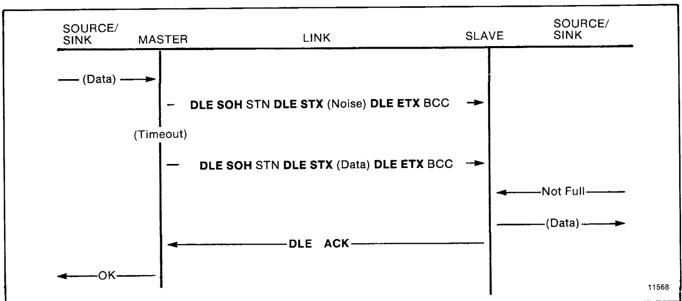
Figure 4.18 — Message Transfer with Invalid BCC
