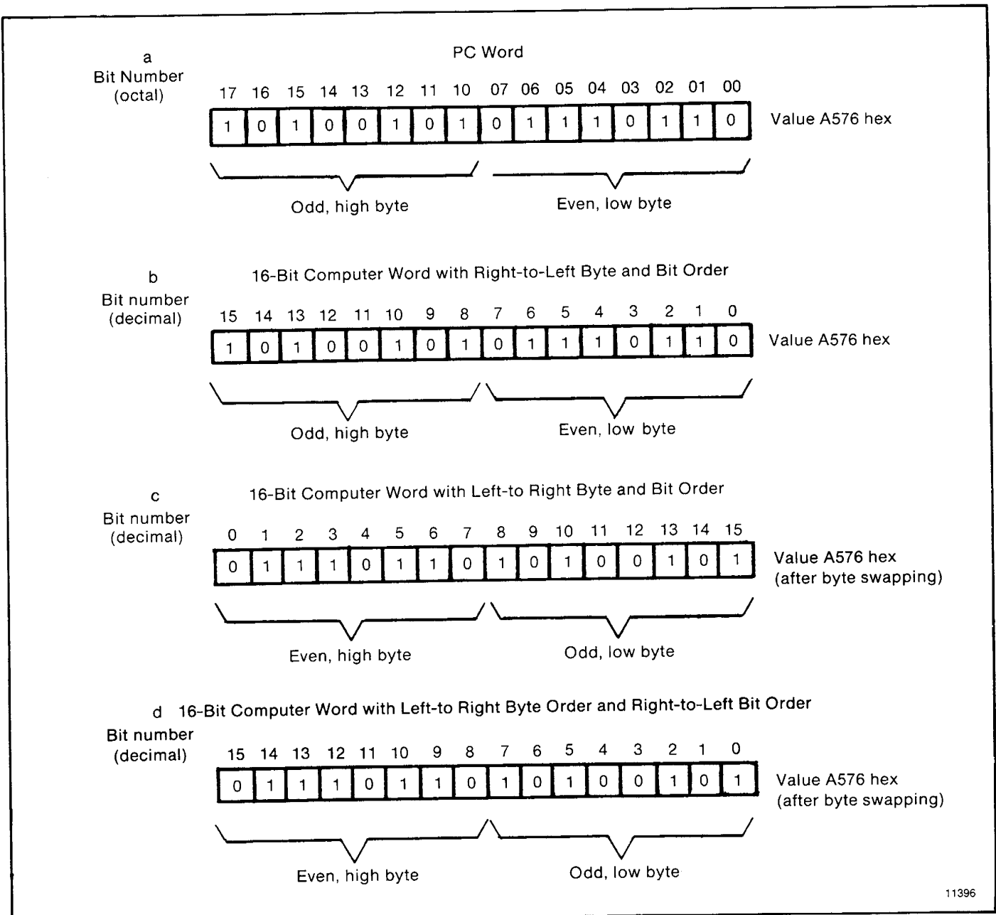
Figure 6.6 a, b, c, & d — Results of Transmitting Low Byte First
