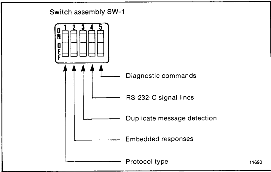
Figure 3.2 — RS-232-C Link Features
