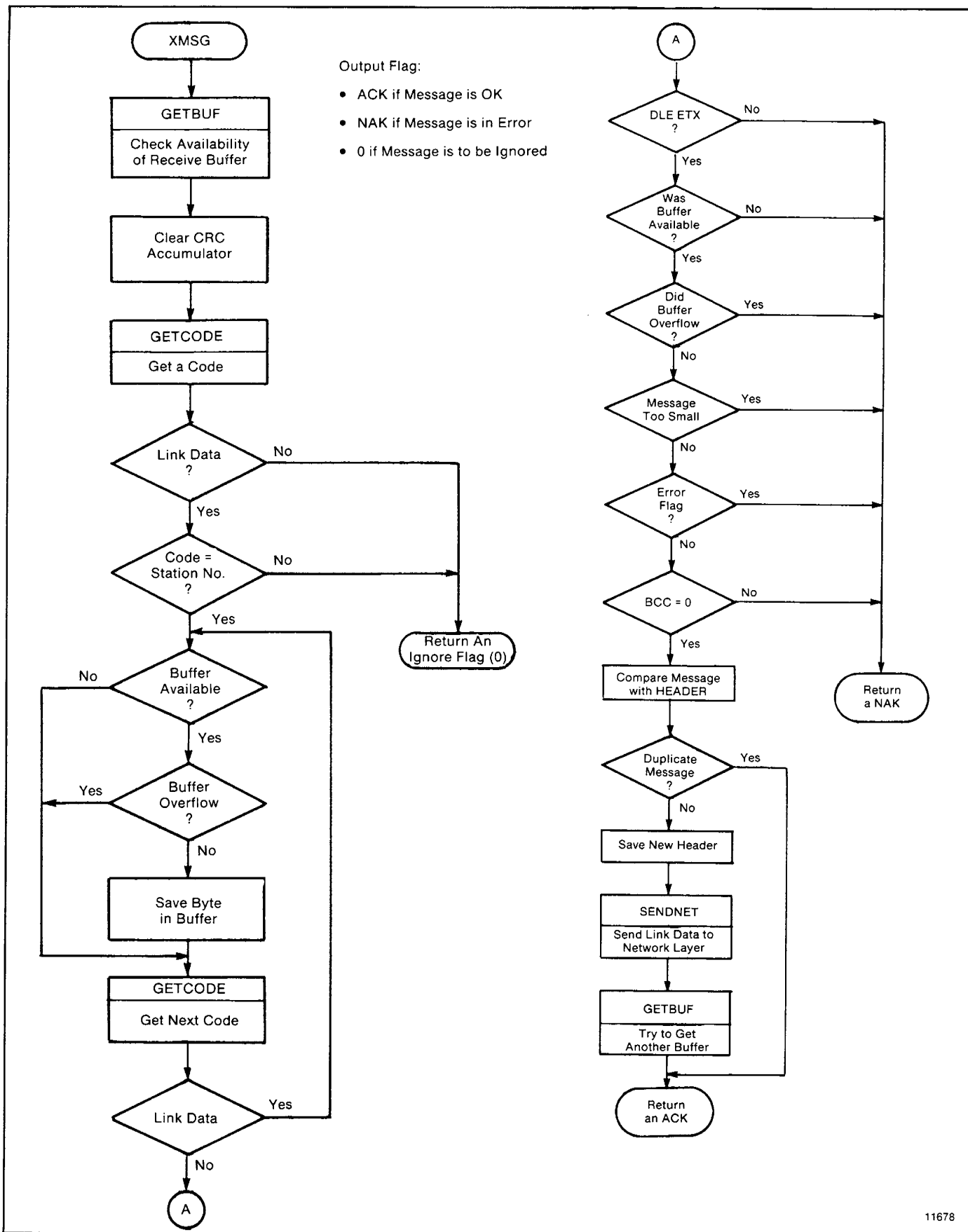
Figure B.25 — XMSG Subroutine
