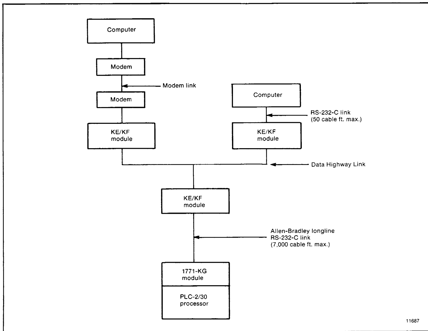
Figure 1.2 — Point-to-Point Links
