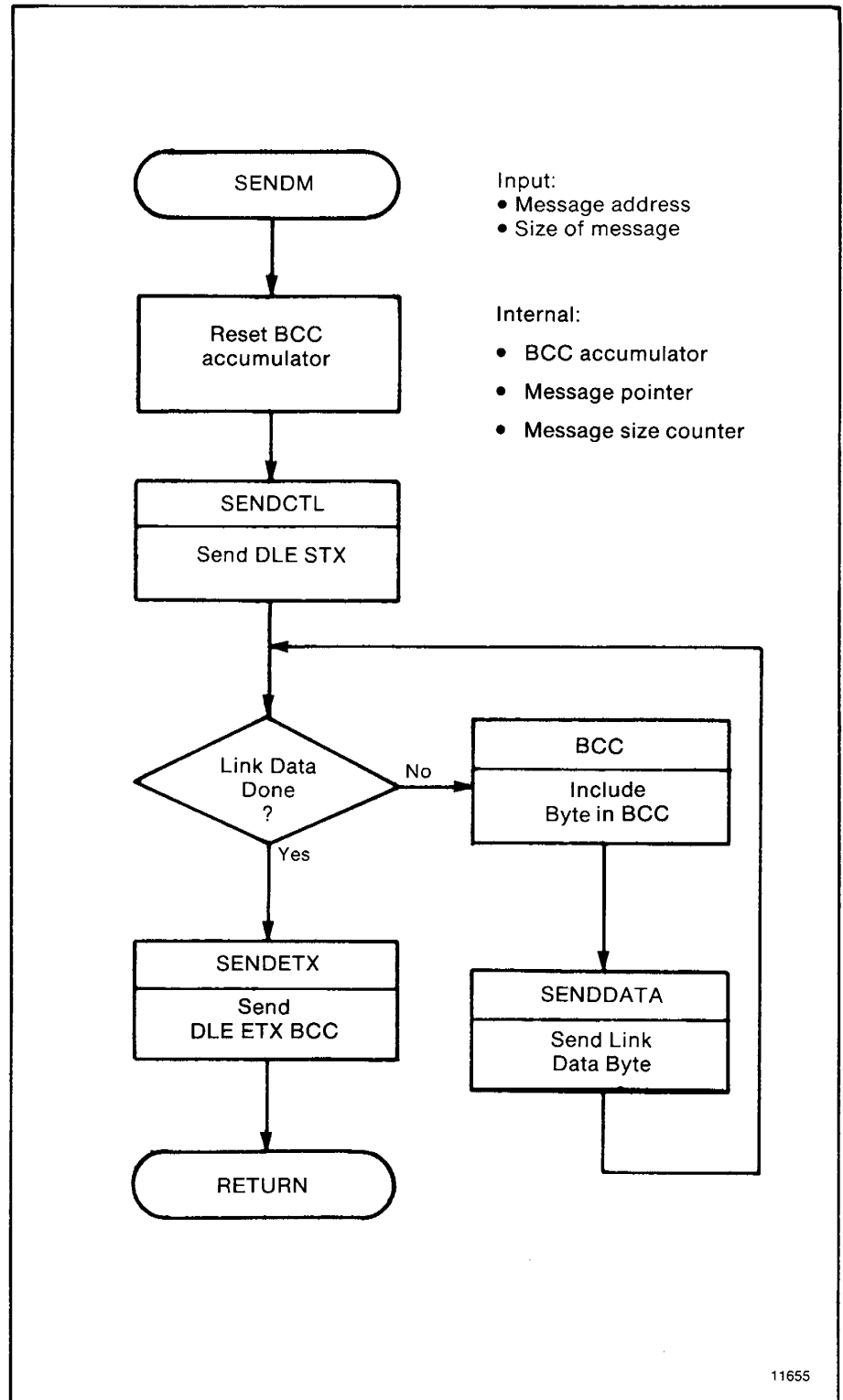
Figure B.4 — SENDM Subroutine
