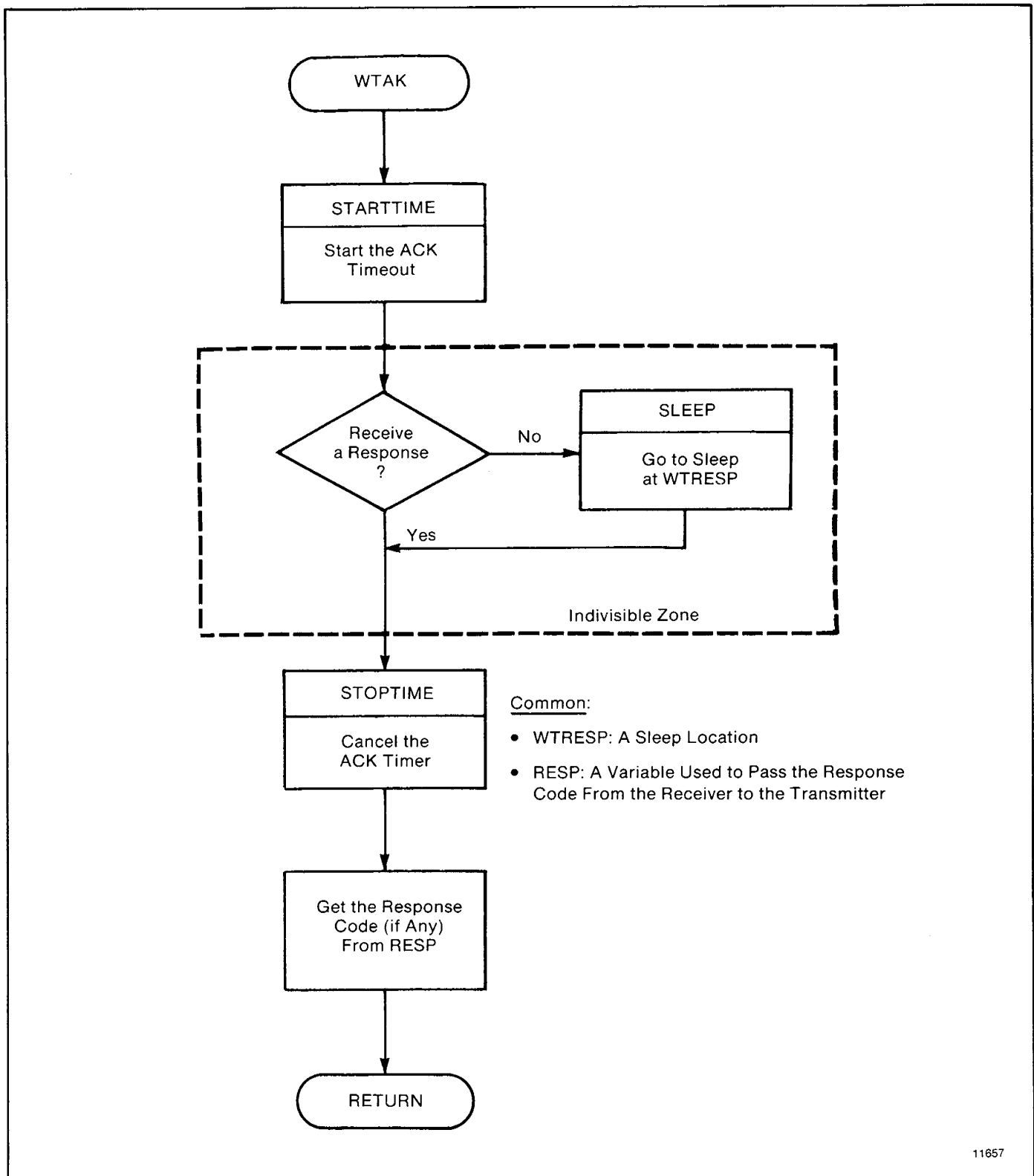
Figure B.3 — WTAK Subroutine
