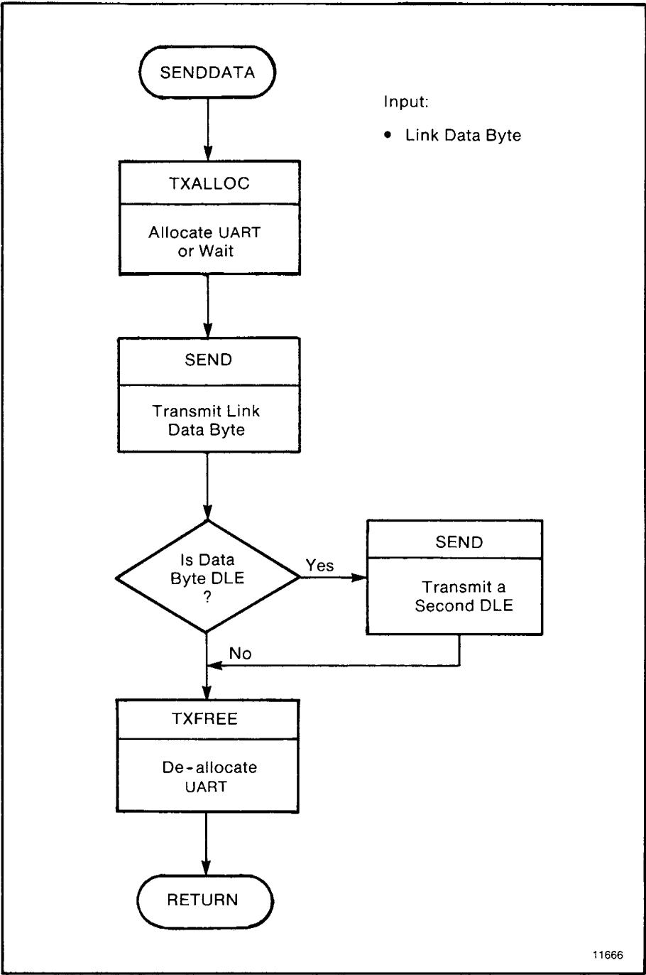
Figure B.14 — SENDDATA Subroutine
