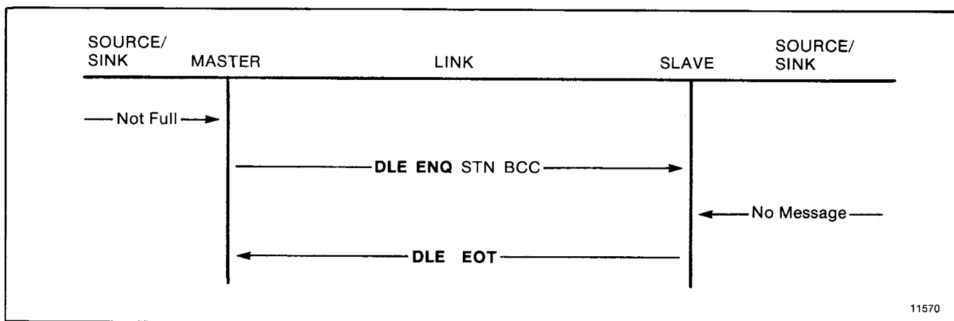
Figure 4.20 — Poll with No Message Available
