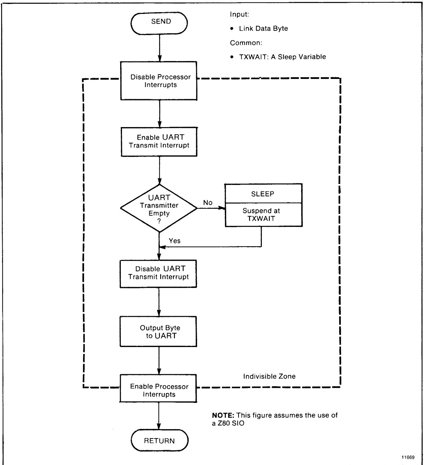
Figure B.13 — SEND Subroutine
