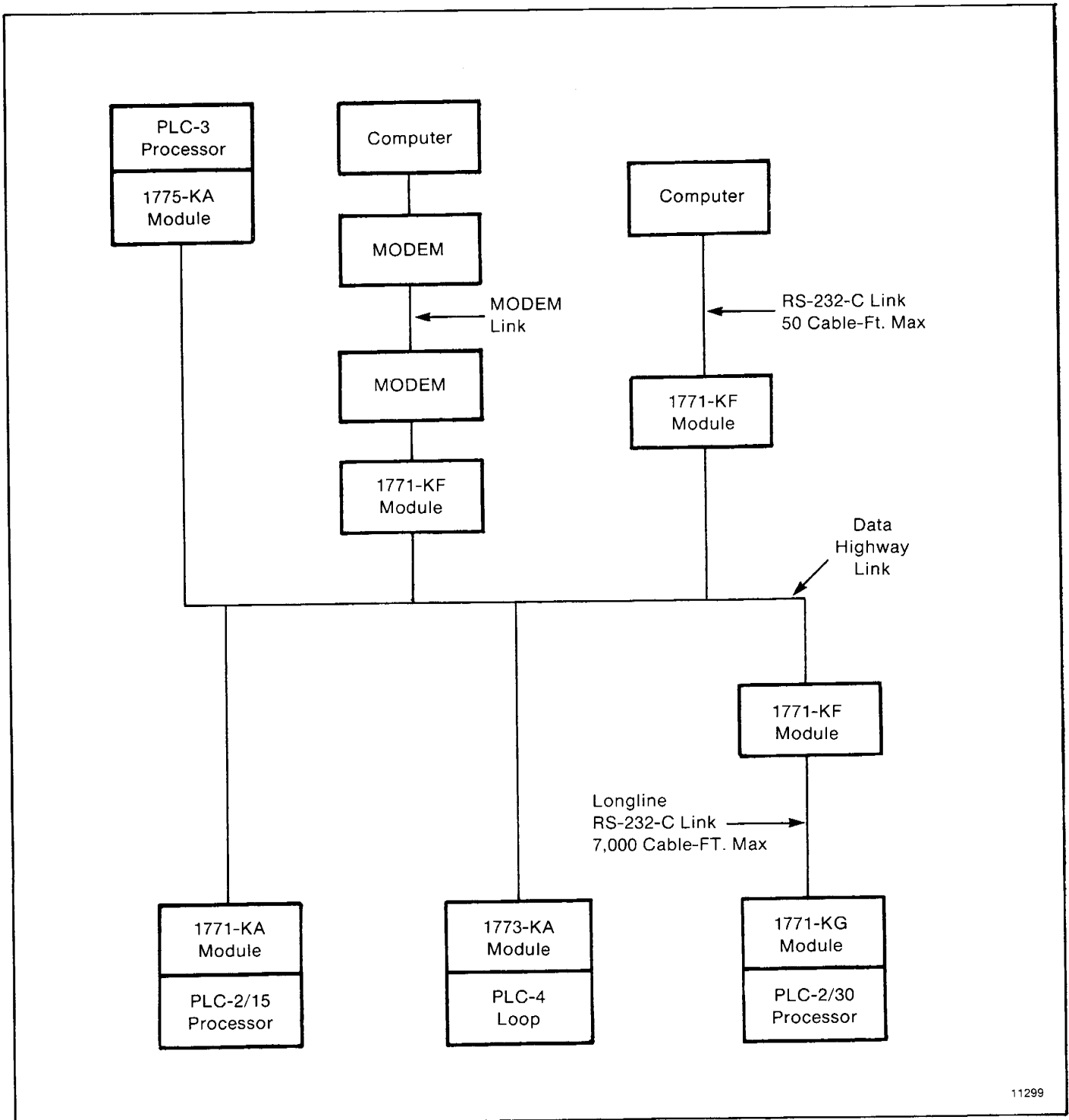
Figure 2.1 — Data Highway Network
