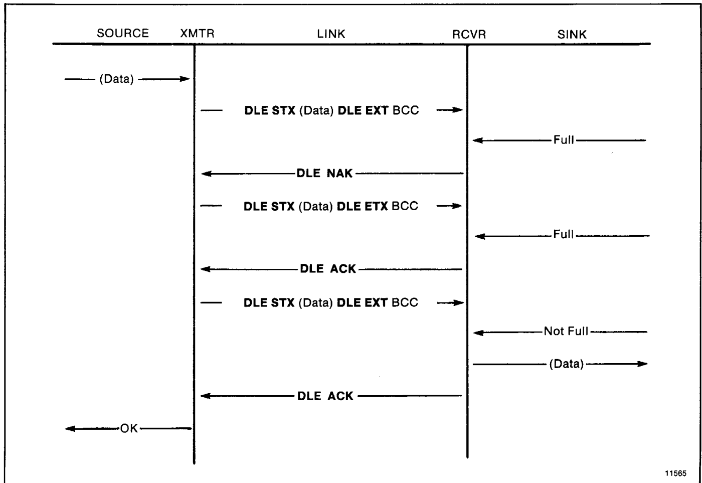
Figure 4.13 — Message Transfer with Message Sink Full
