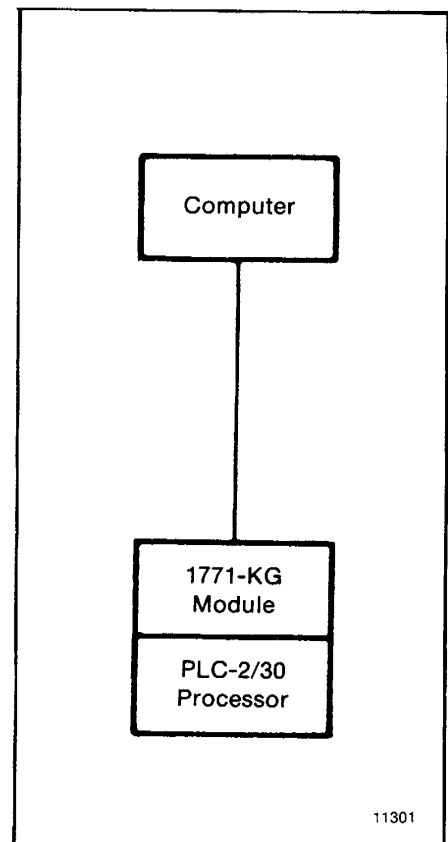
Figure 2.3 — Stand-alone Point-to-Point Link to a Computer
