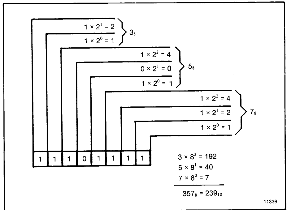
Figure 6.5 — Octal Numbers
