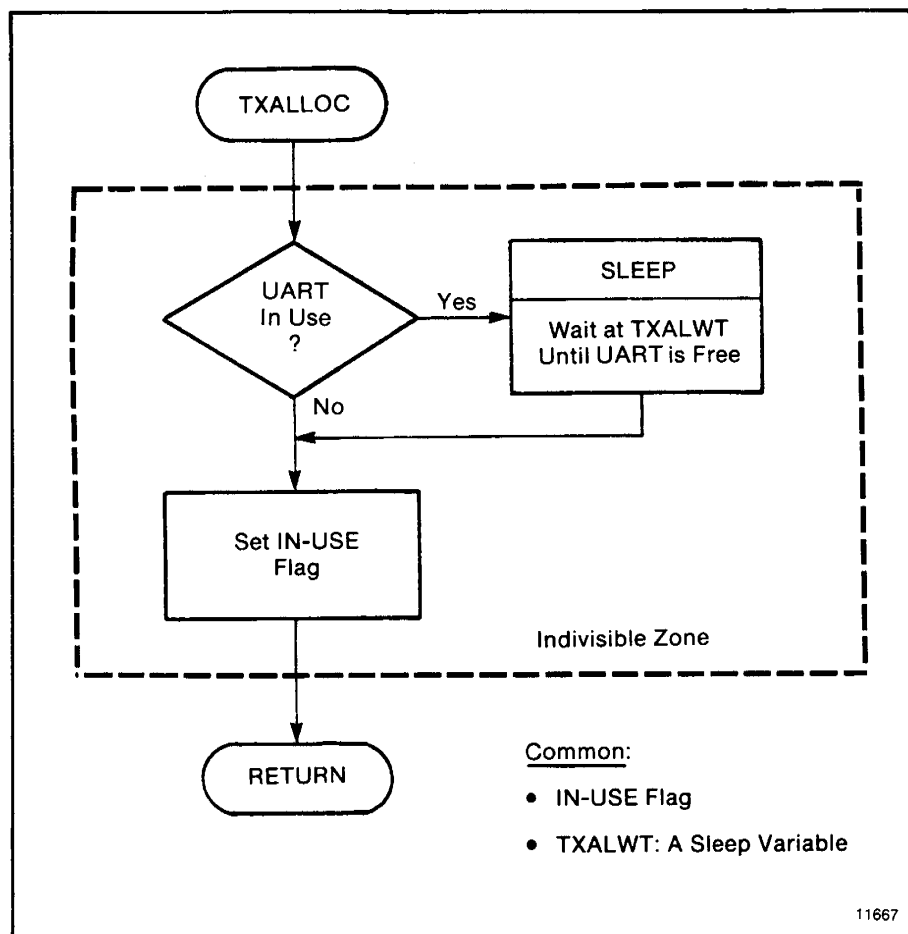
Figure B.15 — TXALLOC Subroutine
