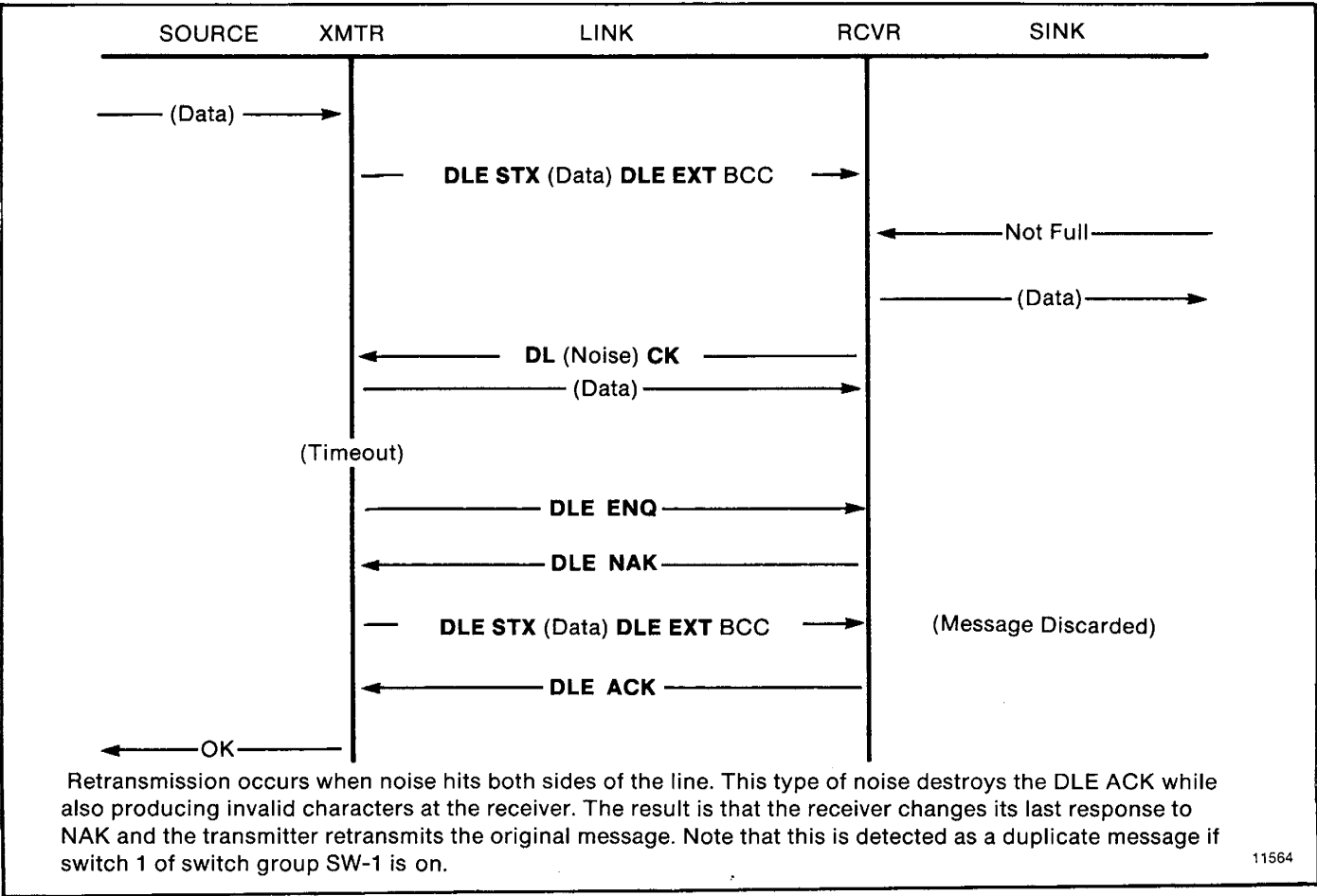
Figure 4.12 — Message Transfer with Retransmission
