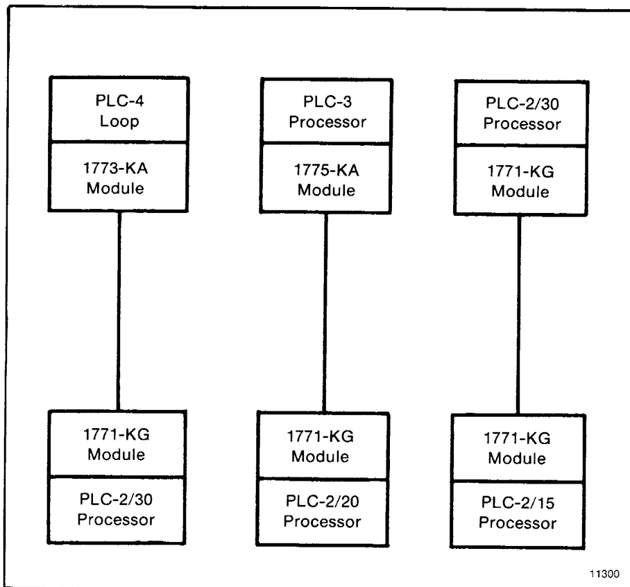
Figure 2.2 — Stand-alone PC to PC Links
