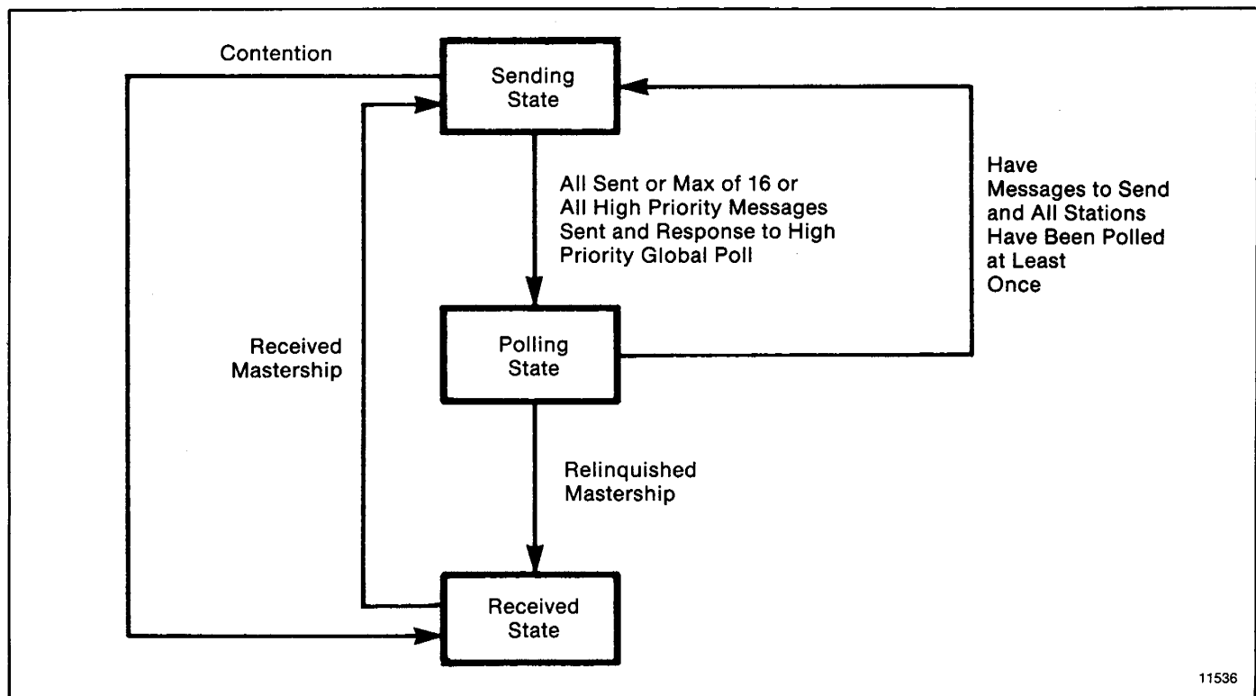
Figure 2.5 — State Transition at Master Station
