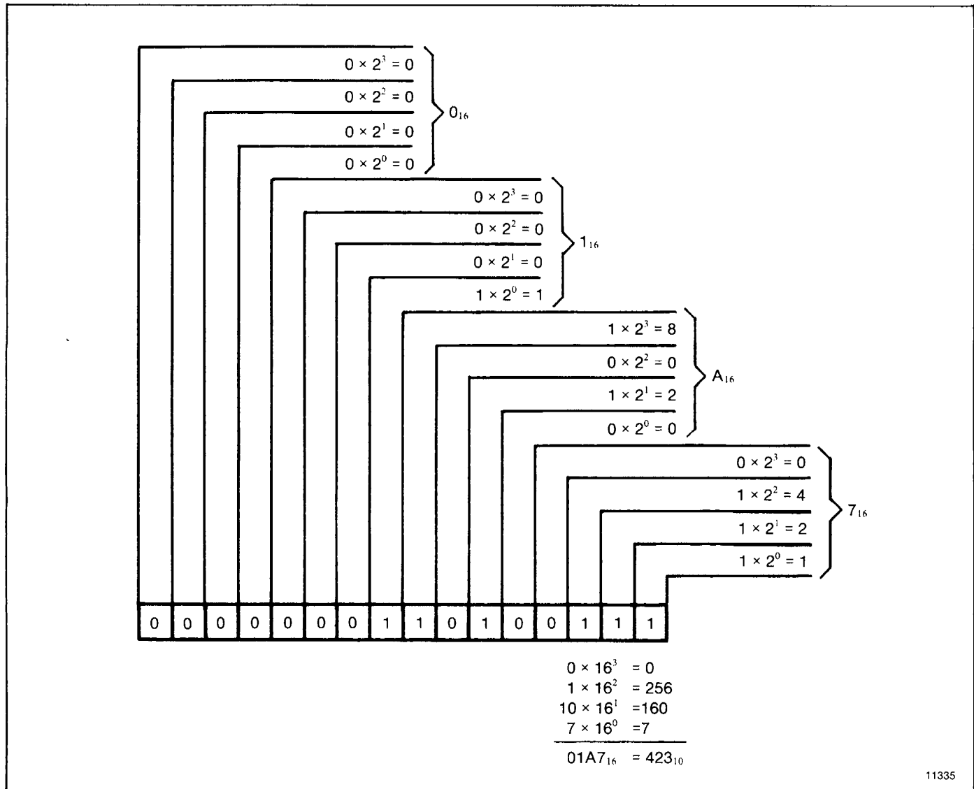
Figure 6.4 — Hexadecimal Numbers
