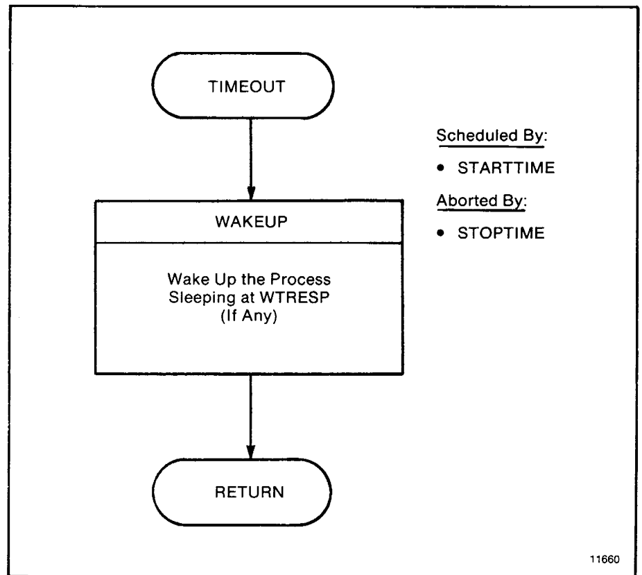
Figure B.7 — TIMEOUT Subroutine
