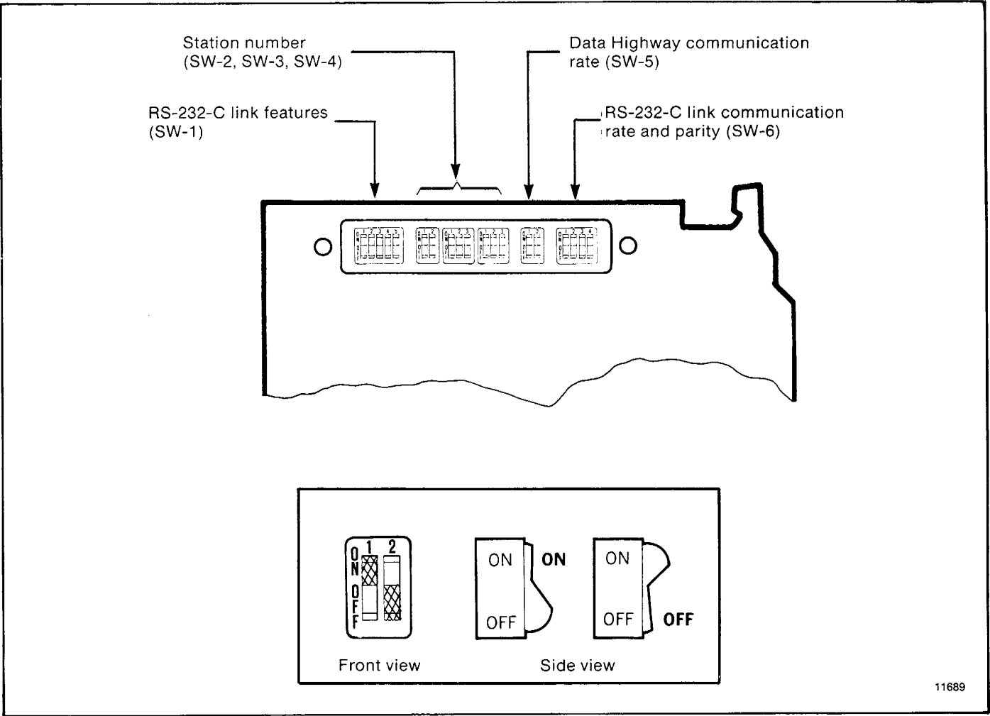
Figure 3.1 — Communication Option Switches
