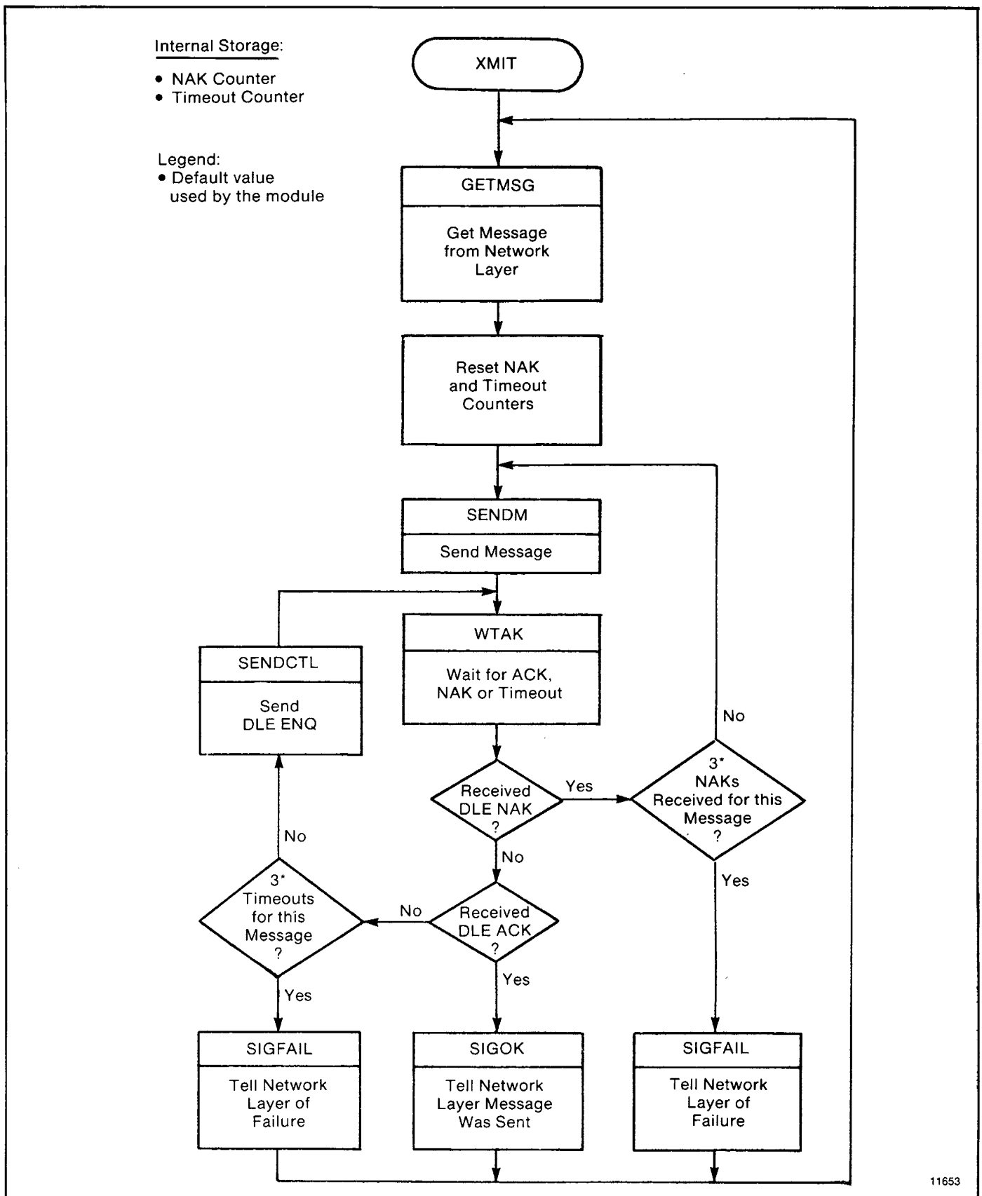
Figure B.2 — Transmitter Routine for Full Duplex Protocol
