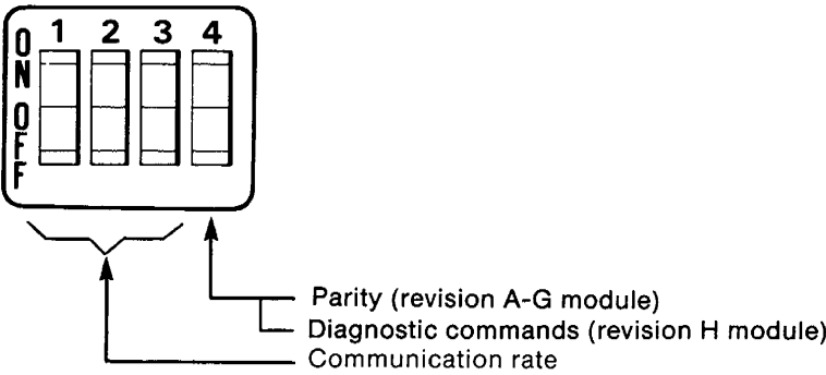
Switch assembly SW-6
