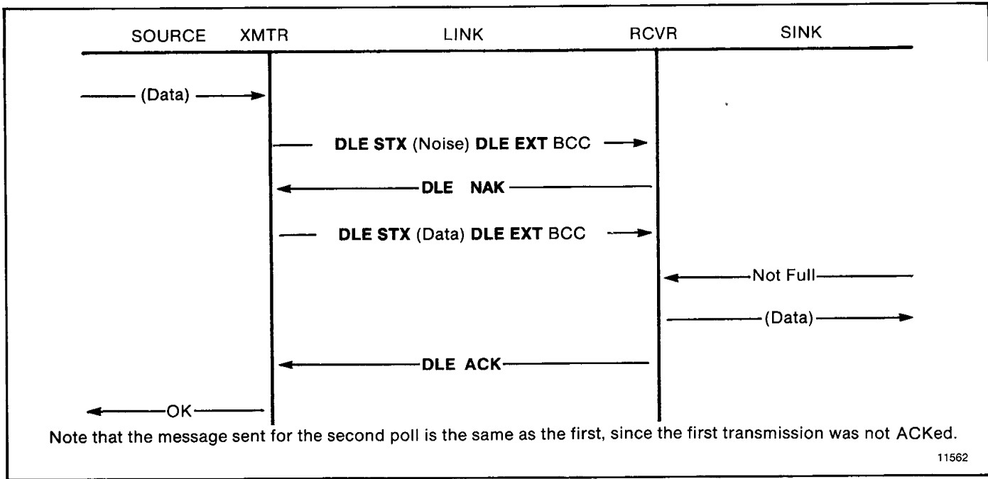
Figure 4.10 — Message Transfer with NAK
