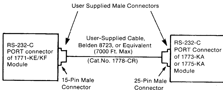
a) Connection Diagram
