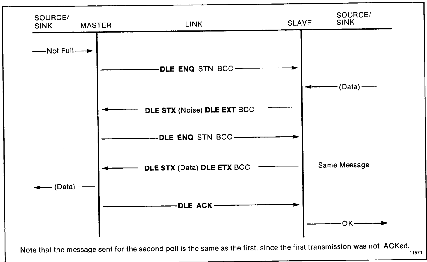
Figure 4.21 — Poll with Message Returned
