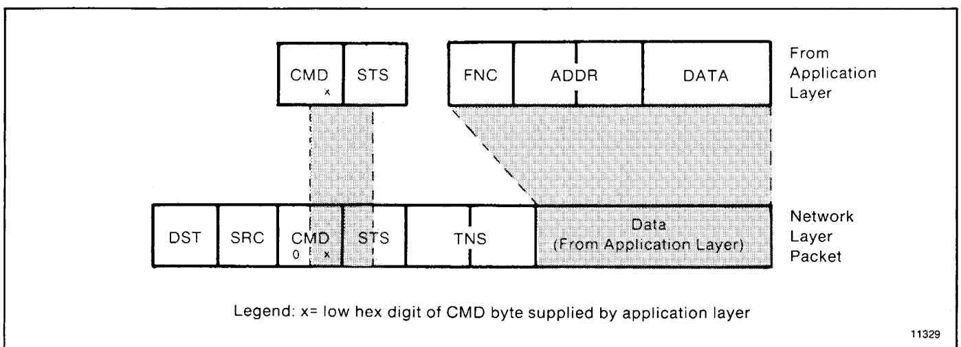
Figure 5.2 — Command Message Packet Format
