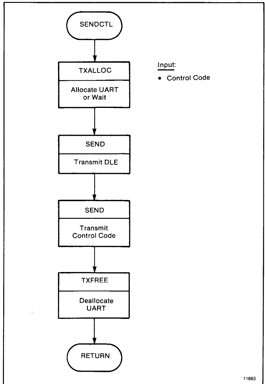
Figure B.11 — SENDCTL Subroutine
