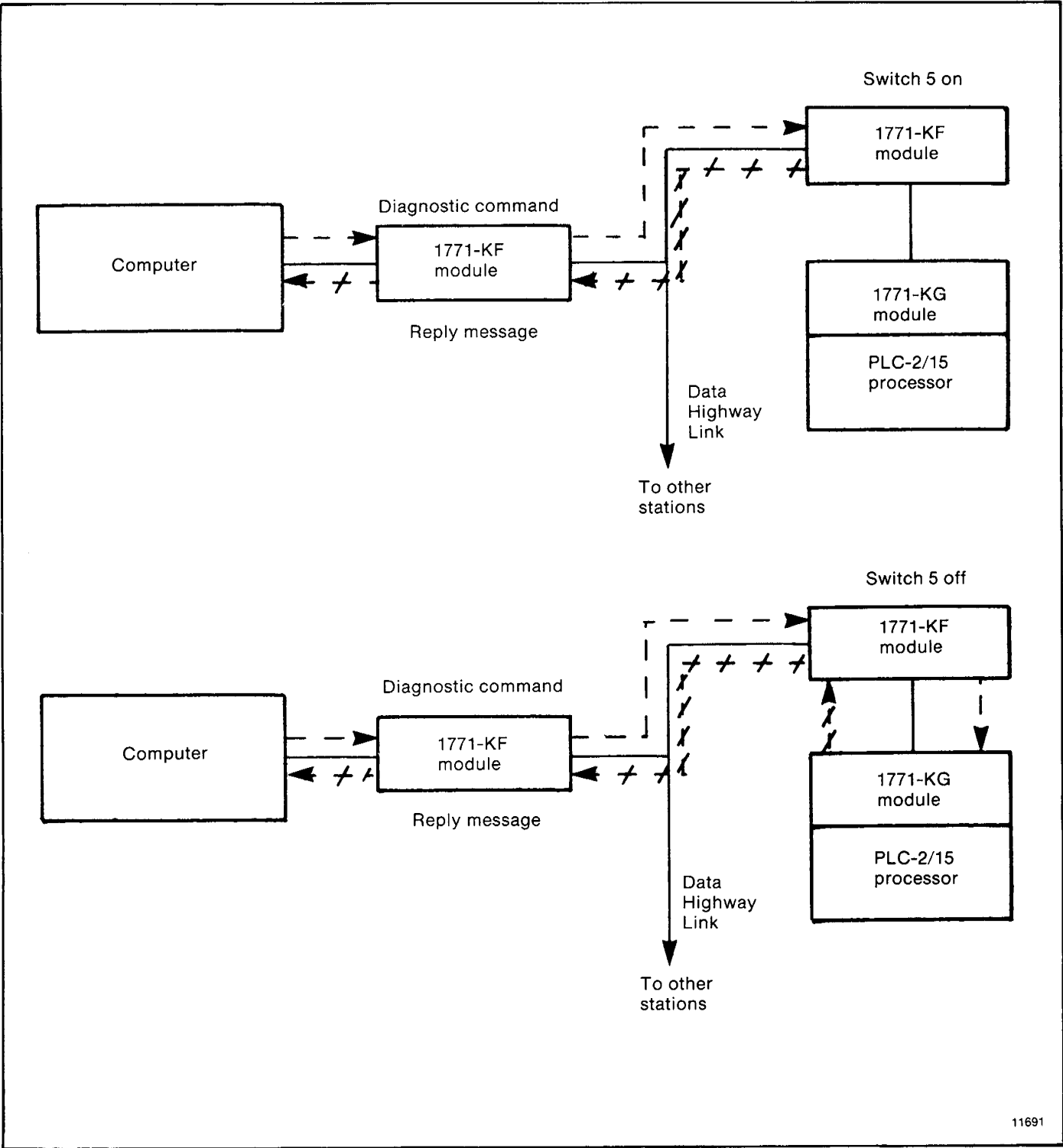
Figure 3.3 — Effect of Switch 5 on Diagnostic Commands
