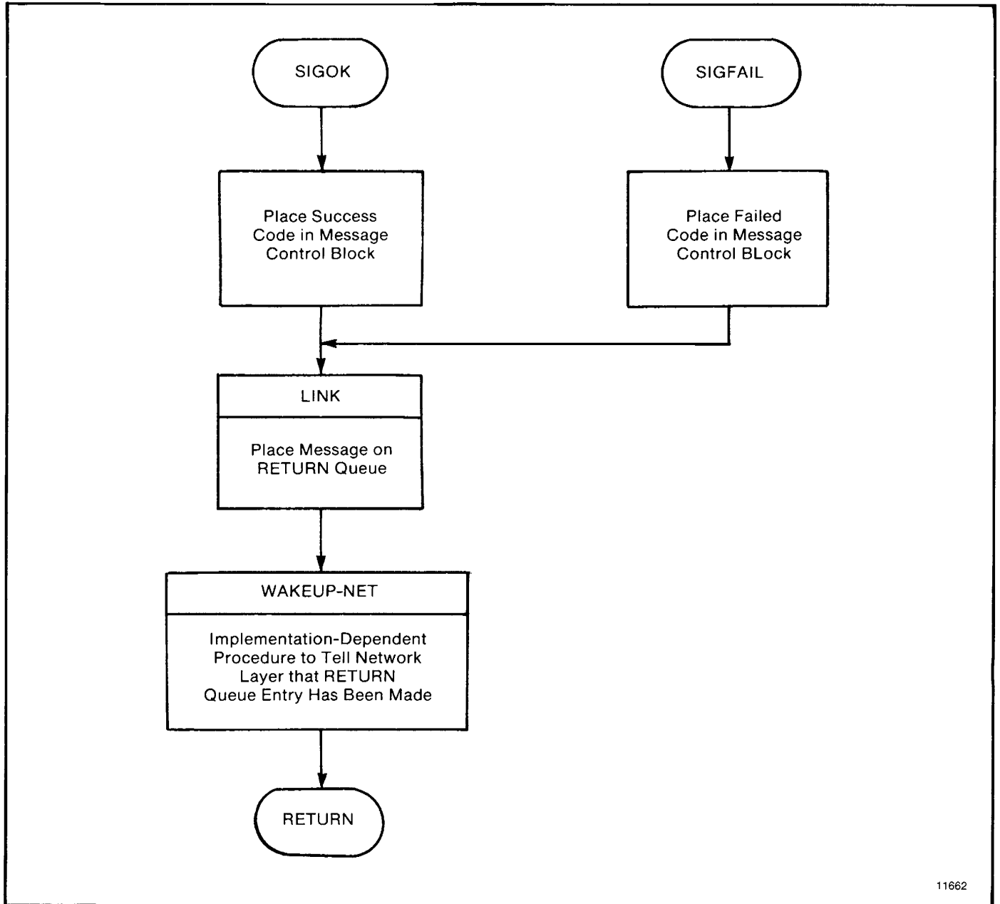
Figure B.9 — SIGOK/SIGFAIL Subroutine
