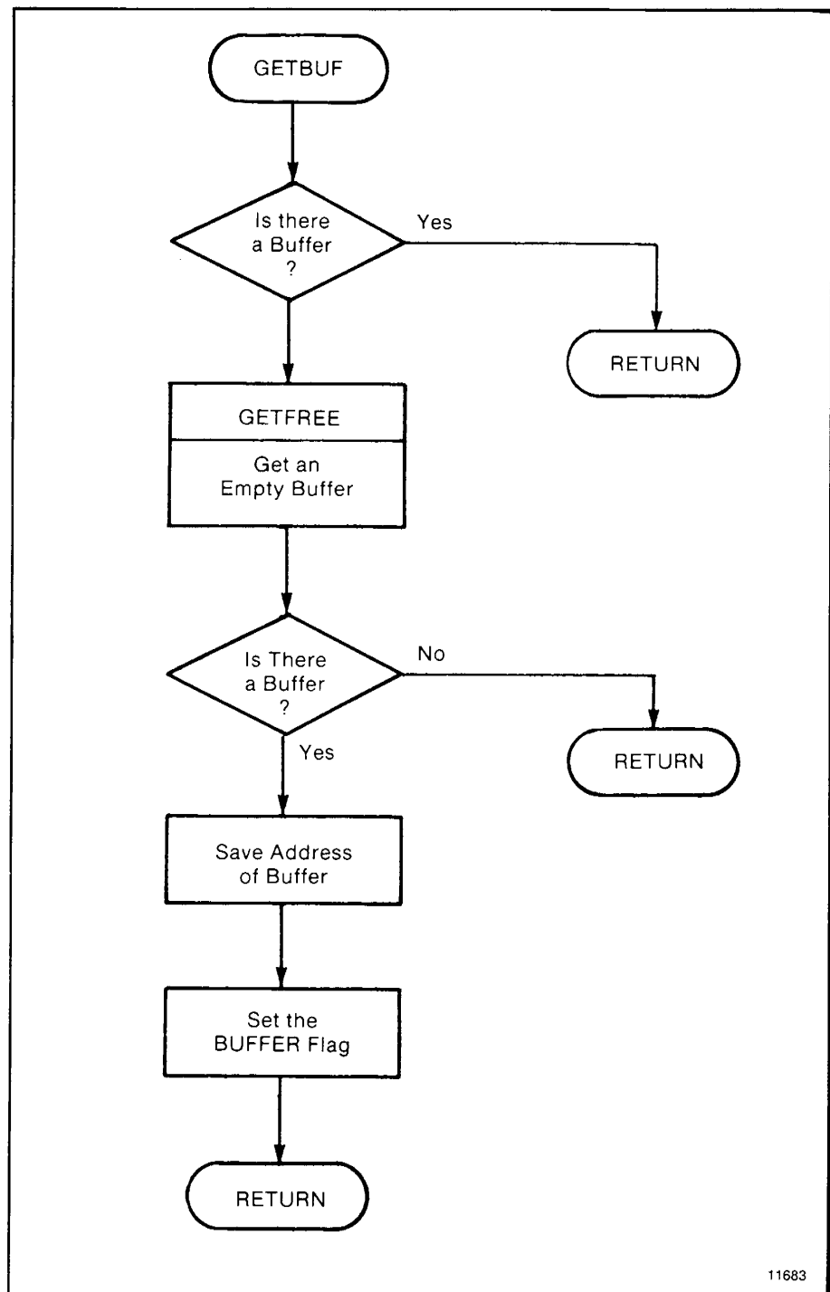
Figure B.29 — GETBUF Subroutine
