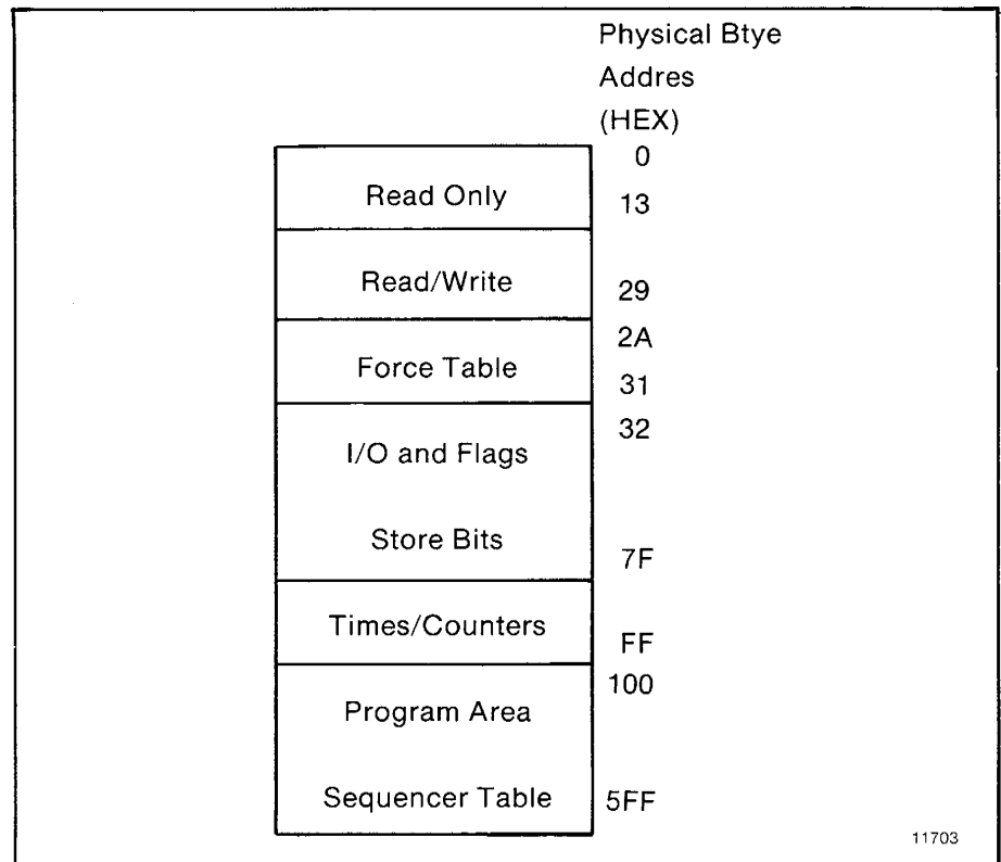
Figure 6.9 — PLC-4 Physical Memory
