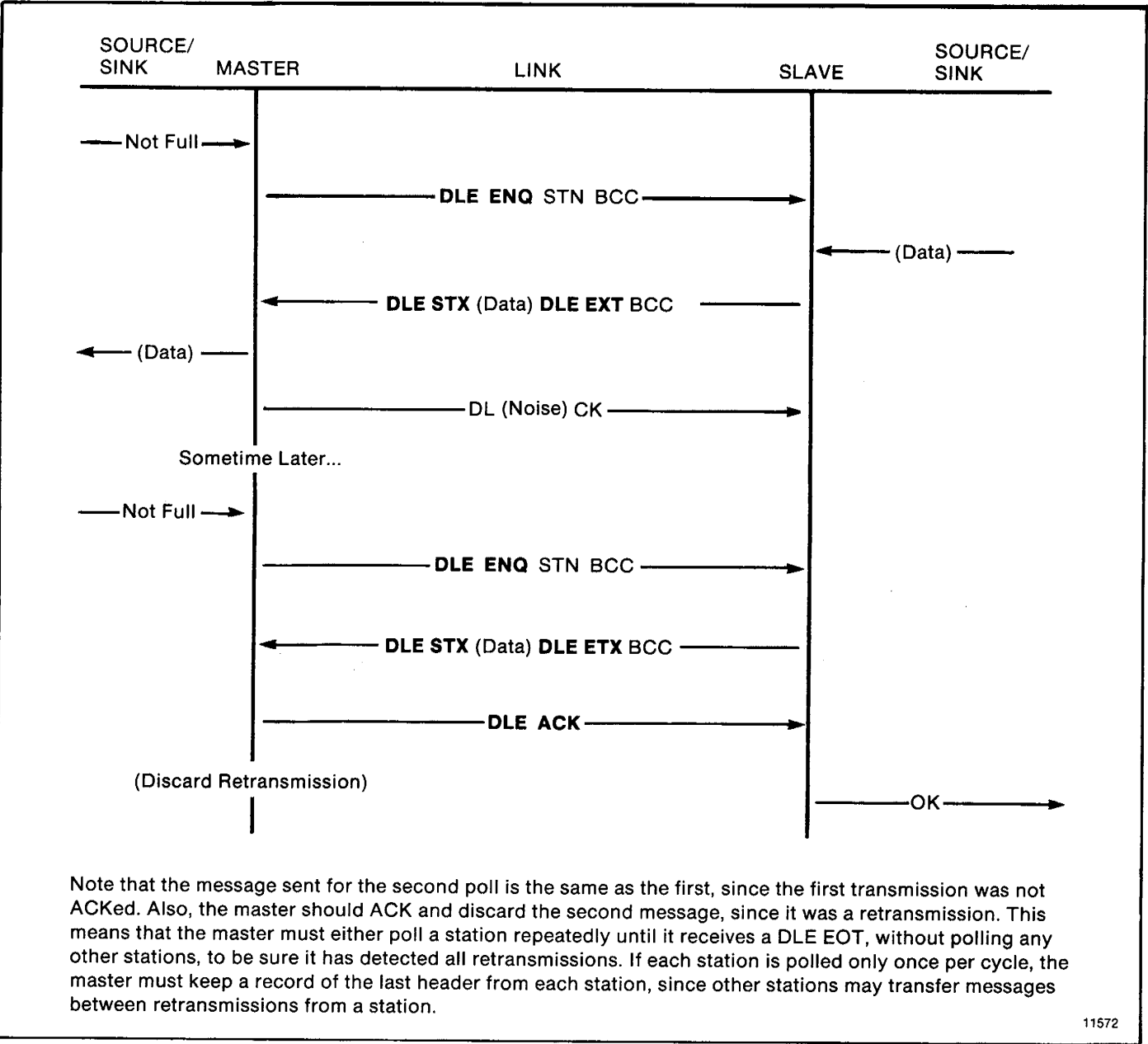
Figure 4.22 — Duplicate Message Transmission
