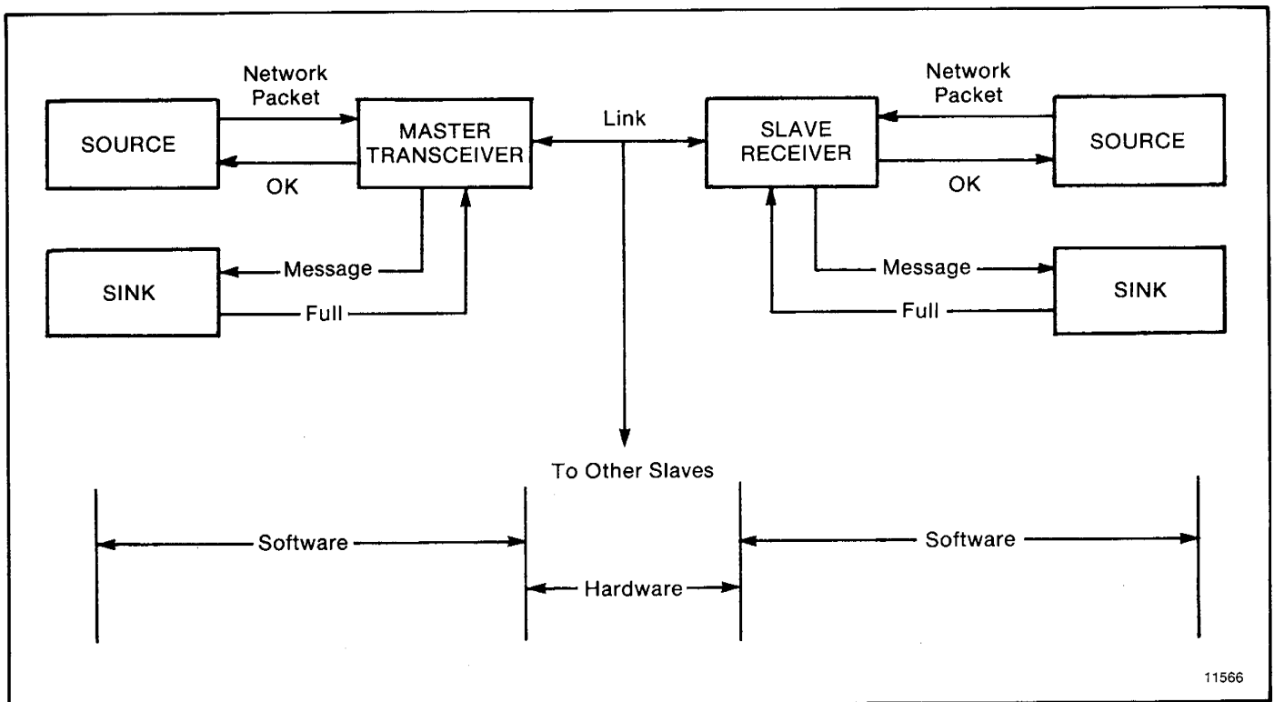
Figure 4.15 — Slave Transceiver
