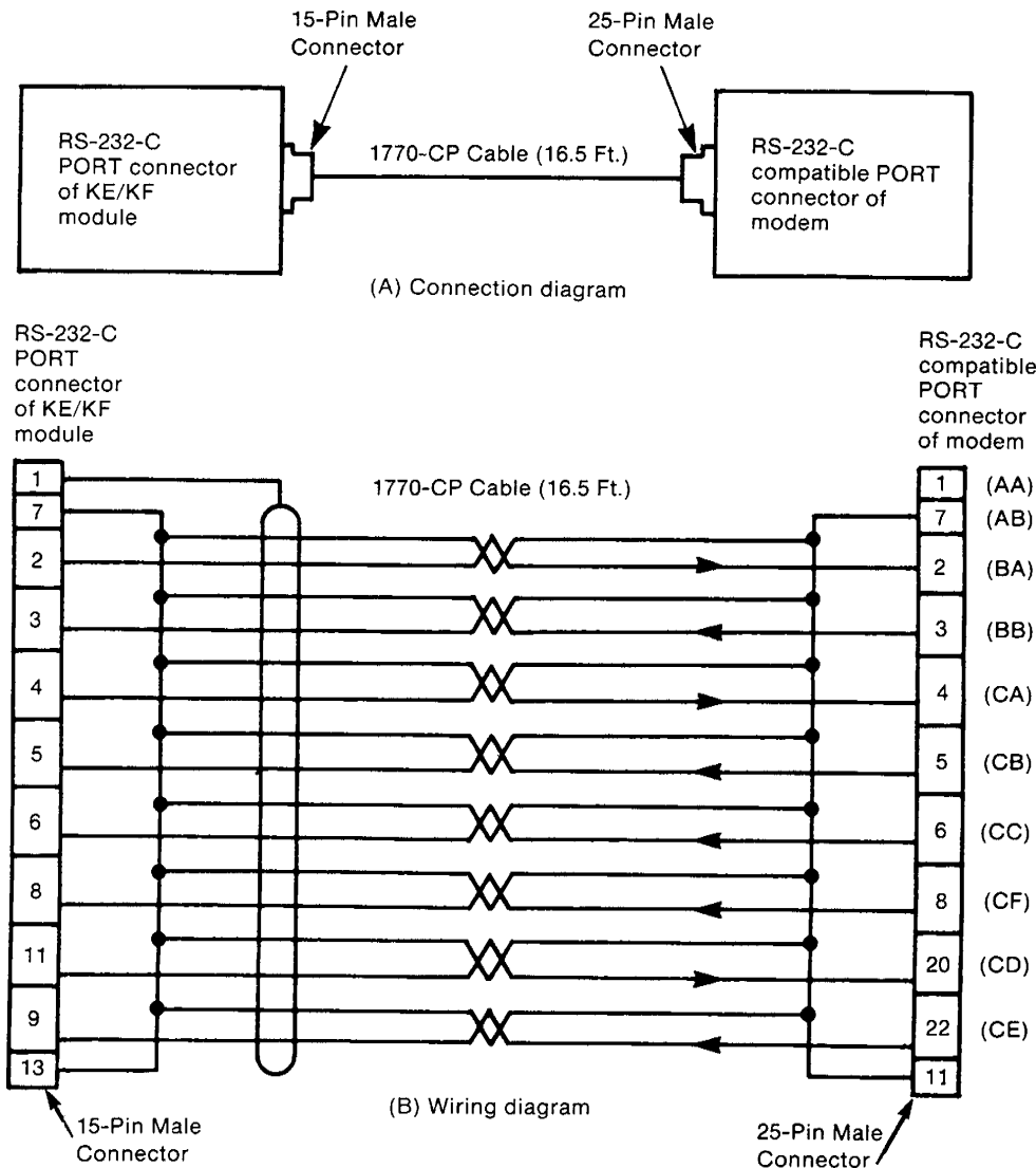
Figure 3.10 — Connection to a Modem
