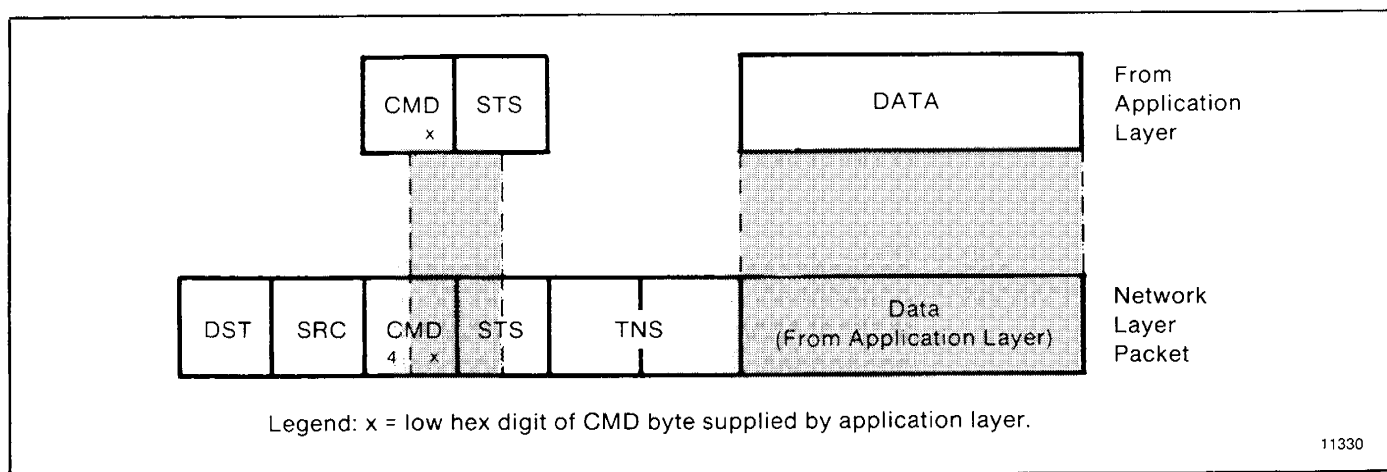
Figure 5.3 — Reply Message Packet Format
