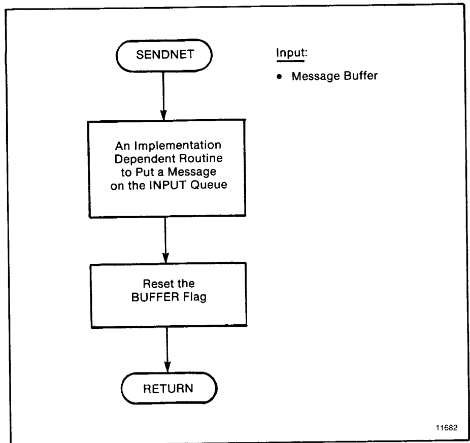
Figure B.28 — SENDNET Subroutine
