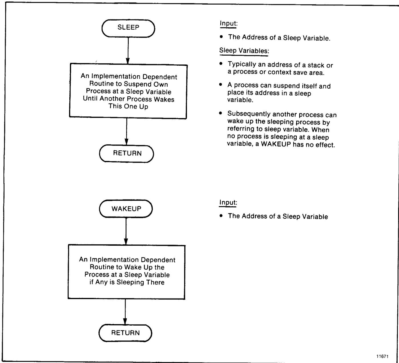
Figure B.18 — SLEEP and WAKEUP Subroutines
