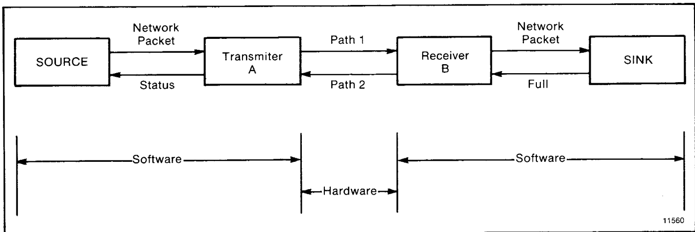
Figure 4.6 — Protocol Environment
