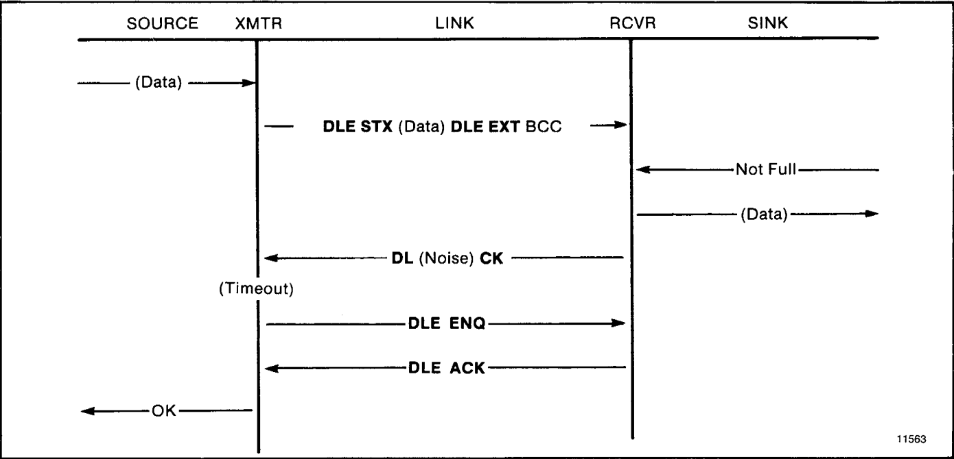
Figure 4.11 — Message Transfer with Timeout & ENQ
