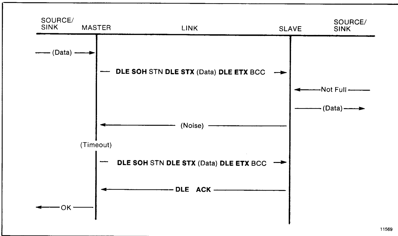
Figure 4.19 — Message Transfer with ACK Destroyed
