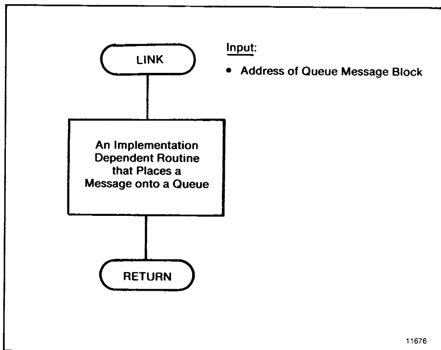
Figure B.23 — LINK Subroutine
