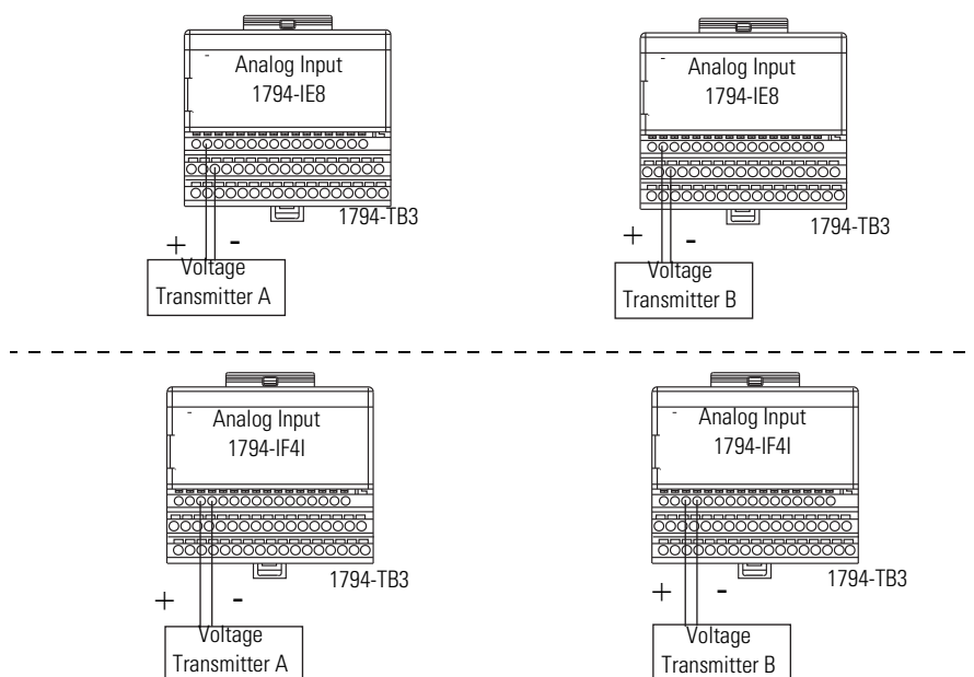
Figure 3.9 FLEX I/O Analog Input Module Wiring in Voltage Mode
