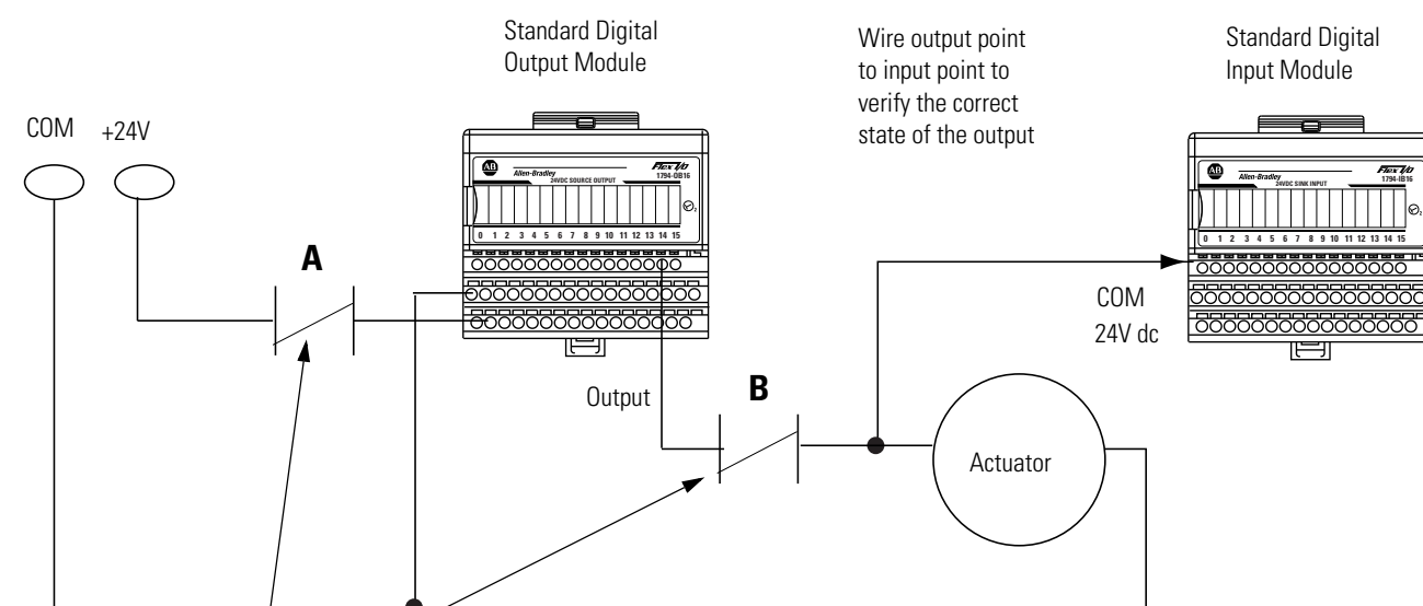
Figure 3.5 ControlLogix/FLEX I/O Standard Output Module Wiring
