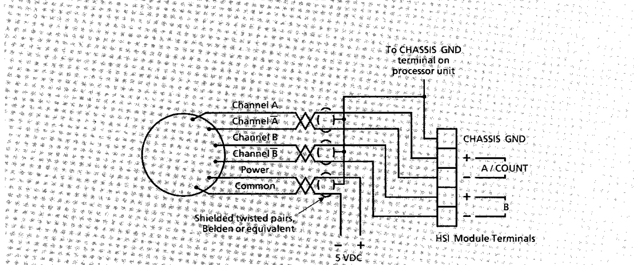
Differential wiring connections for a Bulletin 845N encoder
