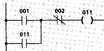
A typical hold-in rung
