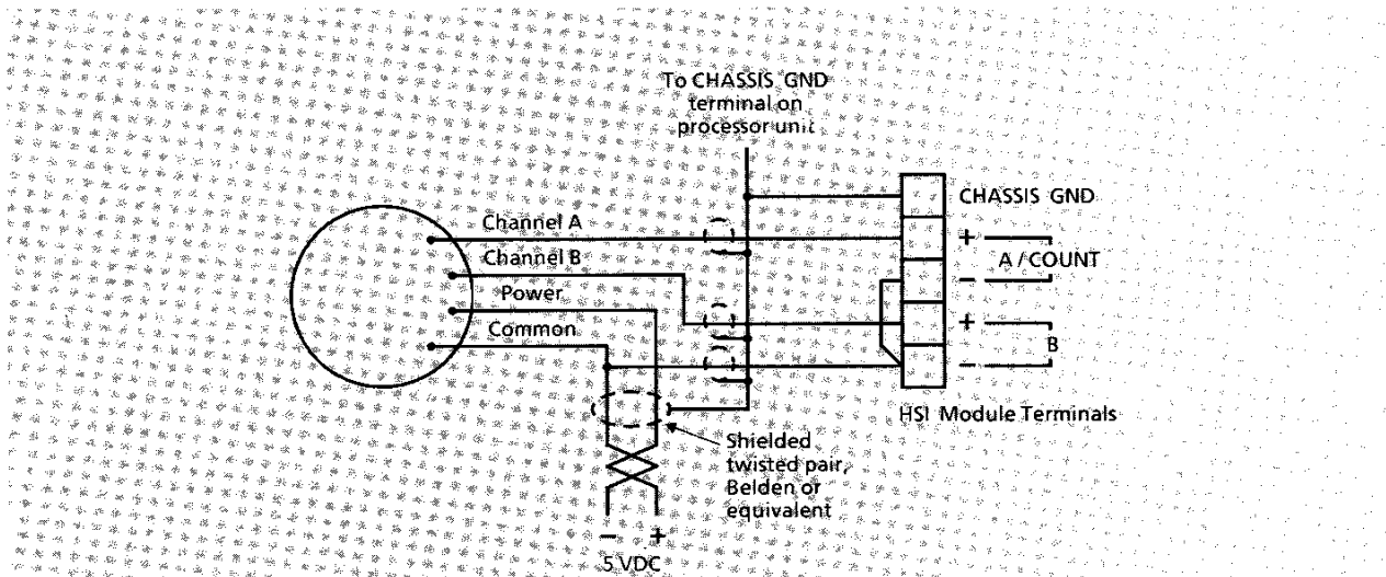
Single-ended wiring connections for a Bulletin 845N encoder
