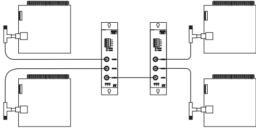
Figure 2—Active hubs can be cascaded for greater distances.
