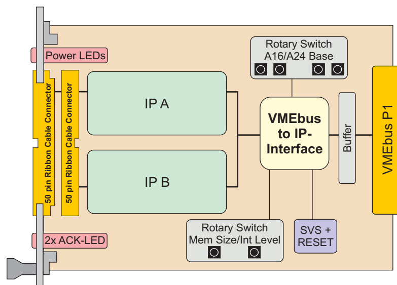
Figure 1-1 : Block Diagram
