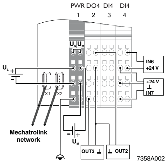
Figure 7 Connection example
