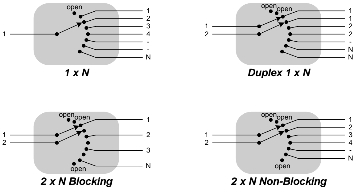
FIGURE 1-2: SM8001 / 8002 SWITCHES
