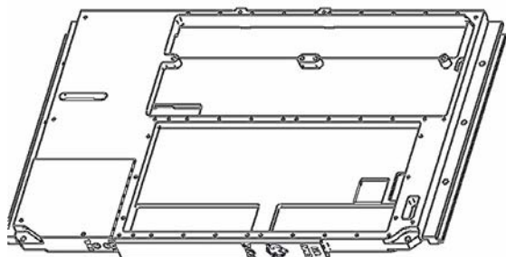
Figure 5: Thermal Frame with VITA 20-2001 PMC Cooling Surfaces and Mid-Plane Thermal Shunt
