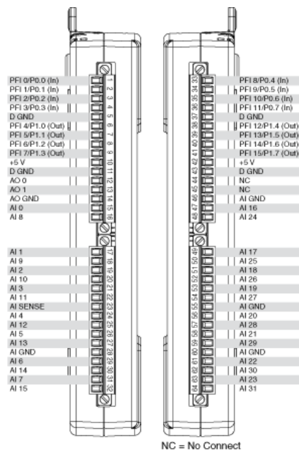
USB-6218 Pinout
