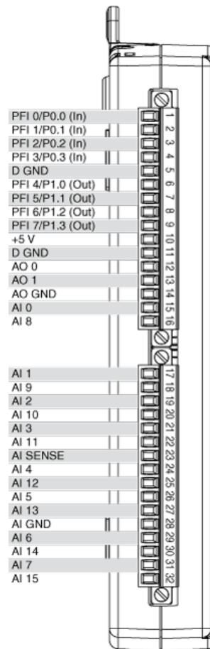
USB-6211/6215 Pinout
