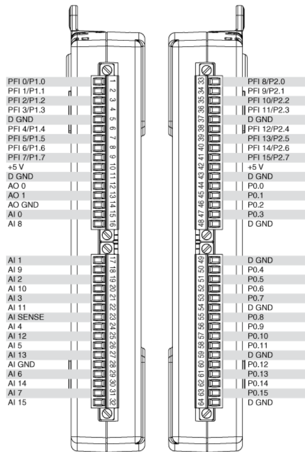
USB-6212/6216 Pinout
