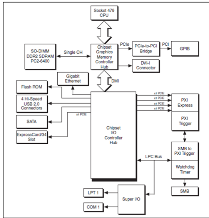
Figure 2. NI PXIe-8108 Block Diagram
