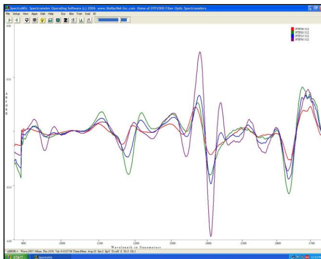
2 nd Derivative spectra of Ready to Eat Food (samples provided by USDA)
