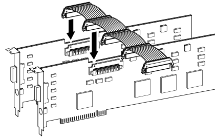
Attaching a TDM ribbon cable
