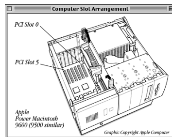
Slot numbering for 9600
