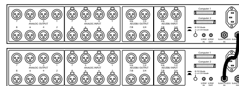
Connecting multiple audio interfaces
