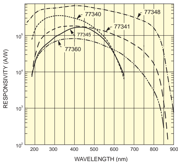
Typical responsivity curves of photomultiplier tubes
