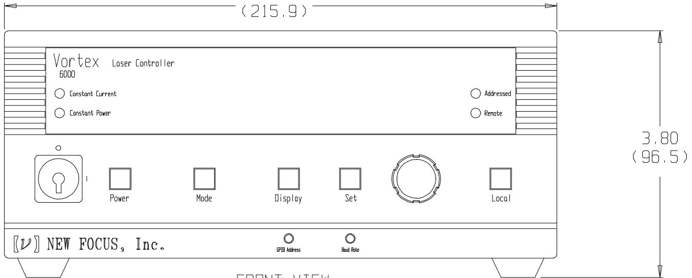
FRONT VIEW
