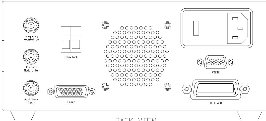
BACK VIEW
