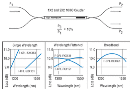
Fig. 2—Typical Spectral Response of 10/90 Couplers
