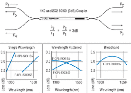
Fig. 1—Typical Spectral Response of 3 dB Couplers
