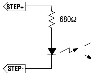
Figure 7 - INPUT CIRCUIT
