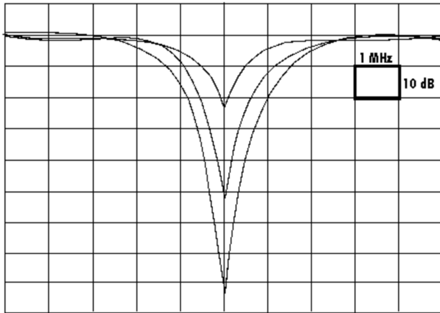
Typical notch loss for one, two and three cavity assemblies for 3 dB bandwidth = 3 MHz.
