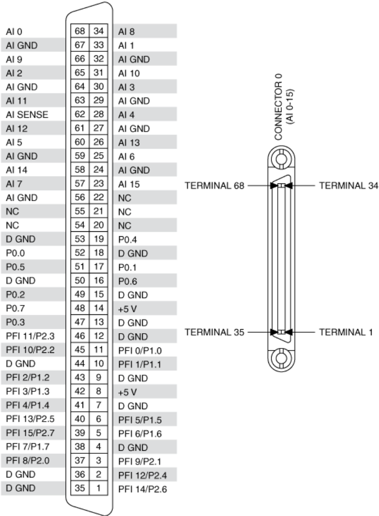
PCI/PXI-6220 Pinout
