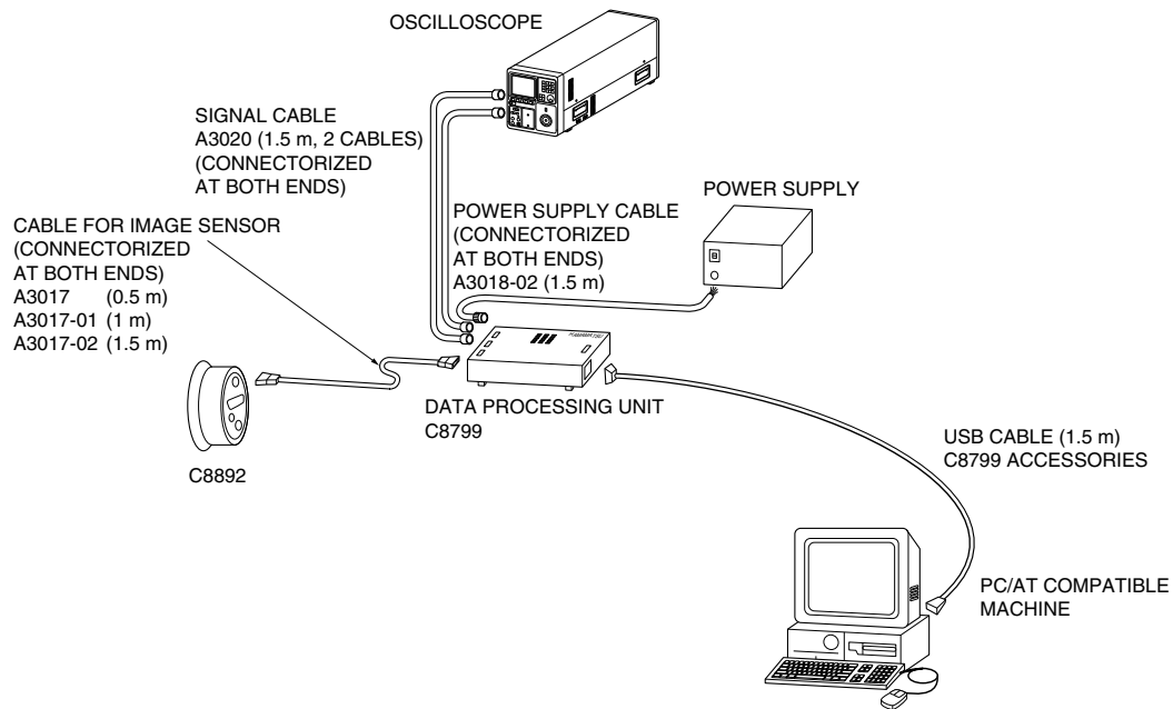
Figure 7-2 Typical setup for multichannel detector head and peripheral devices
