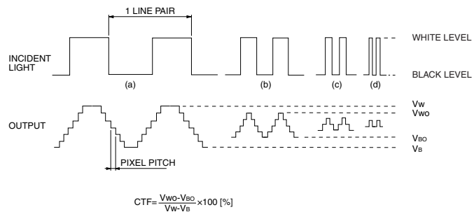
Figure 4-12 CTF characteristics
