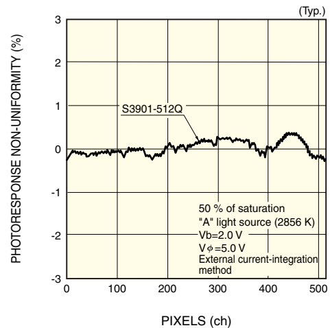
Figure 4-7 Non-uniformity
