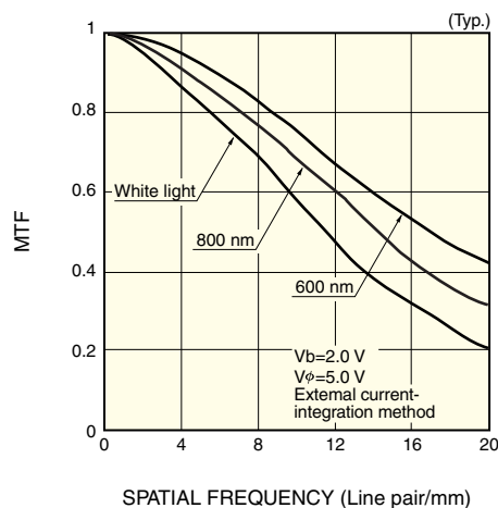
Figure 4-16 MTF (S3904-1024Q)
