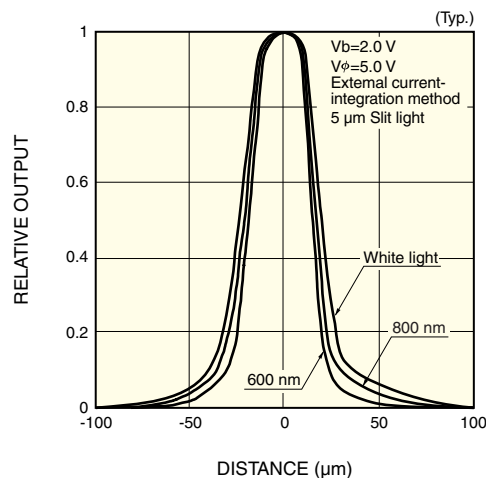
Figure 4-13 Output response to slitted incident light (S3901-512Q)
