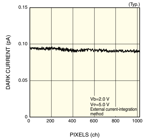
Figure 4-11 Dark current uniformity (S3904-1024Q)
