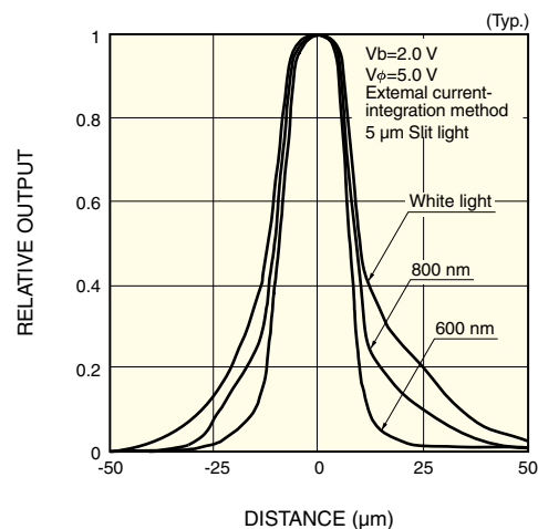
Figure 4-14 Output response to slitted incident light (S3904-1024Q)
