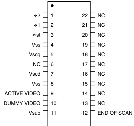
Figure 3-2 Pinout (current output type)
