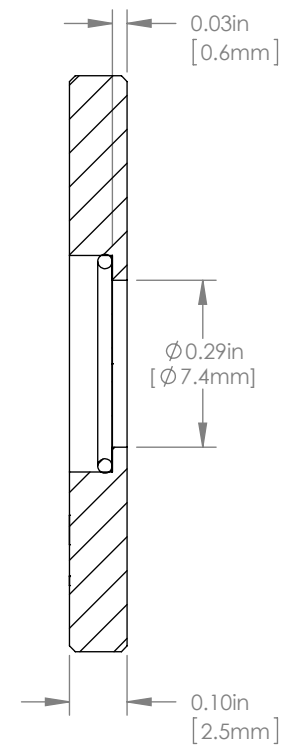
SECTION X-X
