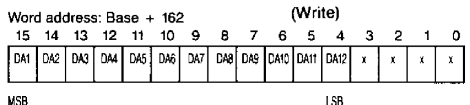
Figure 10b: D/A Channel 1 Register Format
