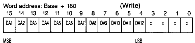
Figure 10a: D/A Channel 0 Register Format
