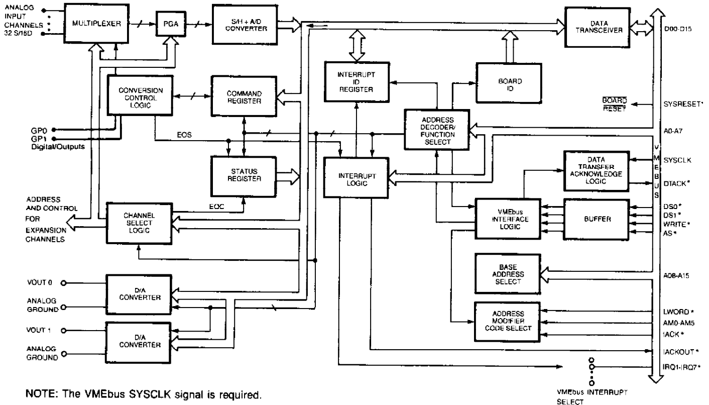
Figure 1. DVME-611/612 Functional Block Diagram
