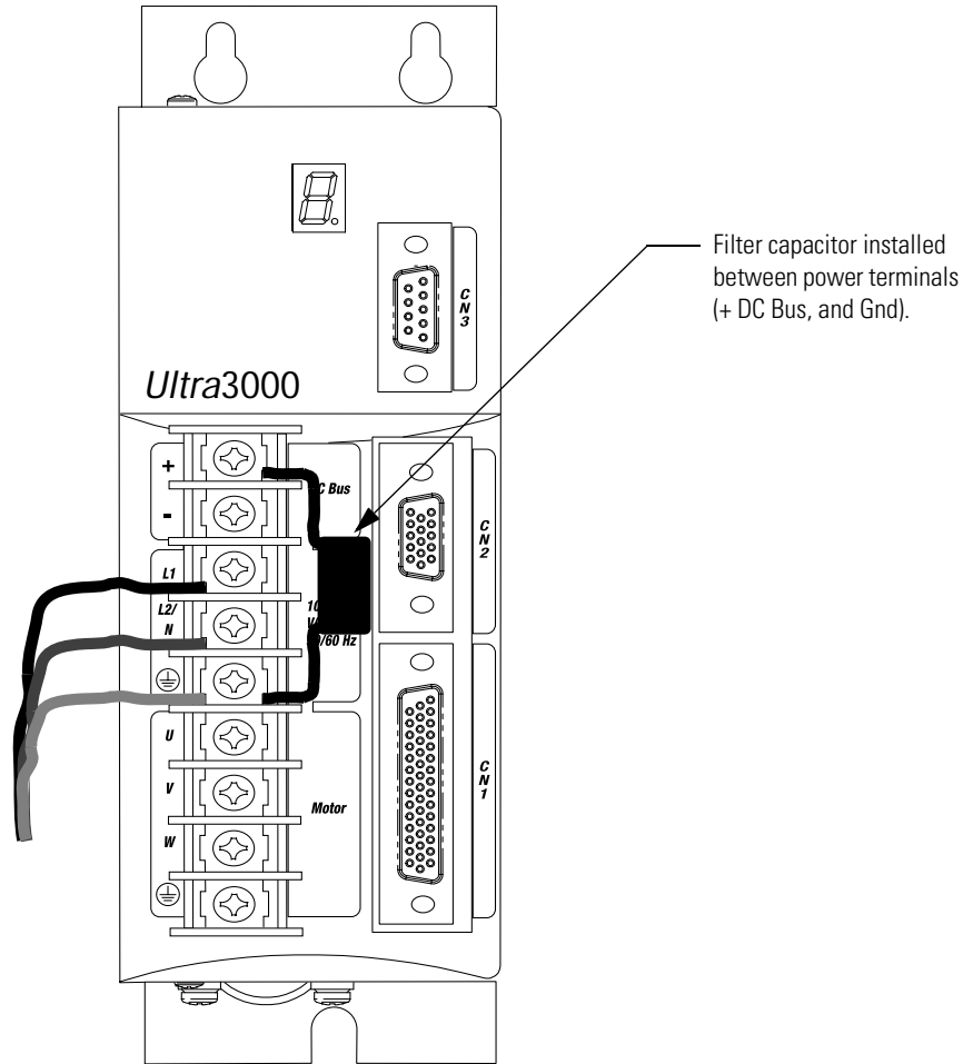
Figure 1 Filter Capacitor Installation on Ultra3000 Drive
