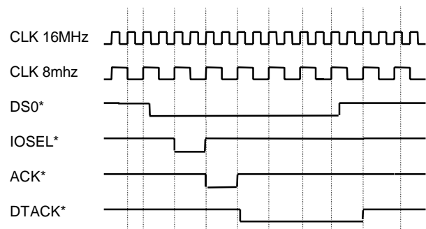
Timing Diagram
