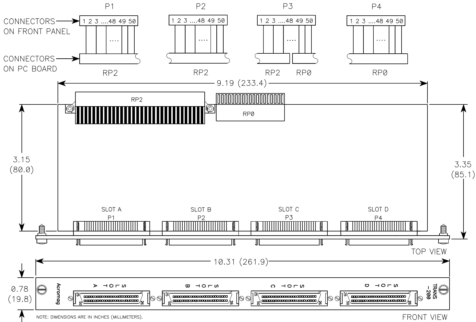
TRANS-200 MECHANICAL DIMENSIONS AND SIMPLIFIED SCHEMATIC
