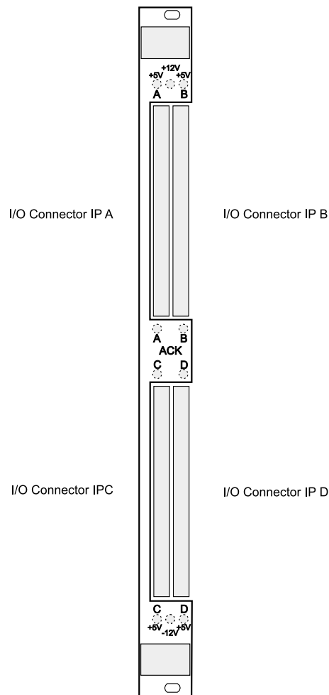
Figure 6-1 : Front Panel
