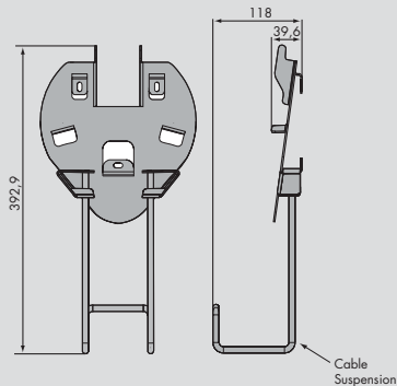
Wall Bracket, rear and side view
