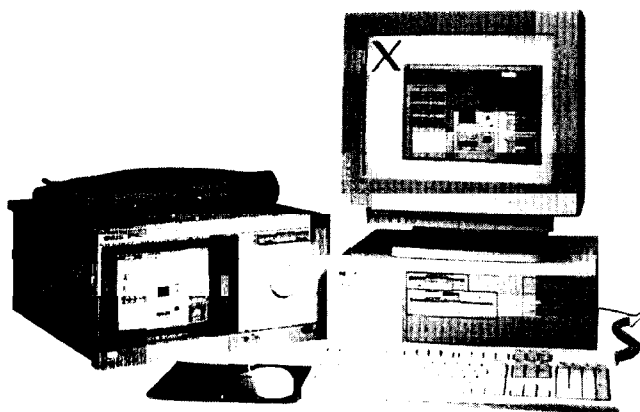
The HP 16500B's menus can be remotely viewed and controlled from a PC or workstation using the X-Window protocol.
