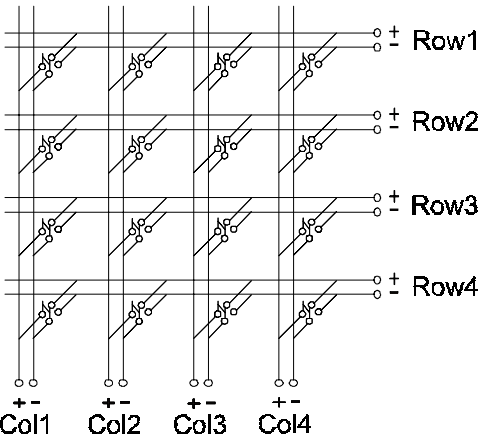
Matrix Switching
