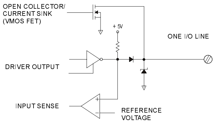
A Simple Digital I/O Circuit
