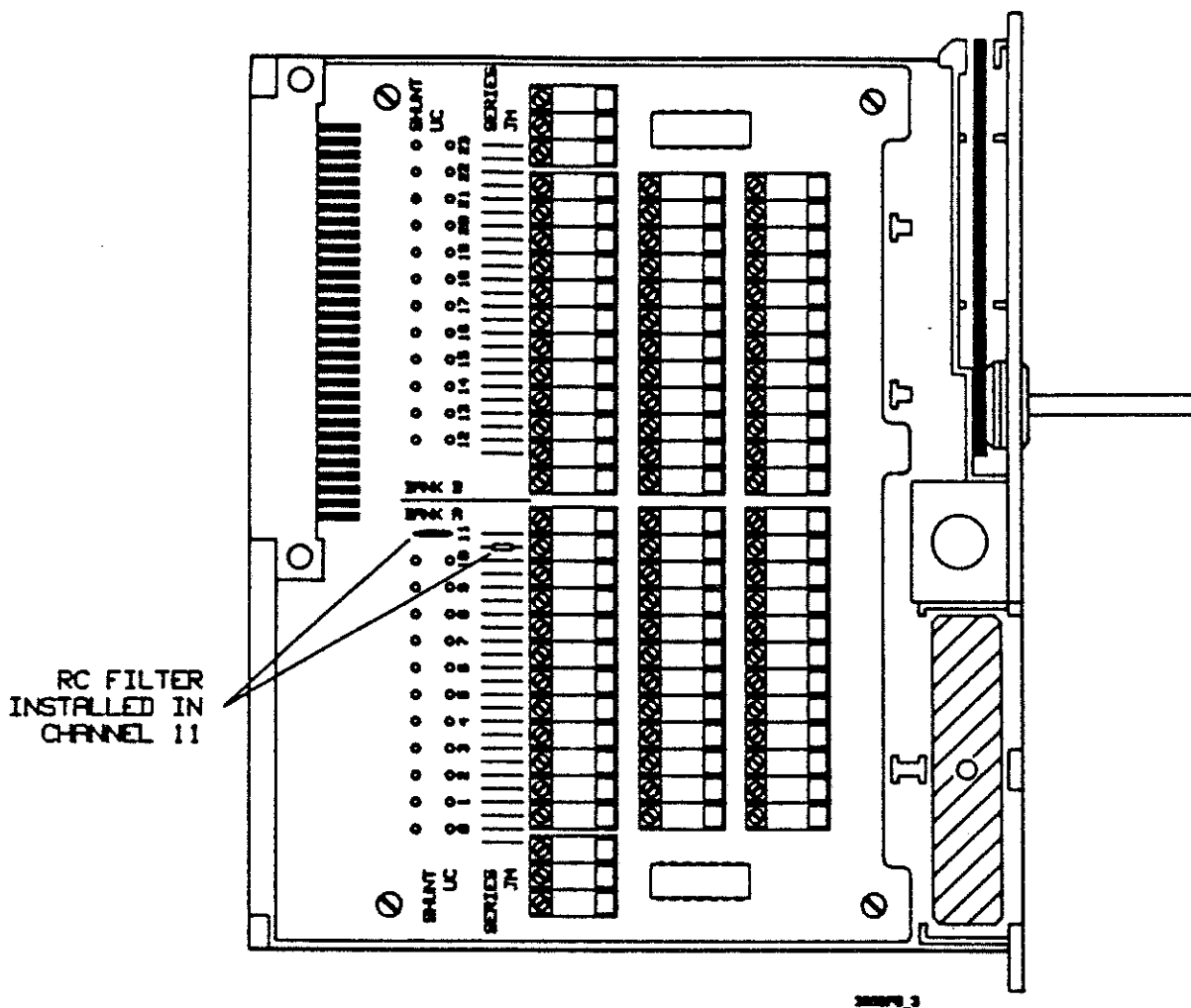
Figure 9-3. Installing Low-Pass Filter
