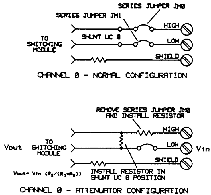
Figure 11-4. Channel Configuration with Attenuator
