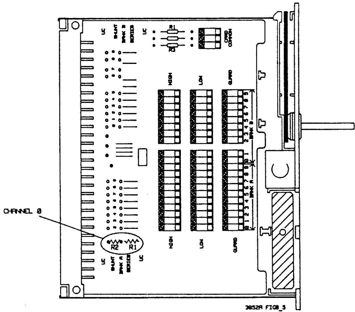
Figure 8-5. Installing Attenuators
