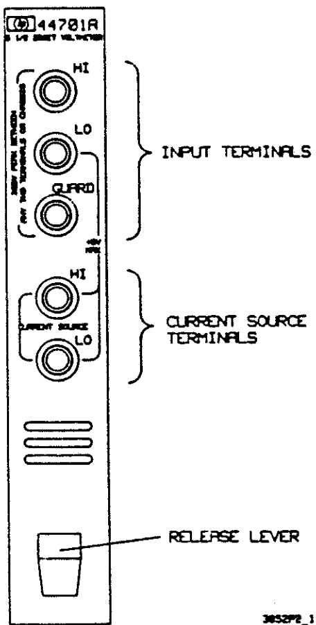
Figure 2-1. HP 44701A Backpanel
