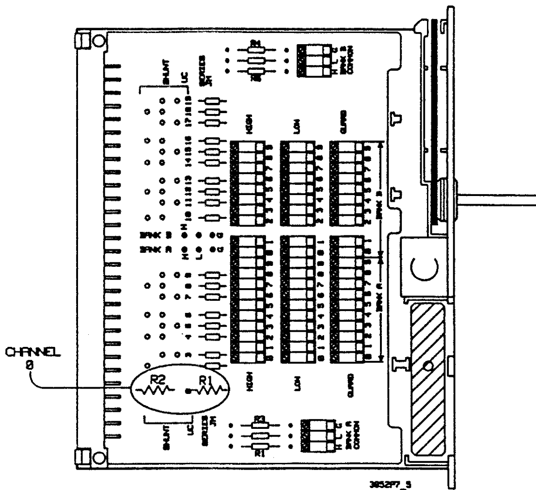
Figure 7-5. Installing Attenuators
