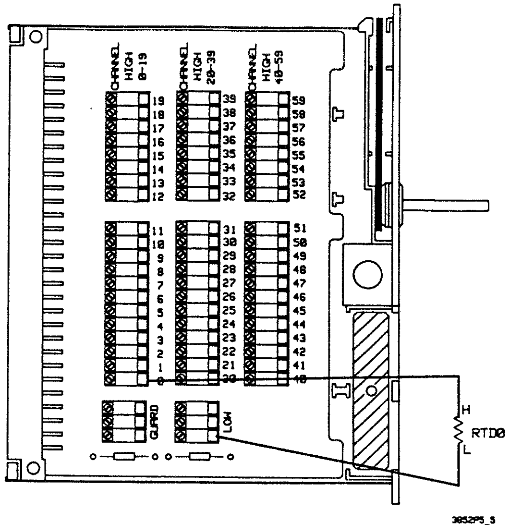
Figure 5-5. Connecting RTDs for Temperature Measurements
