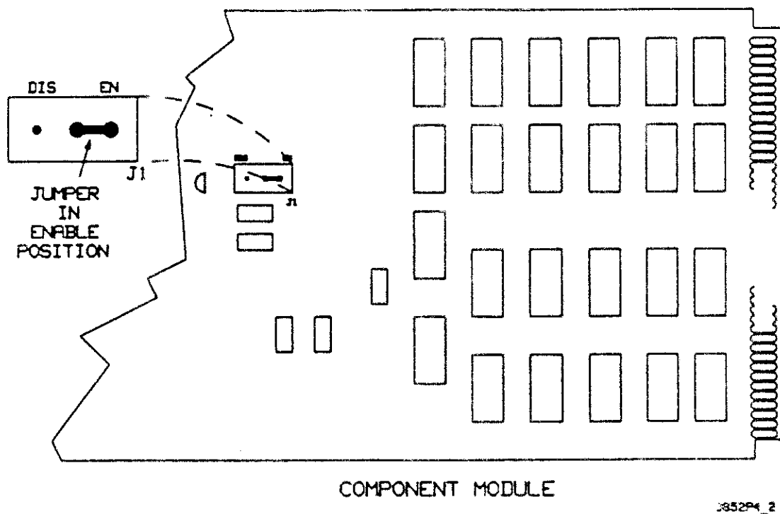
Figure 4-2. Setting the Isolation Jumper
