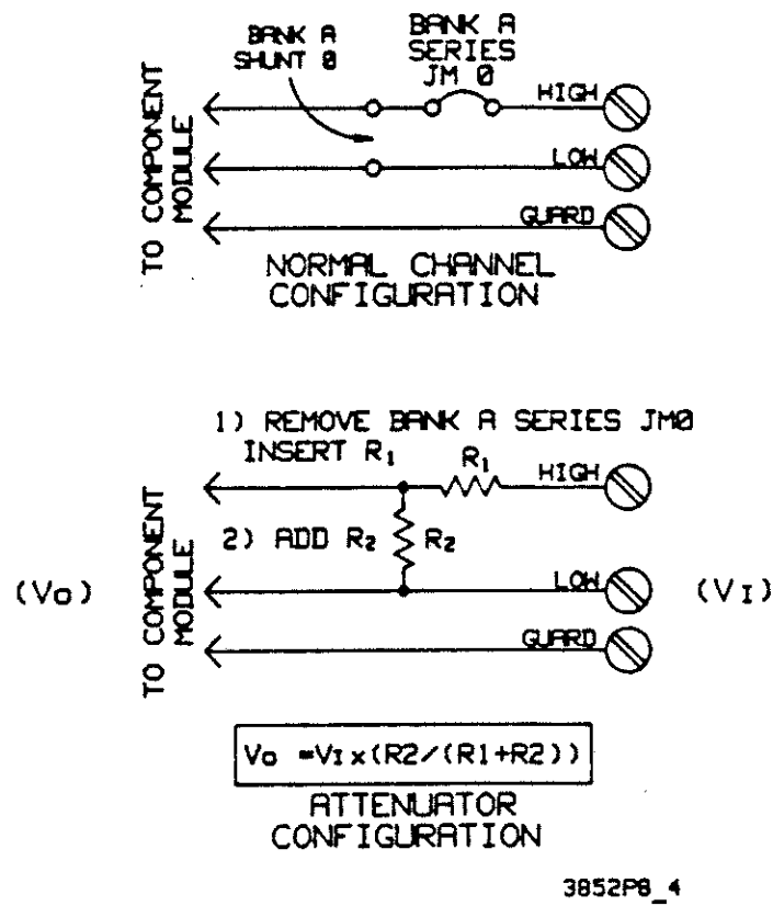
Figure 8-4. Attenuator Channel Configuration
