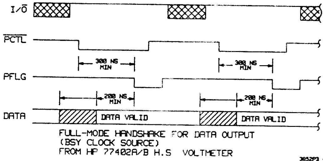
Figure 3-4. Full-Mode Handshake Timing
