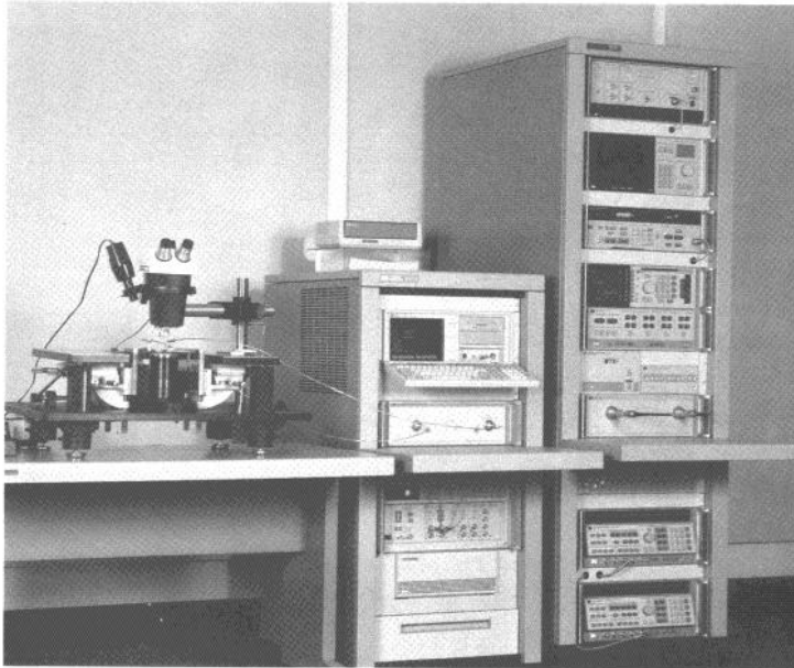
The HP 4142B obtains all DC parameters and provides RF biasing for single connection microwave testing.
