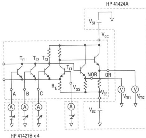
Easily characterize ECL circuits
