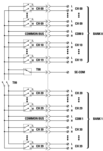
N2260A/66A MUX Module Terminal Block
