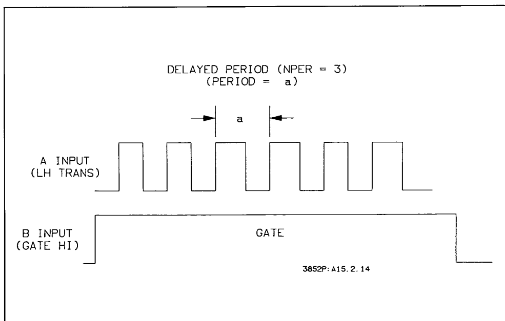
Figure 2-14. Example: Delayed Period Measurements (PERD)
