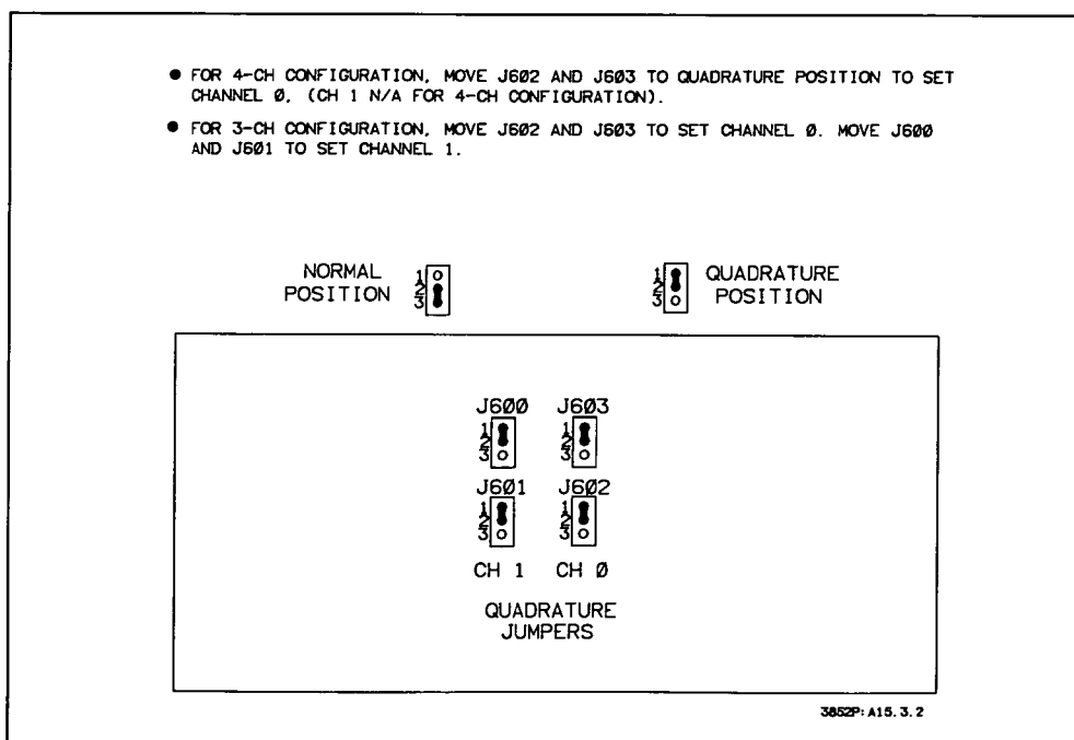
Figure 3-2. Setting Quadrature Jumpers
