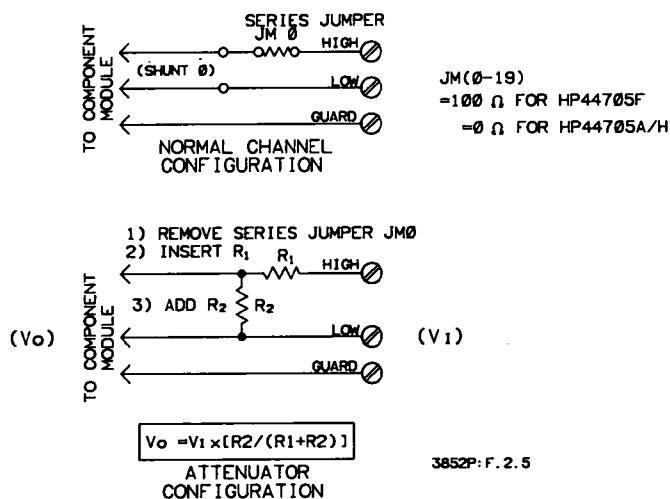
Figure 2-4. HP 44705 Attenuator Channel Configuration
