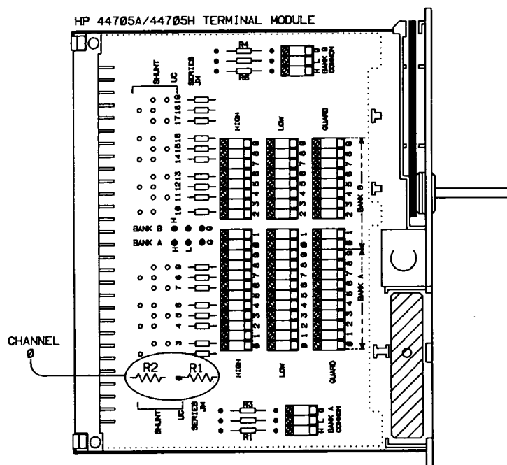
CH 0 ATTENUATOR INSTALLATION
