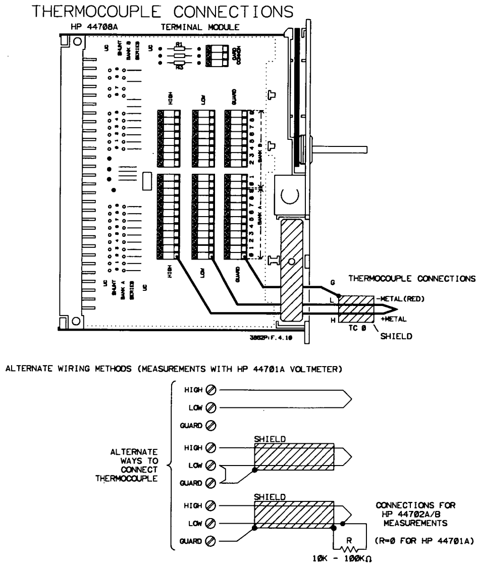
Figure 4-9. HP 44708 Thermocouple Connections
