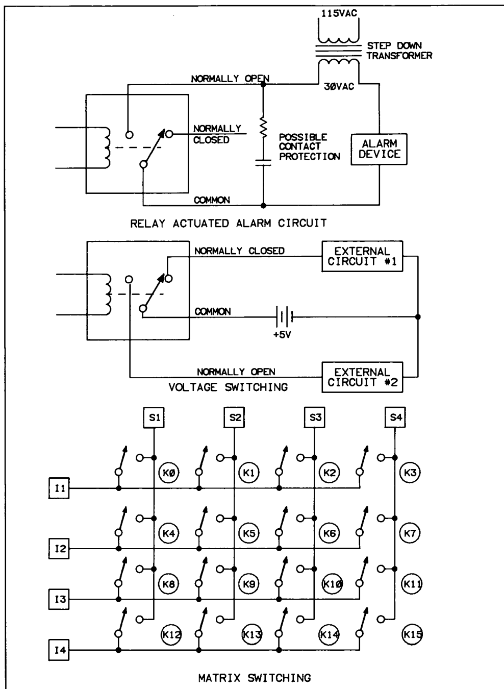
Figure 2-4. Voltage/Matrix Switching Examples
