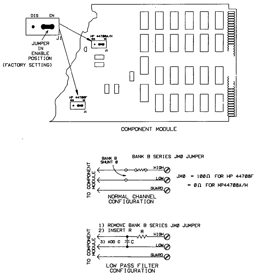
Figure 4-2. HP 44708 Isolation Jumper Configuration
