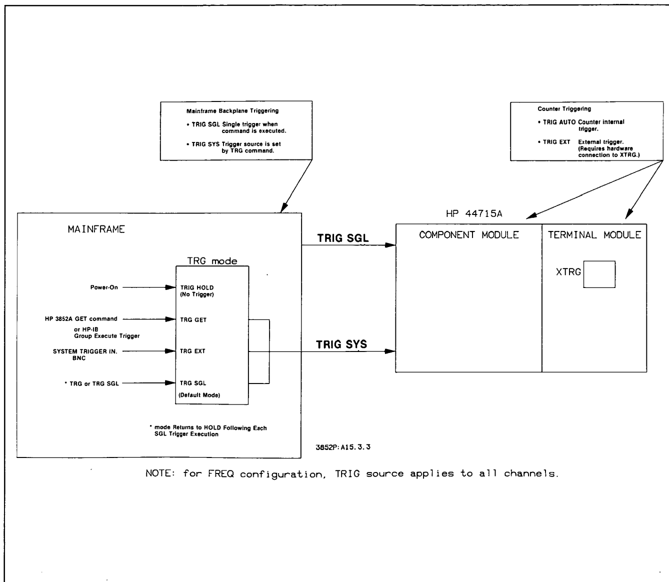
Figure 3-3. Counter Triggering Sources
