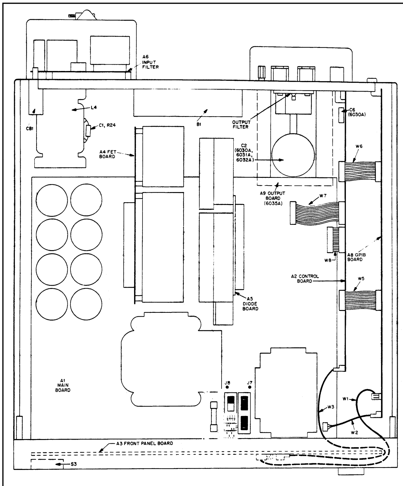
Figure 6-1. Top View, Top Covers Removed
