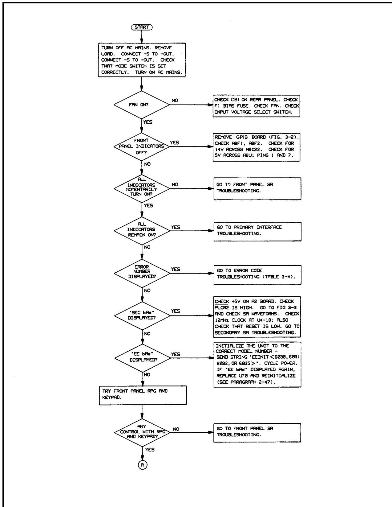
Figure 3-1. Troubleshooting Isolation
