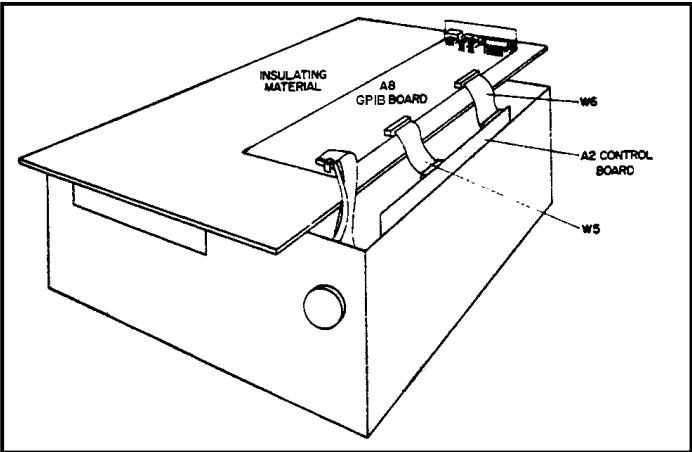
Figure 3-2. GPIB Board Test Setup
