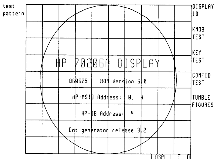
Figure 2-64. Display Tests Menu
