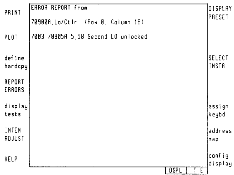
Figure 1-10. Report Errors
