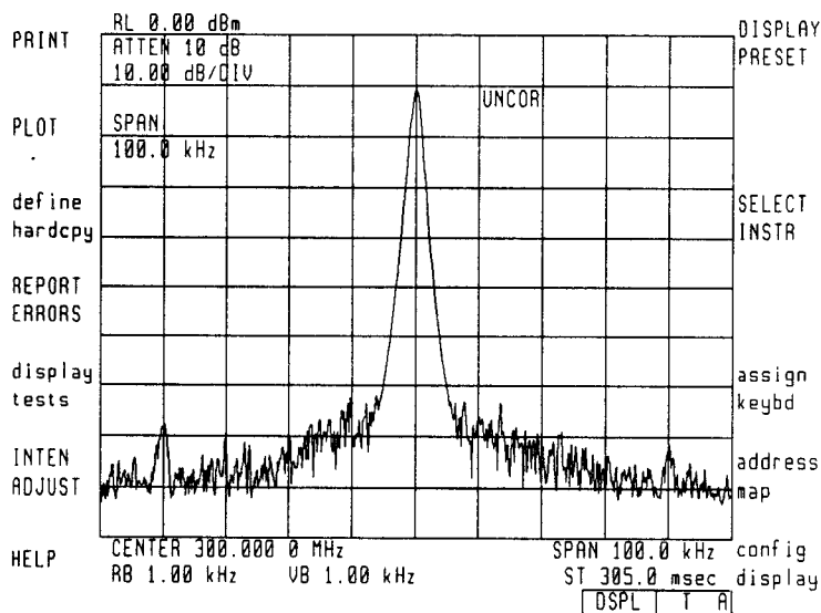
Figure 1-5. Display Capabilities
