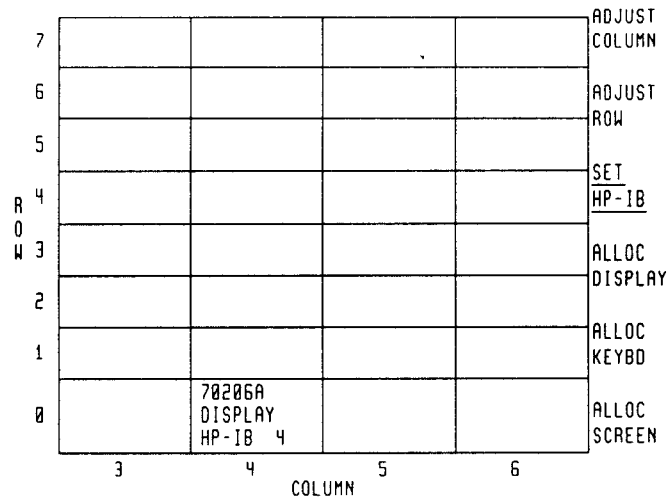
Figure 2-10. Adjust Column
