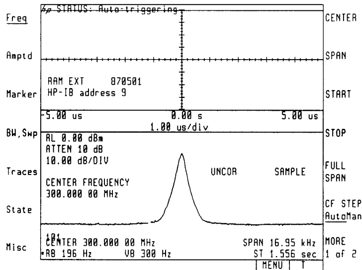
Figure 2-16. Configuring Display
