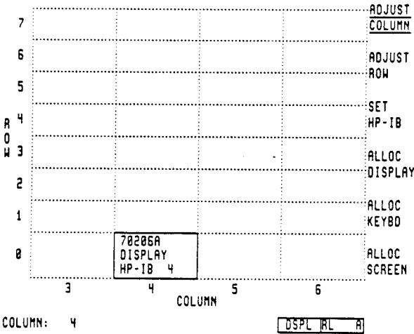
Fig 1. Address Map
