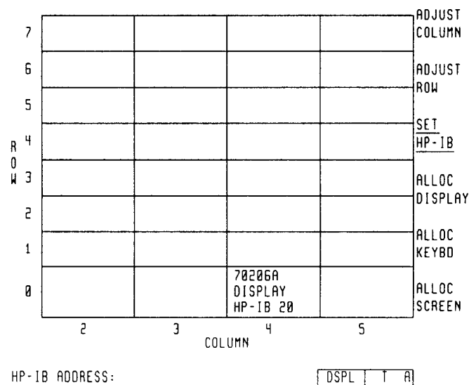
Figure 2-11. Setting HP-IB
