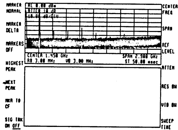
Fig. 3. Two-window screen.
