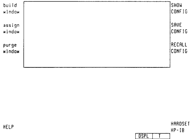
Figure 2-41. Save Configuration
