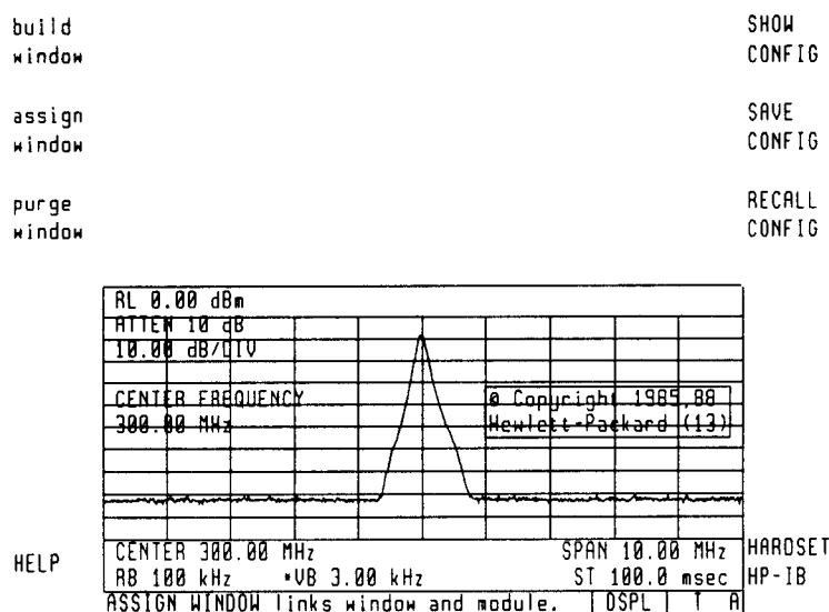
Figure 2-18. Build Window #2
