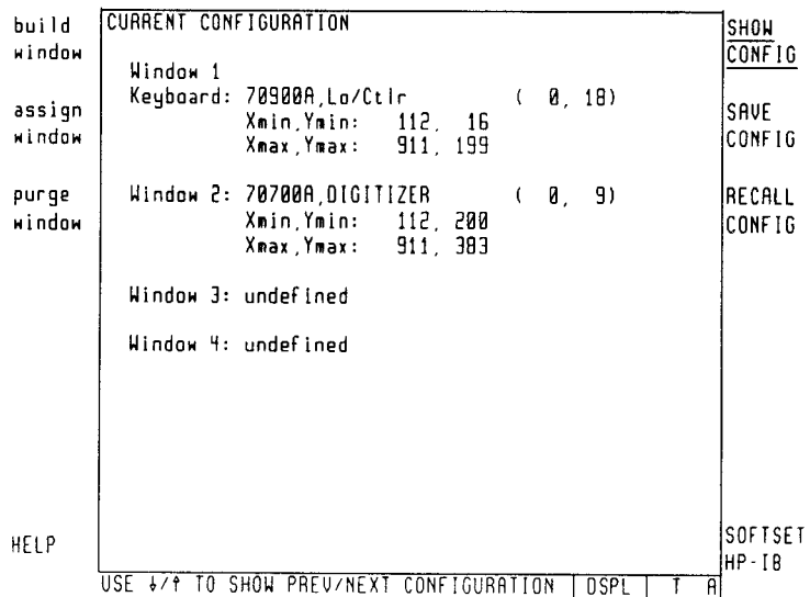
Figure 2-38. Current Configuration
