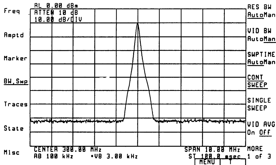
Figure 2-48. Wider Plot
