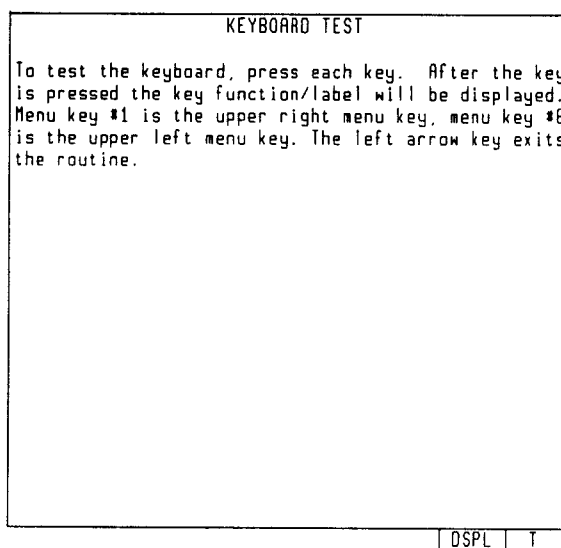
Figure 2-66. Key Test
