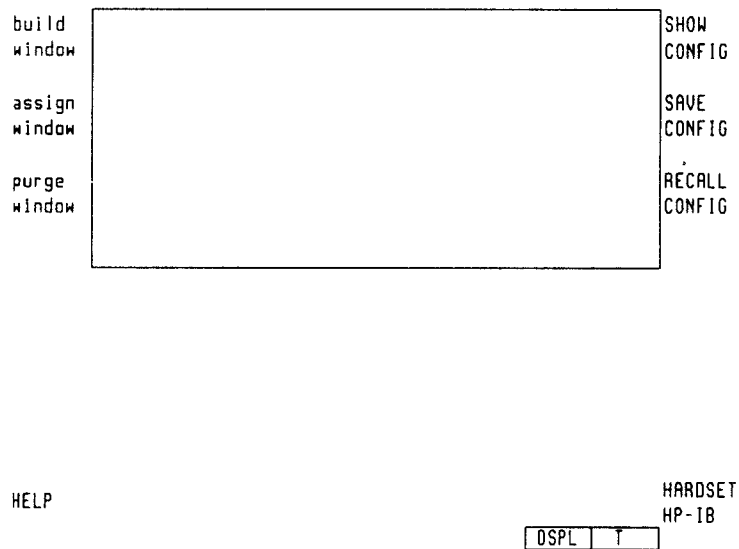
Figure 2-27. Select Window #1
