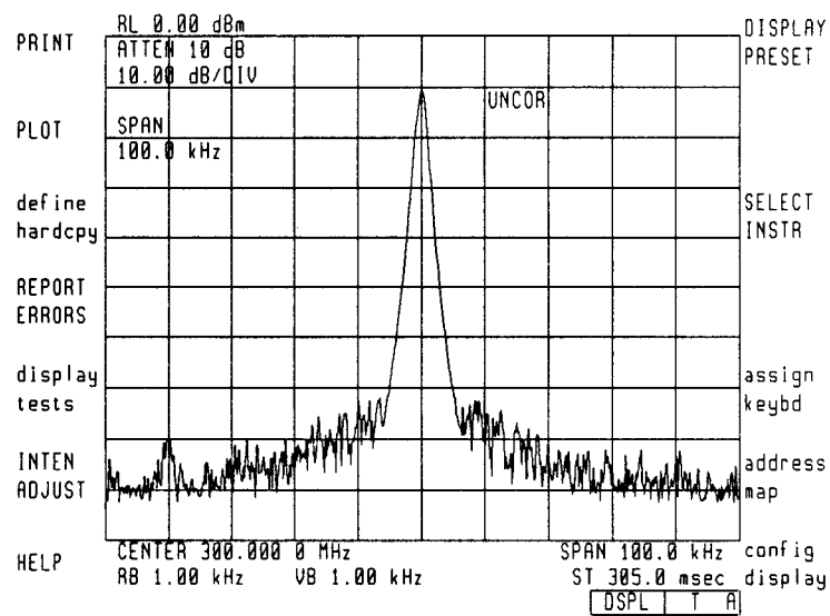
Figure 1-6. Select Instrument
