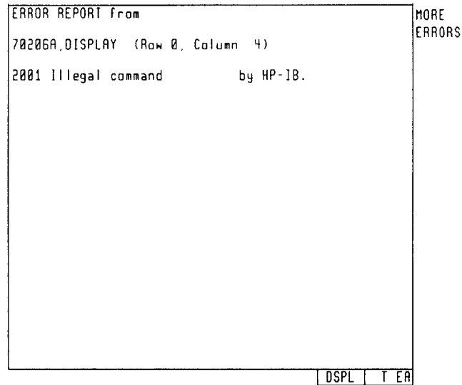
Figure 2-62. Multi-Instrument Errors
