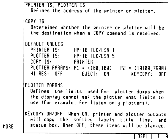
Figure 2-55. Help Screen, Page #1
