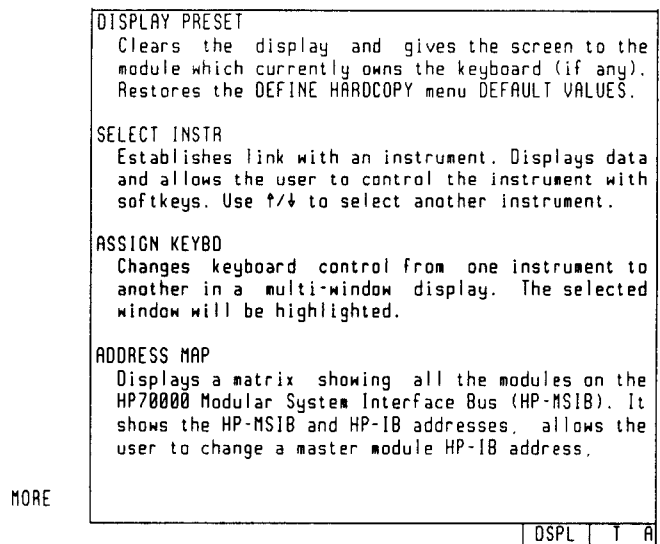
Figure 2-67. Display Help, Page #1
