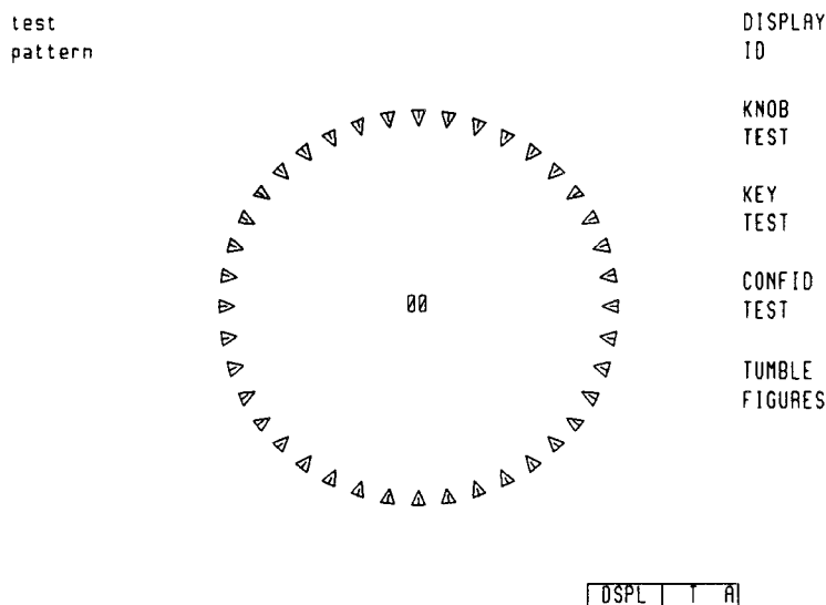
Figure 2-65. Knob Test
