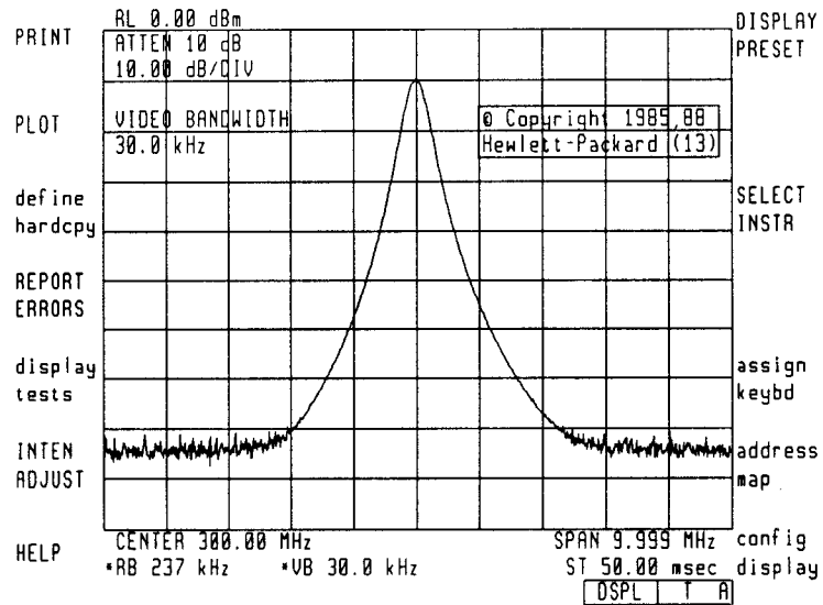
Figure 2-15. Allocated Display
