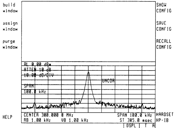
Figure 2-40. Recall Configuration
