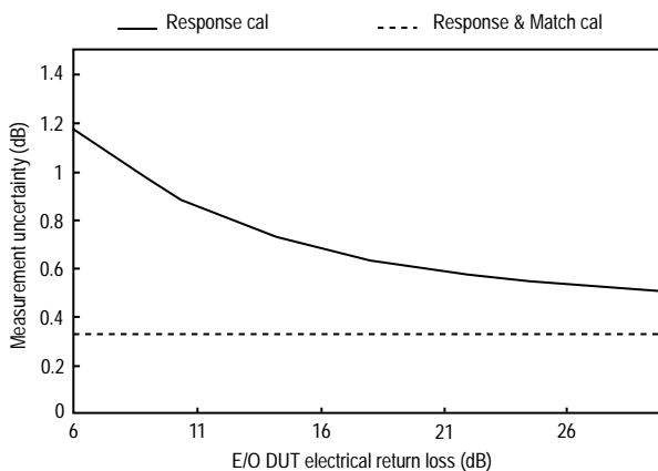
Measurement accuracy vs. E/O electrical return loss (characteristic)
