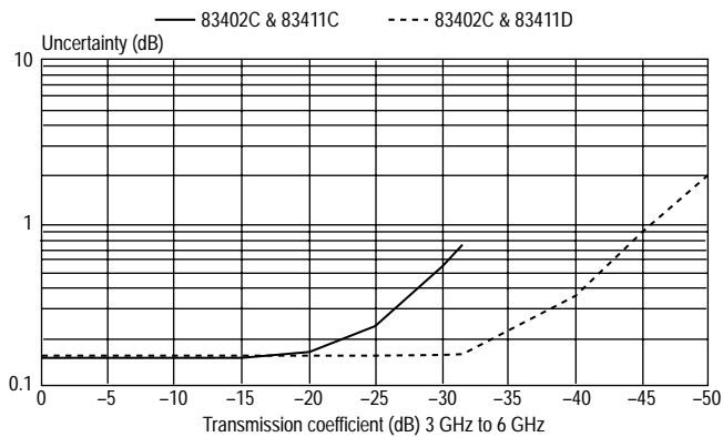
Relative transmission coefficient uncertainty 3 to 6 GHz (characteristic)
