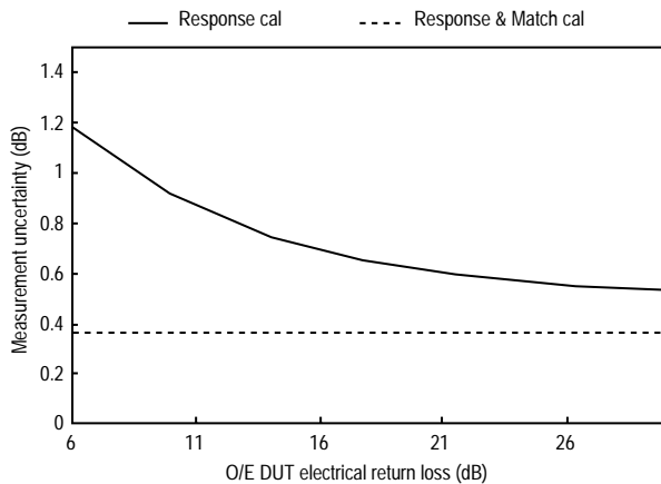
Measurement accuracy vs. O/E electrical return loss (characteristic)
