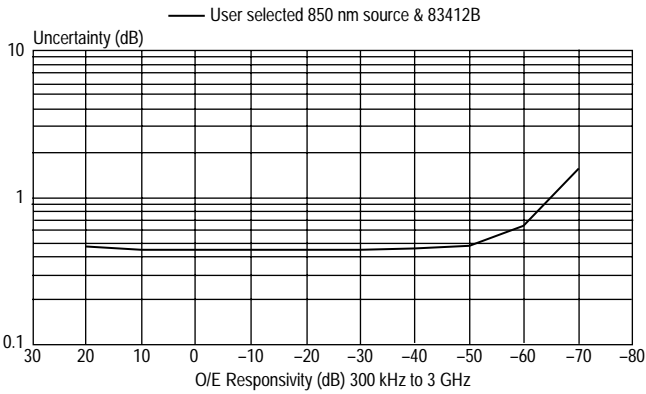
Responsivity flatness uncertainty 300 kHz to 3 GHz (characteristic)
