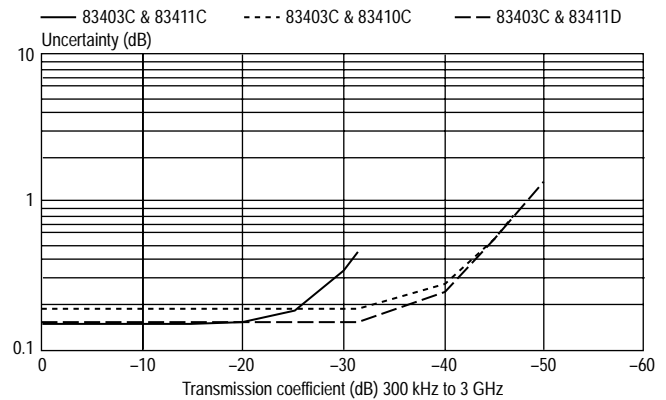
Relative transmission coefficient uncertainty 300 kHz to 3 GHz (characteristic)
