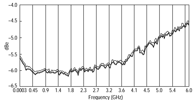
Agilent 8702E system repeatability of O/E measurement
