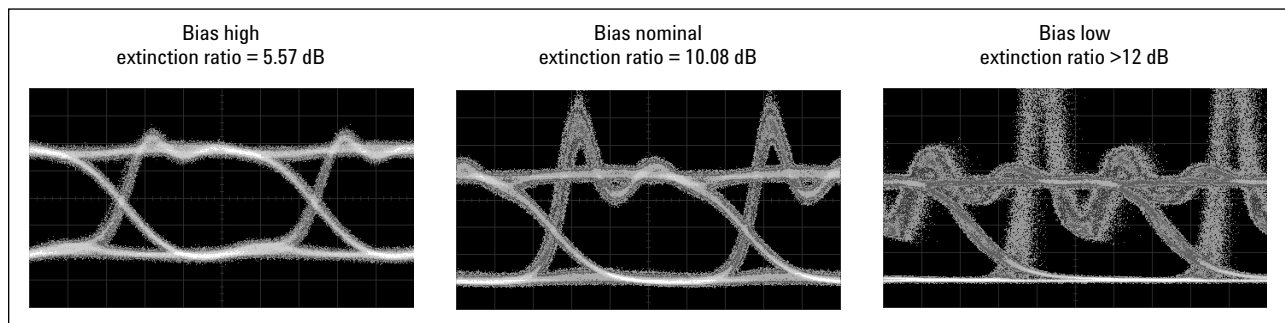
Figure 6. Agilent 83430A extinction ratio versus waveform fidelity at 2.48832 Gb/s
