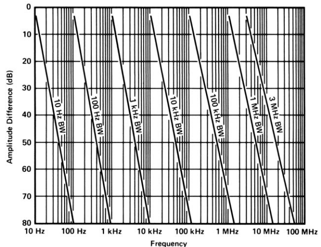
Figure 1. Typical spectrum analyzer resolution
