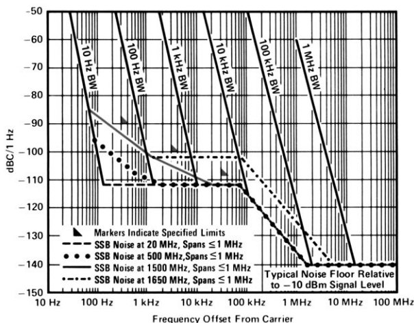
Figure 2. Typical SSB noise versus offset from carrier
