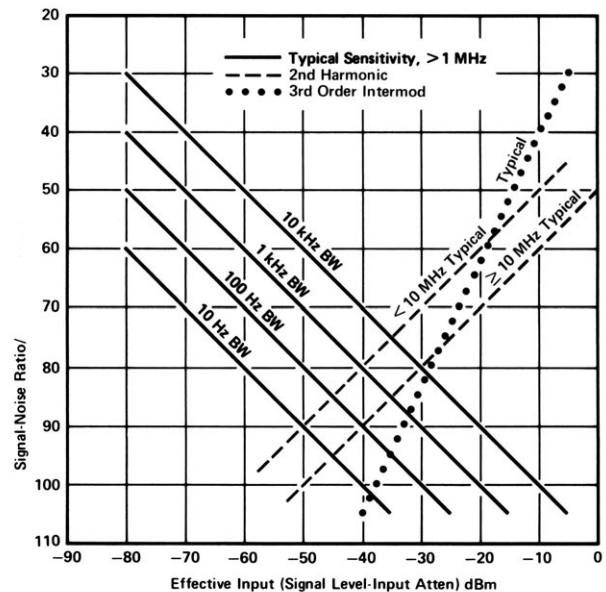
Figure 3. Optimum dynamic range
