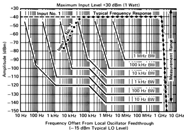
Figure 4. Typical sensitivity vs. input frequency
