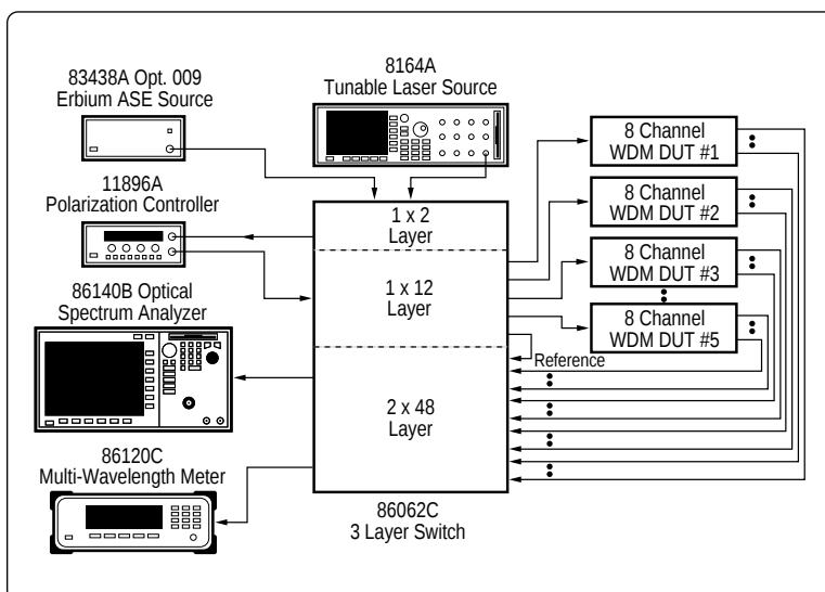
Figure 11. Eight channel WDM/router test setup
