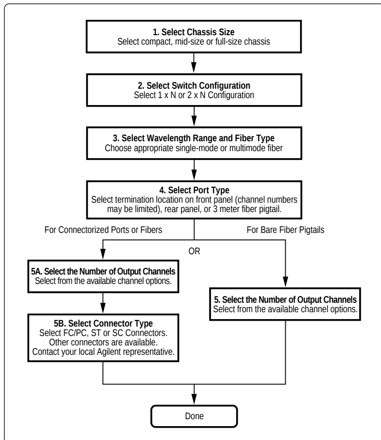
Figure 13. Configuration flowchart
