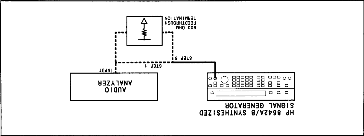
Figure 4-7. Internal Modulation Oscillator Test Setup
