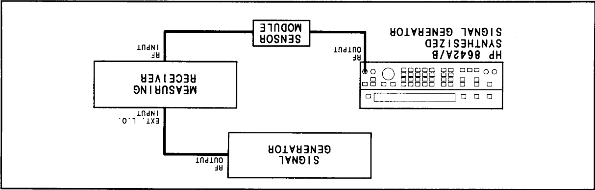
Figure 4-14. Residual Test Setup
