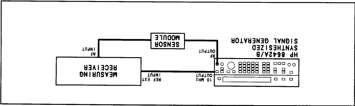
Figure 4-3. Pulse Test Setup
