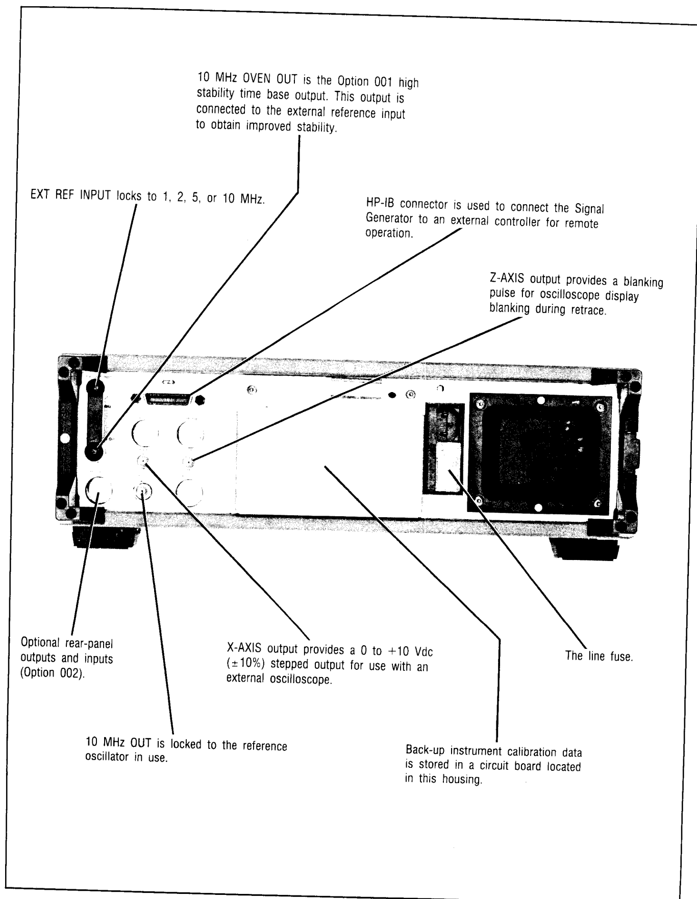
Figure 3-2. Rear-Panel Features
