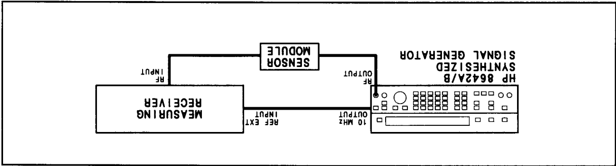
Figure 4-2. Harmonics Test Setup
