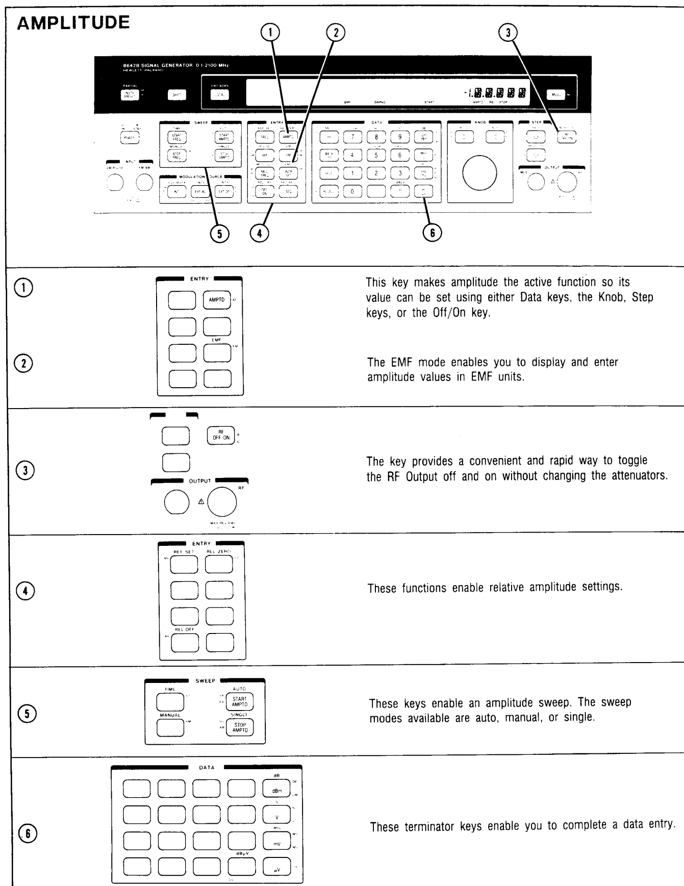
Figure 3-8. Amplitude-Related Functions
