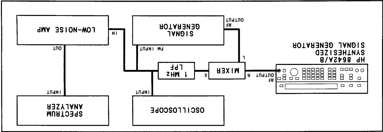
Figure 4-12. SSB Phase Noise Test Setup (Optional)
