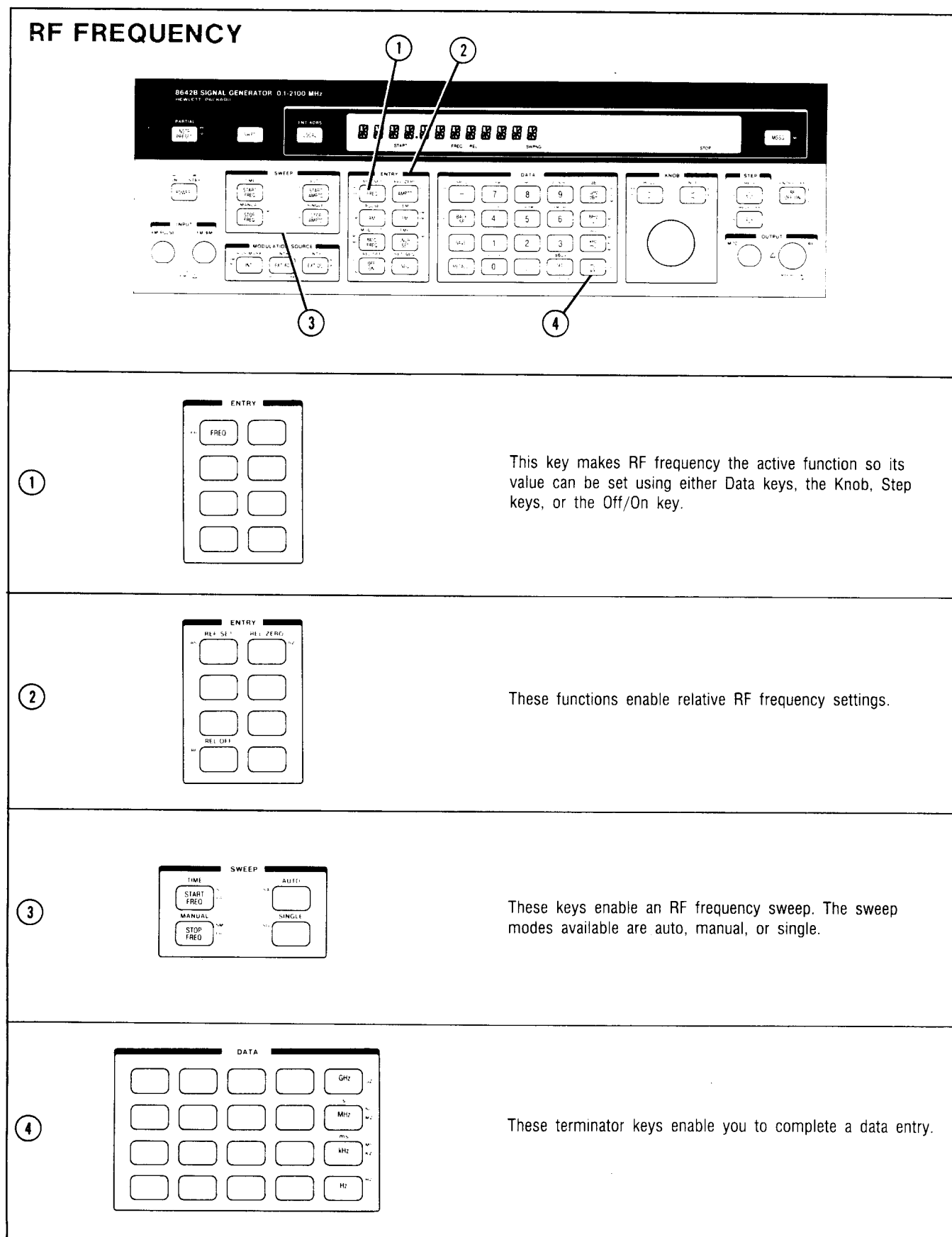
Figure 3-6. RF Frequency-Related Functions
