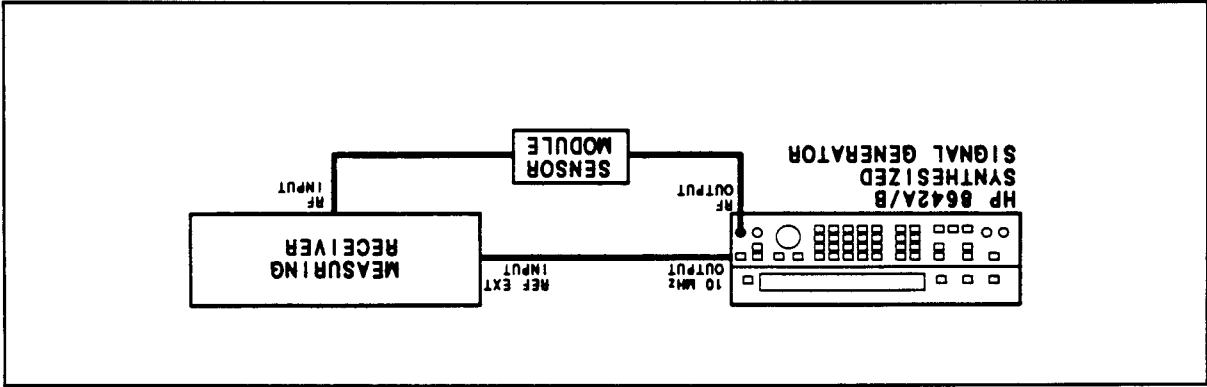
Figure 4-5. AM, FM, and PM Test Setup
