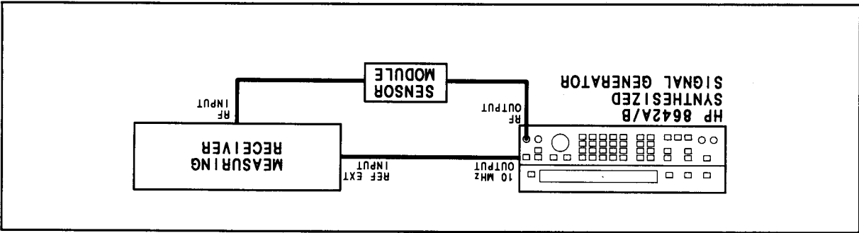
Figure 4-1. Level Accuracy and Flatness Test Setup
