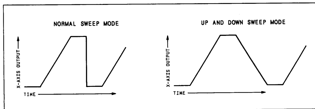
Figure 3-10. Sweep Waveforms
