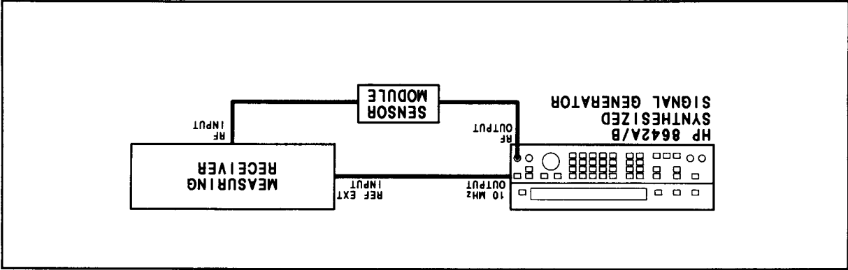
Figure 4-4. Residuals Test Setup
