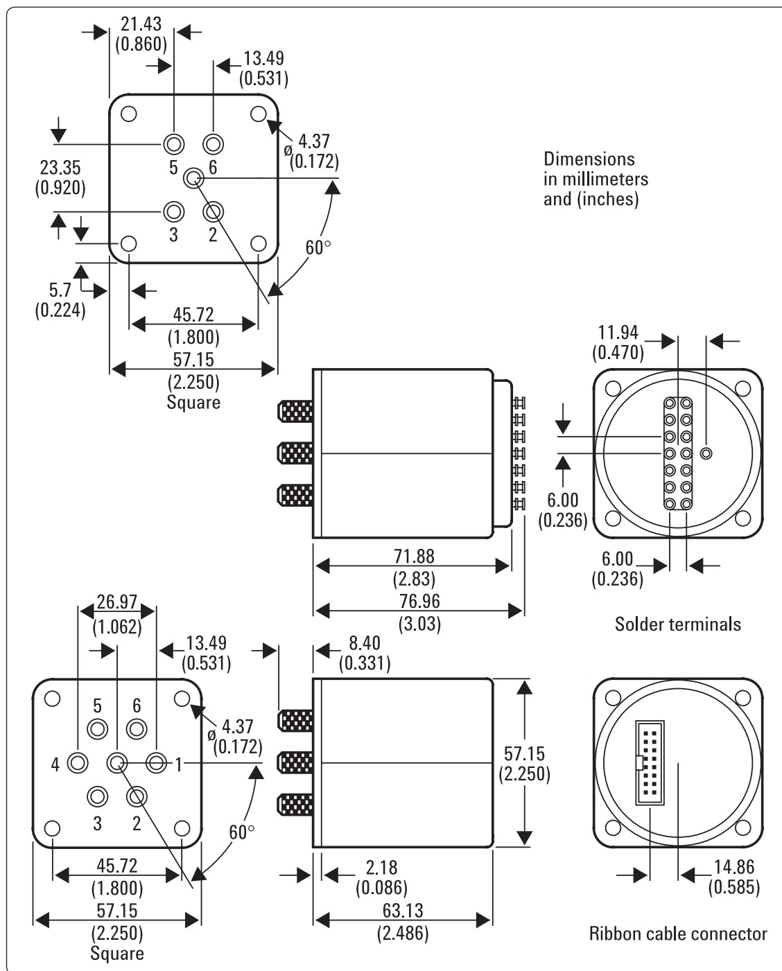
Figure 9. Product outlines
