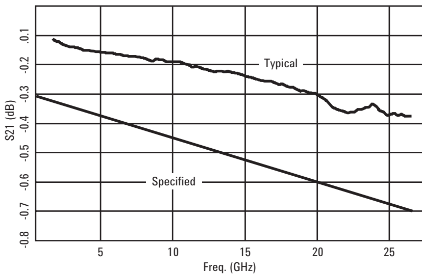
Figure 7. Insertion loss
