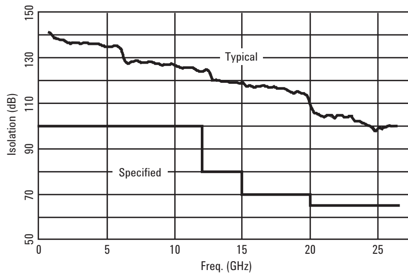
Figure 8. Isolation
