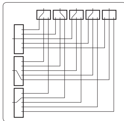
Figure 5. Full access matrix
