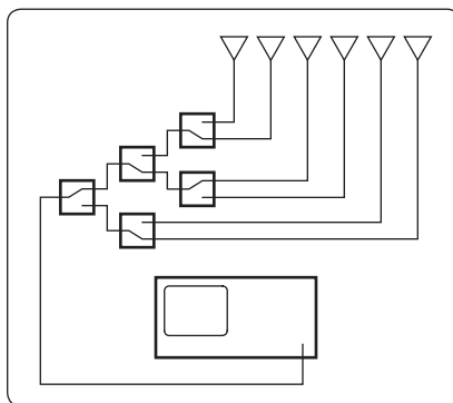
Figure 2. Tree matrix
