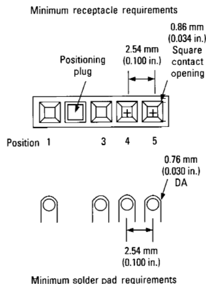
Figure 1b. Suggested receptacle dimensions
