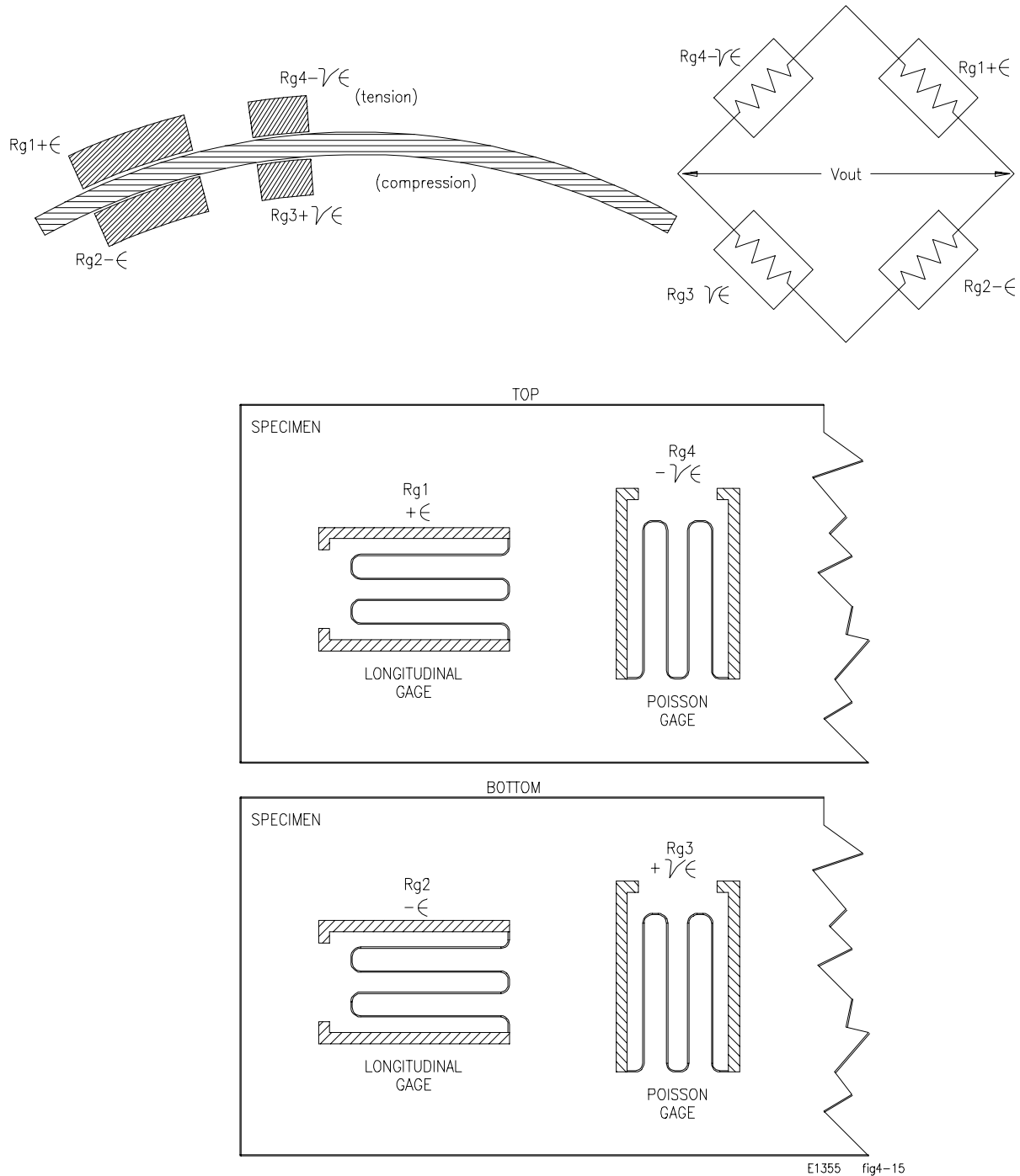
Figure 4-15. Bending Poisson Arrangement
