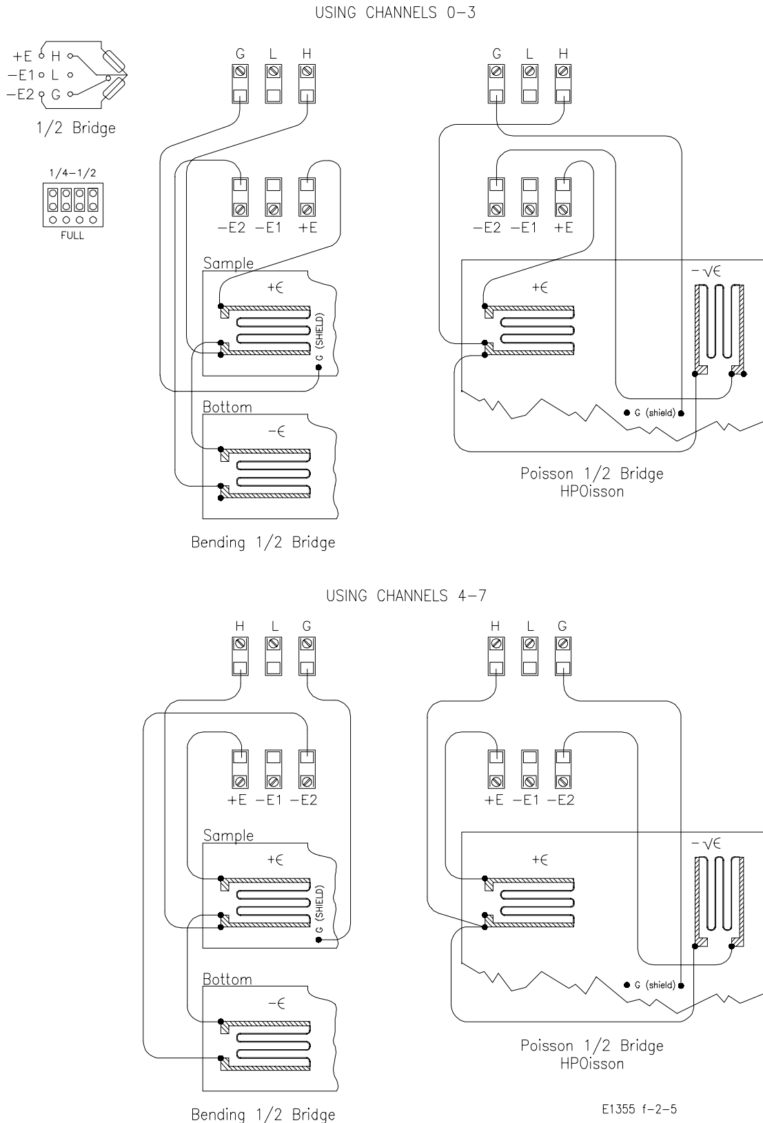
Figure 2-5. Connecting Strain Gages in 1/2 Bridge Arrangements
