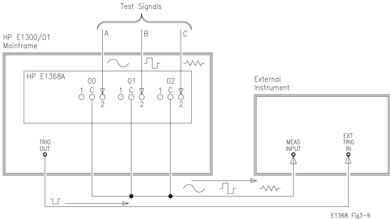
Figure 3-9. Example: Multiple Channel Scanning
