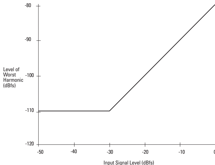
Figure 3: Harmonic distortion as a function of input level.
