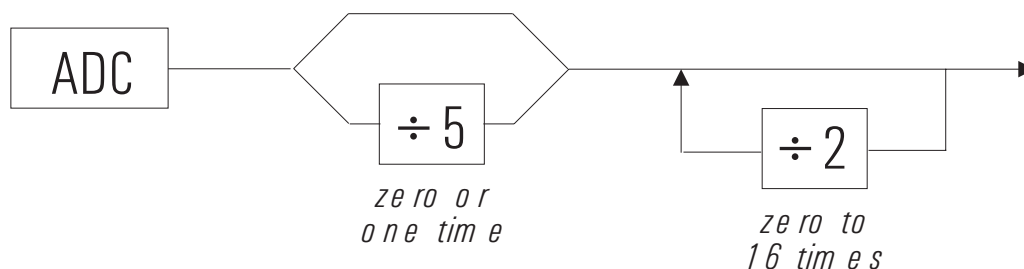
Figure 3-6: Decimation filter diagram - baseband
