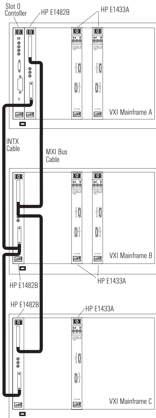
Figure 4-2: Multiple mainframes - three mainframes
