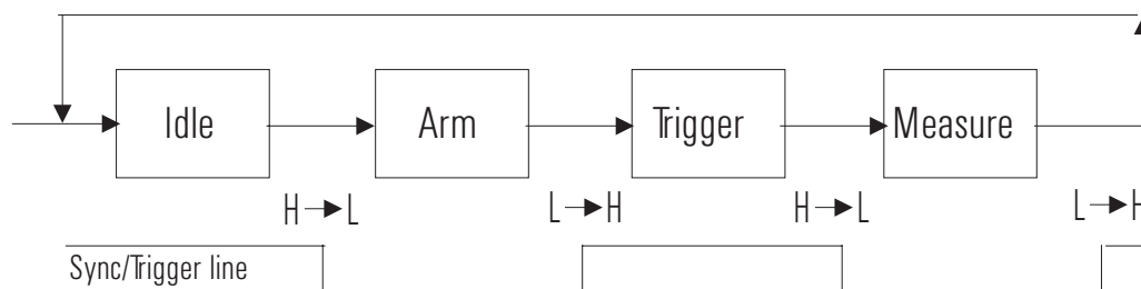
Figure 4-5: Measurement loop
