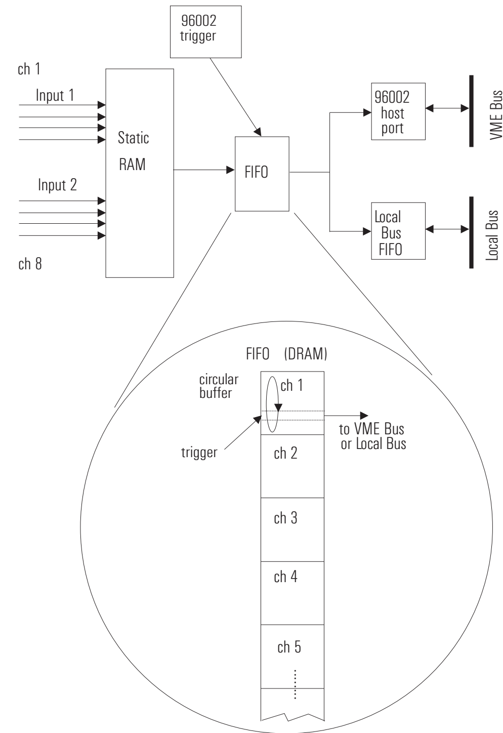
Figure 3-5: Data flow and FIFO architecture
