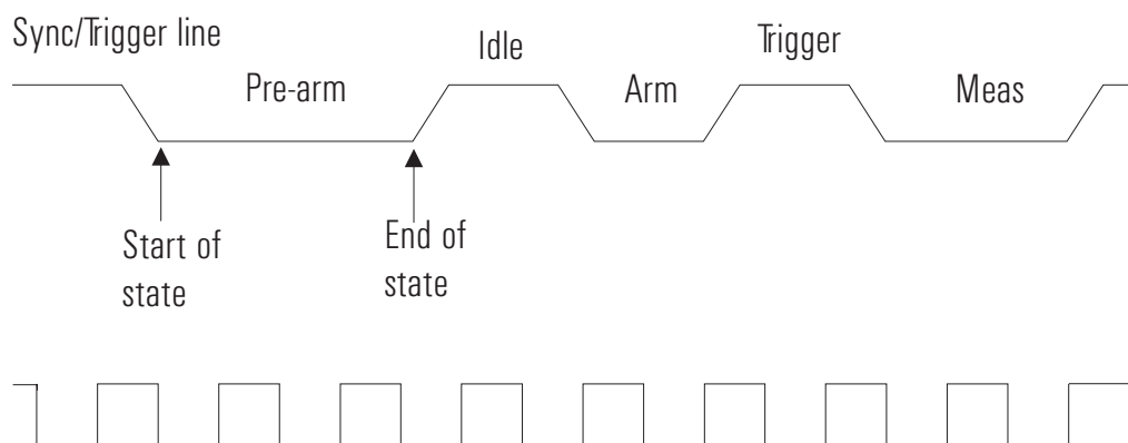
Figure 3-7: Transitions between states
