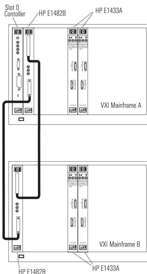
Figure 4-1: Multiple mainframes - two mainframes
