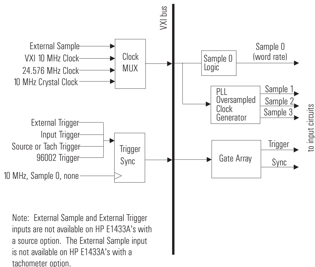
Figure 5-10: Clock/sync diagram
