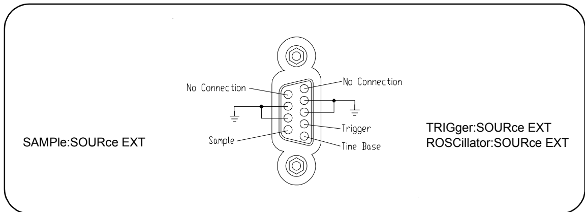
Figure 1-6. E1563A External Trigger Input Port
