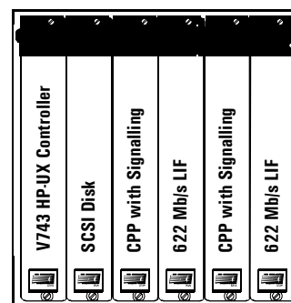
Figure 7: Typical configuration for dual port signalling testing over OC-12c/STM-4c.
